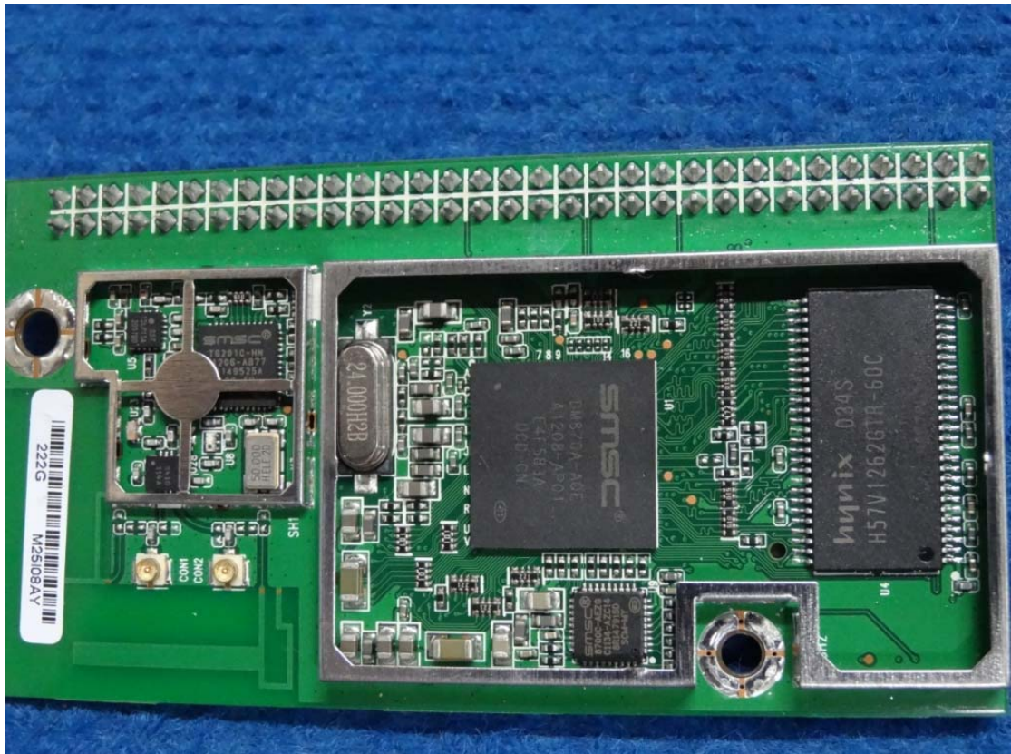
2.4GHz WIFI AIRPLAY module:
