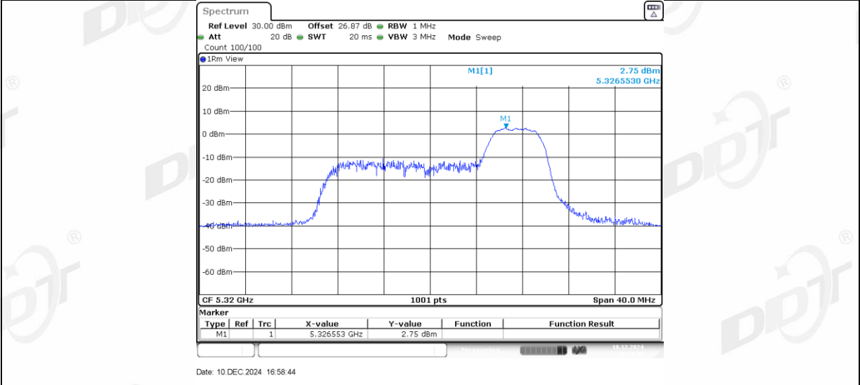
11AX20MIMO Ant2 5320_106Tone RU53
