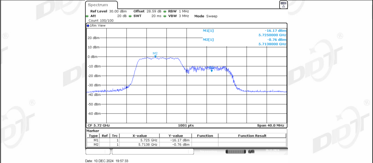
11AX20MIMO Ant1 5720 UNII-2C 106Tone_RU54
