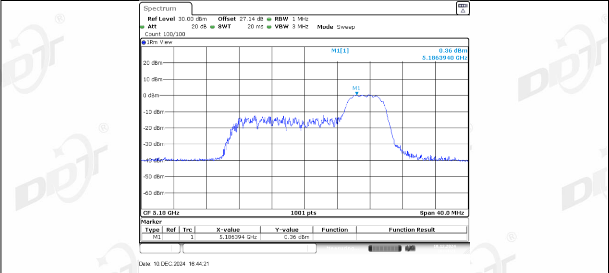
11AX20MIMO Ant1 5180_106Tone RU53
