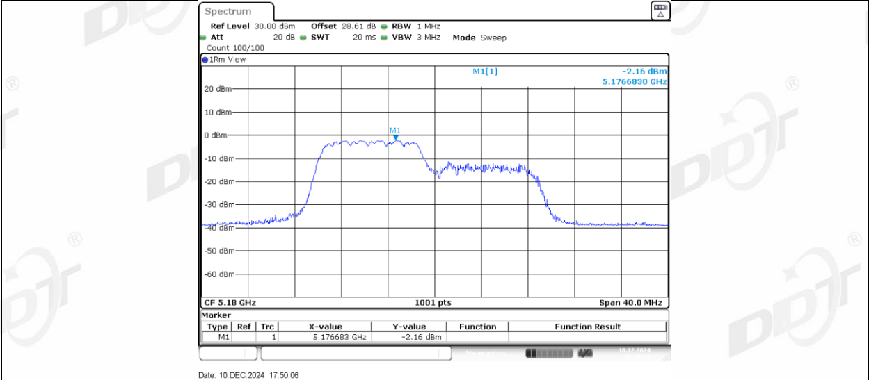
11AX20MIMO Ant1 5180_106Tone RU54
