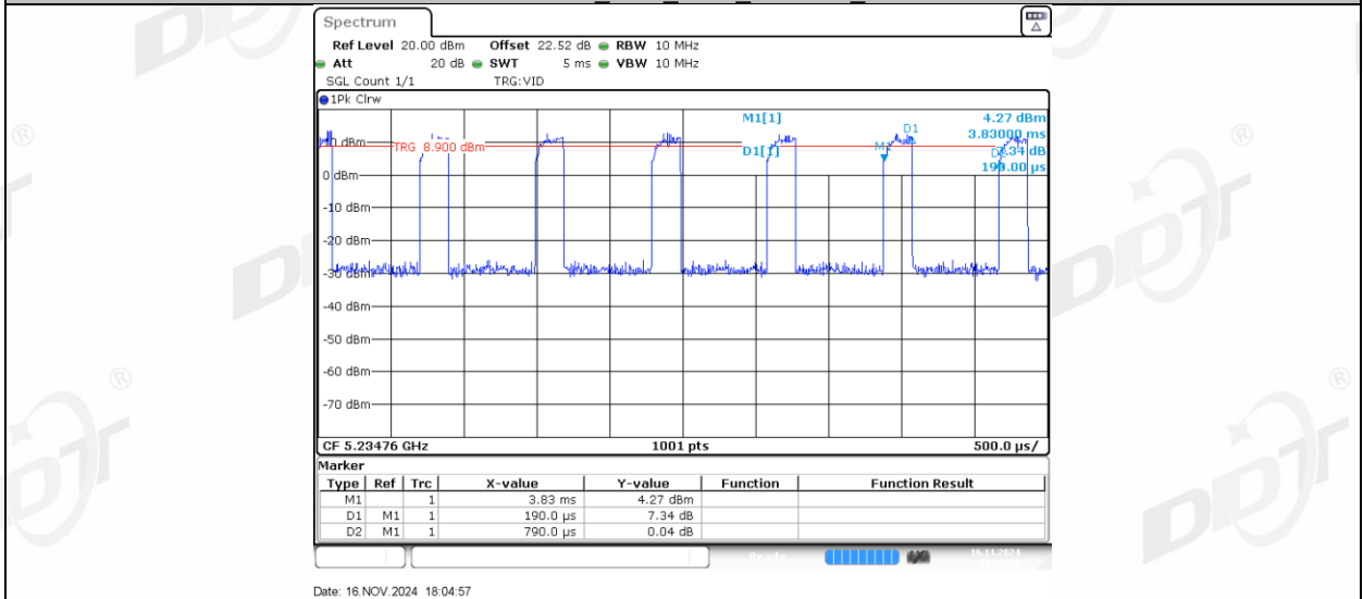
11AX20MIMO Ant1 5240_106Tone RU54
