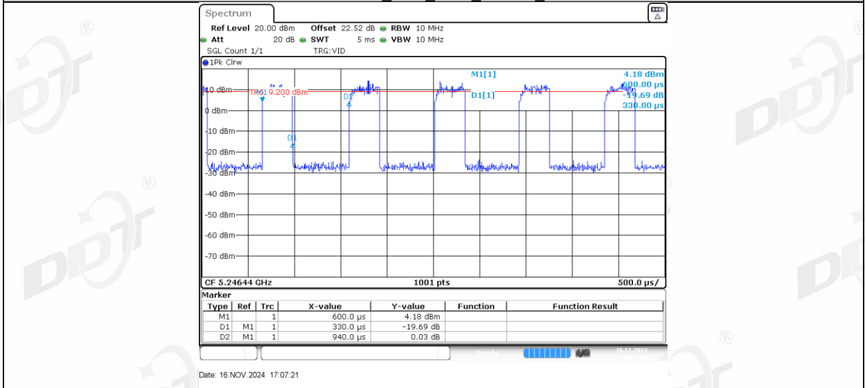
11AX20MIMO Ant1 5240_106Tone RU53
