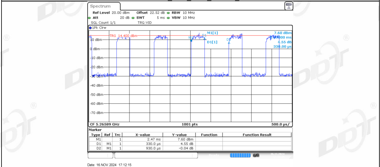
11AX20MIMO Ant1 5260 106Tone RU53
