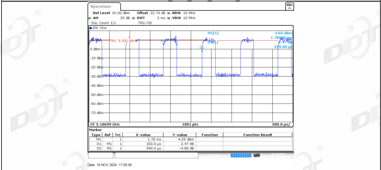
11AX20MIMO Ant2 5180_106Tone RU53
