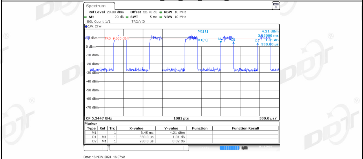
11AX20MIMO Ant2 5240 52Tone RU40
