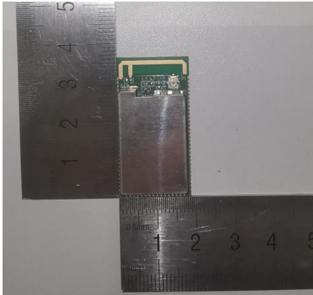
Figure 1. External view 1
