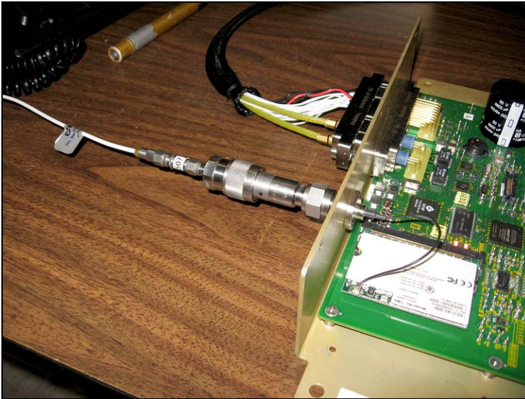
RADIATED SPURIOUS EMISSIONS - L-BAND ANTENNA
