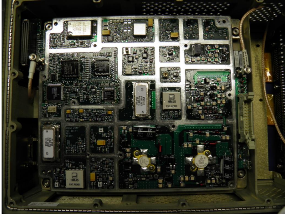
RF – Side B
