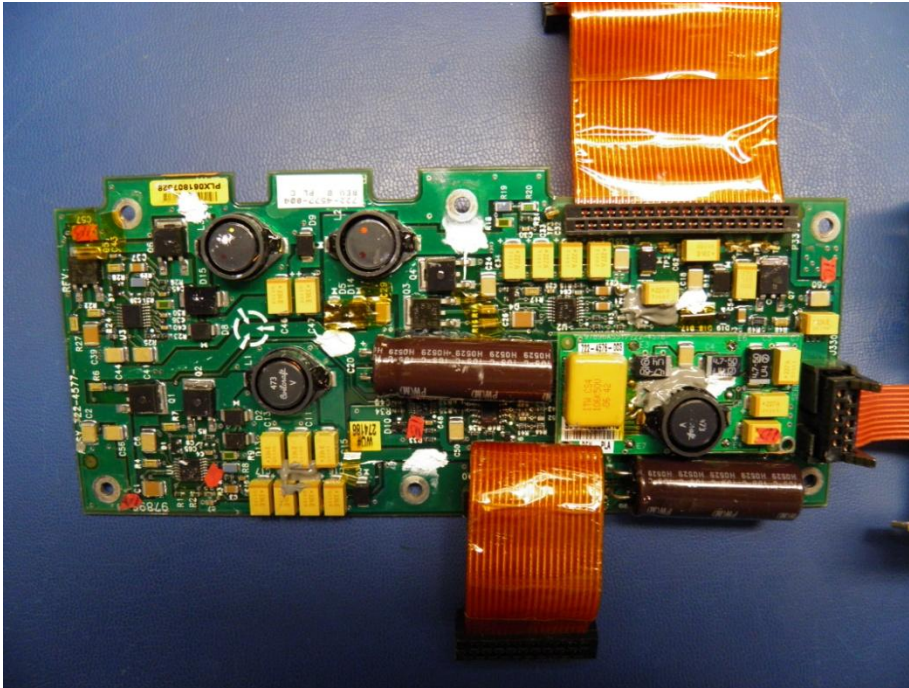
Power Supply Output – Side B
