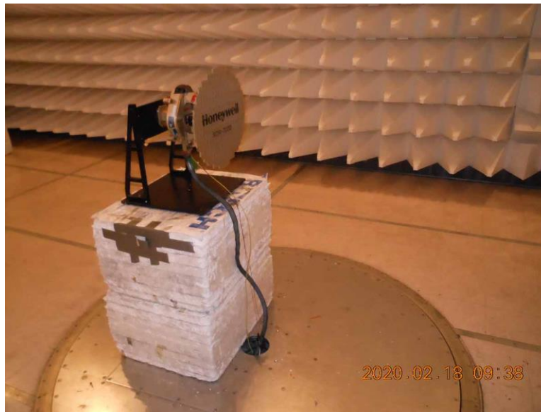
Radiated Emissions 18inch View #1
