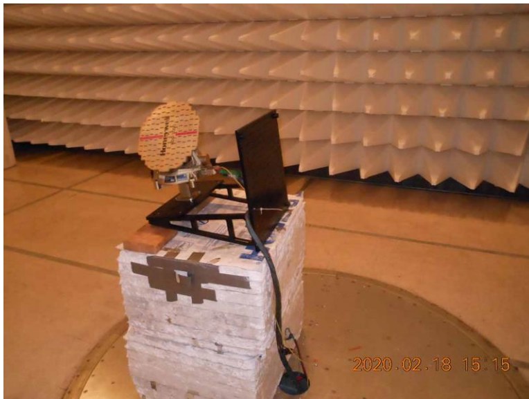
Radiated Emissions 12inch View #2
