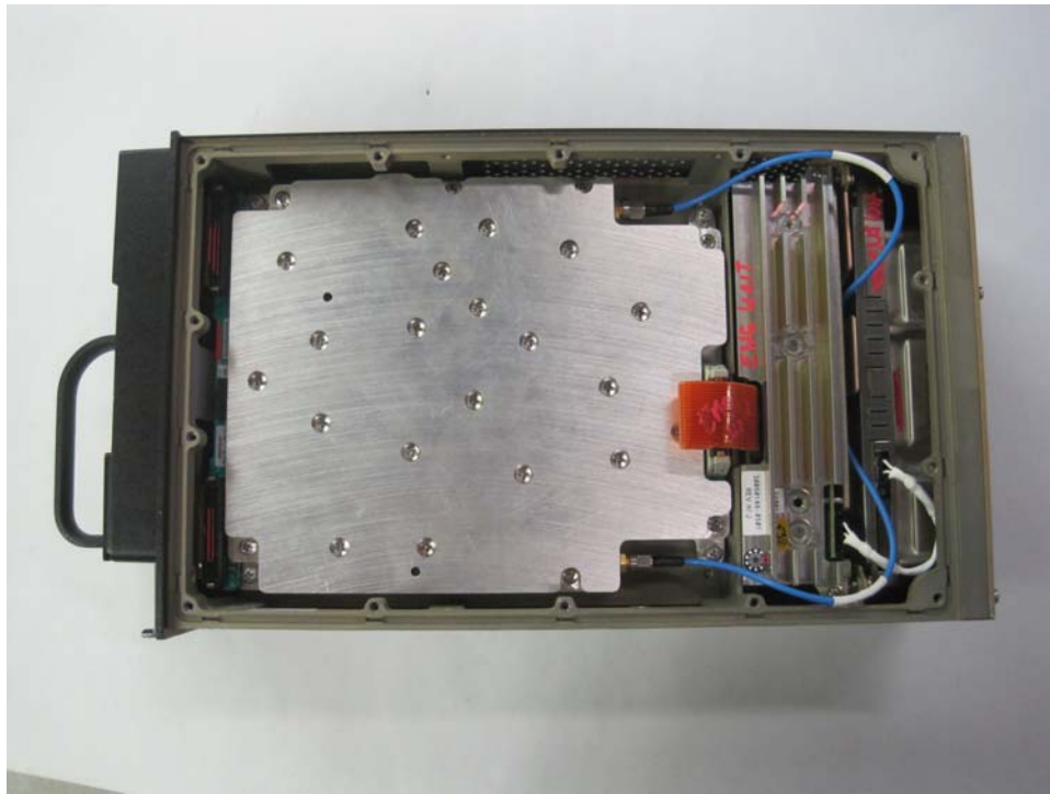
Side Cover Removed RF Board in Shield
