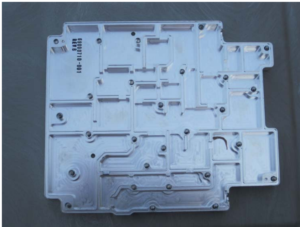
Shield Heatsink 2 with RF Board Removed
