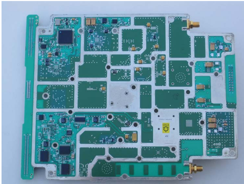
RF Board, Side 1
