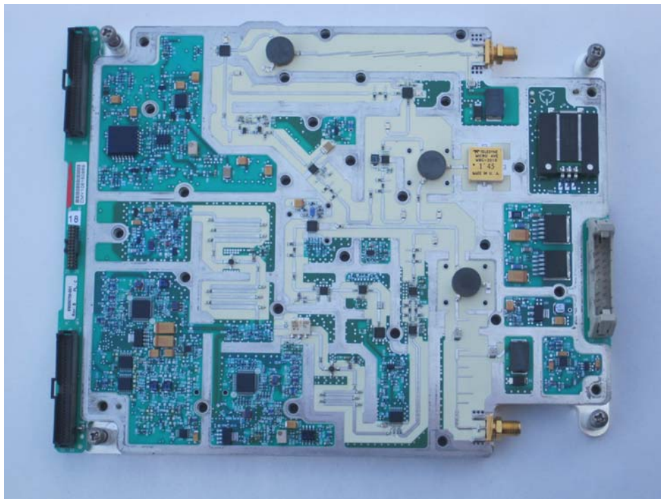
RF Board, Side 2
