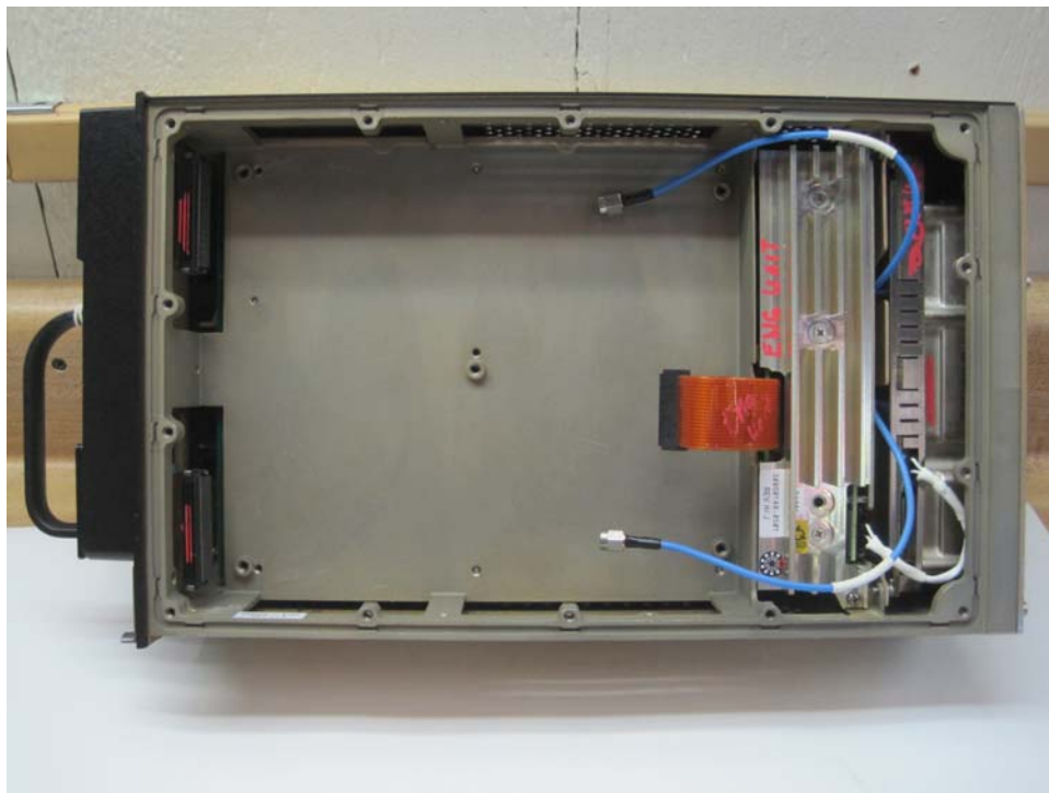
Side Cover Removed RF Board Removed
