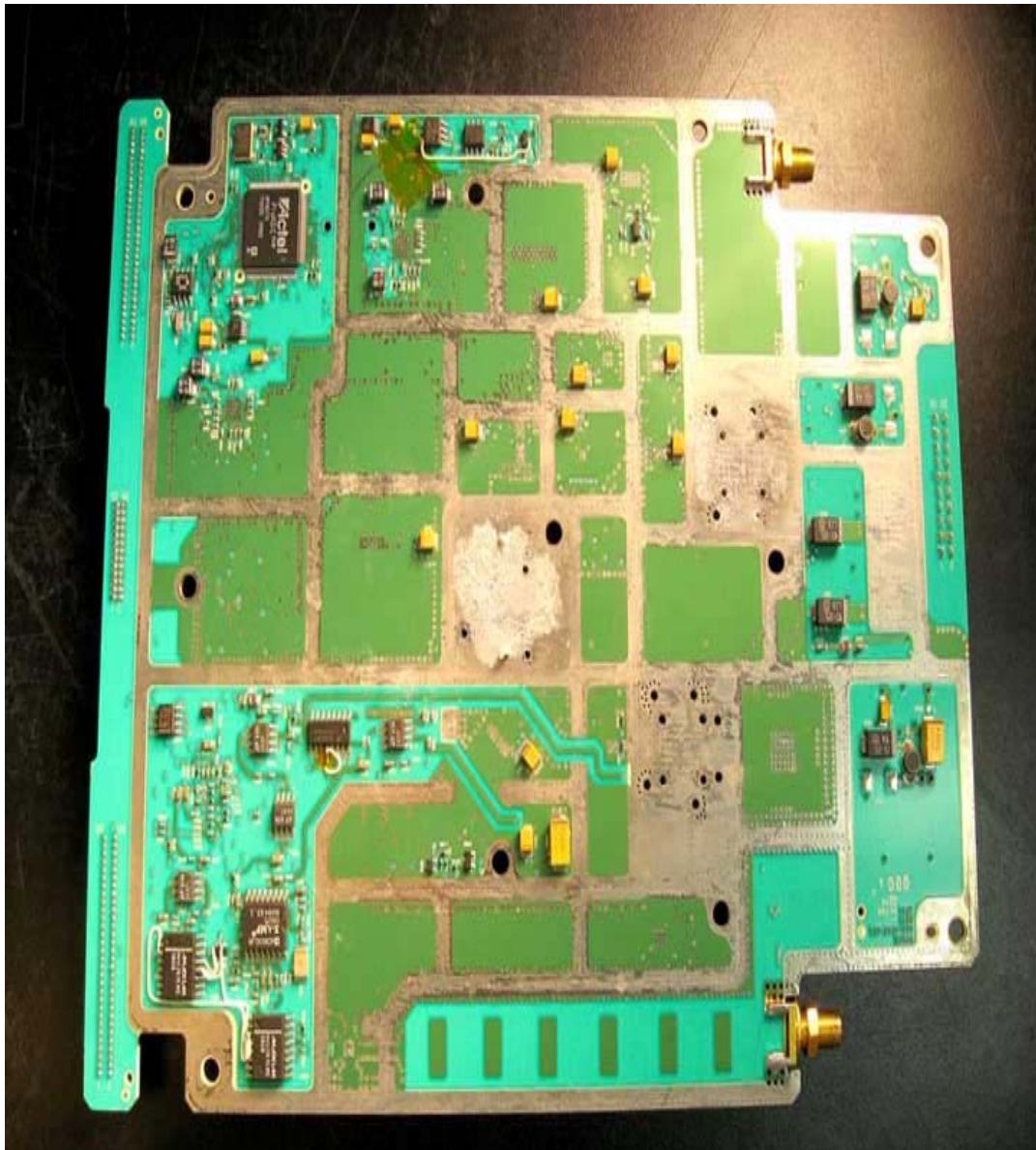
Submittal - RF board bottom side
