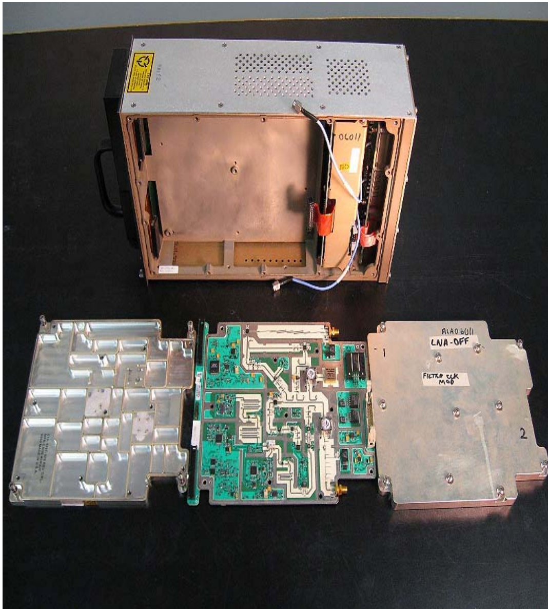
Submittal - RF board shields removed
