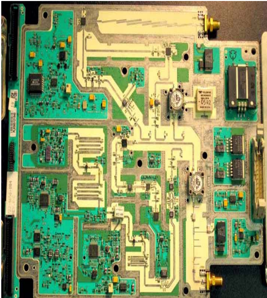
Submittal - RF board top side
