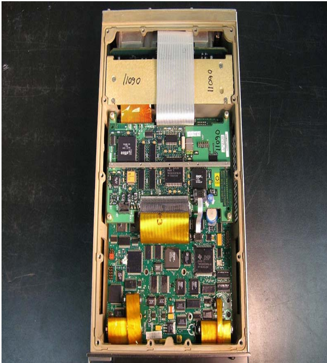
Submittal - Covers removed (control board side)
