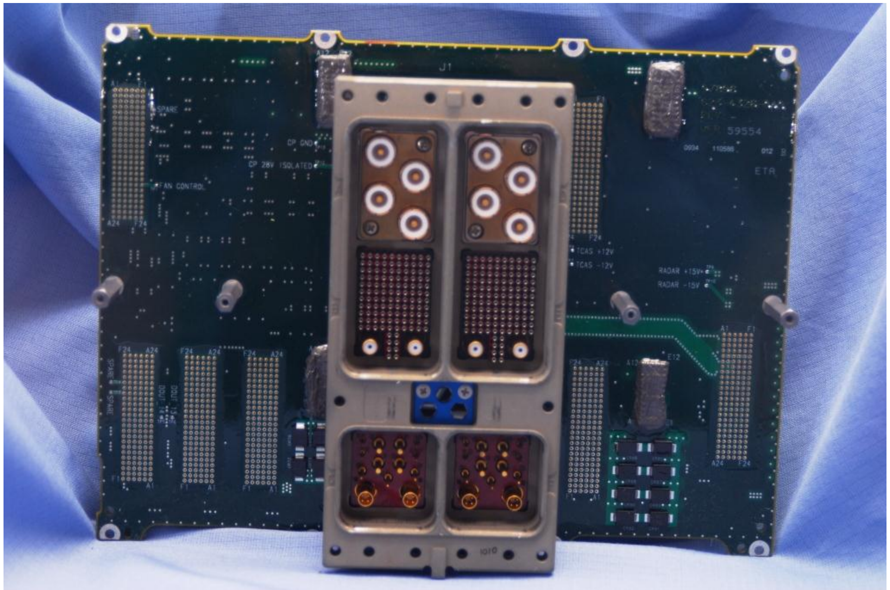
722-4484-040 (1) CCA / PWB, REAR INTERCONNECT
