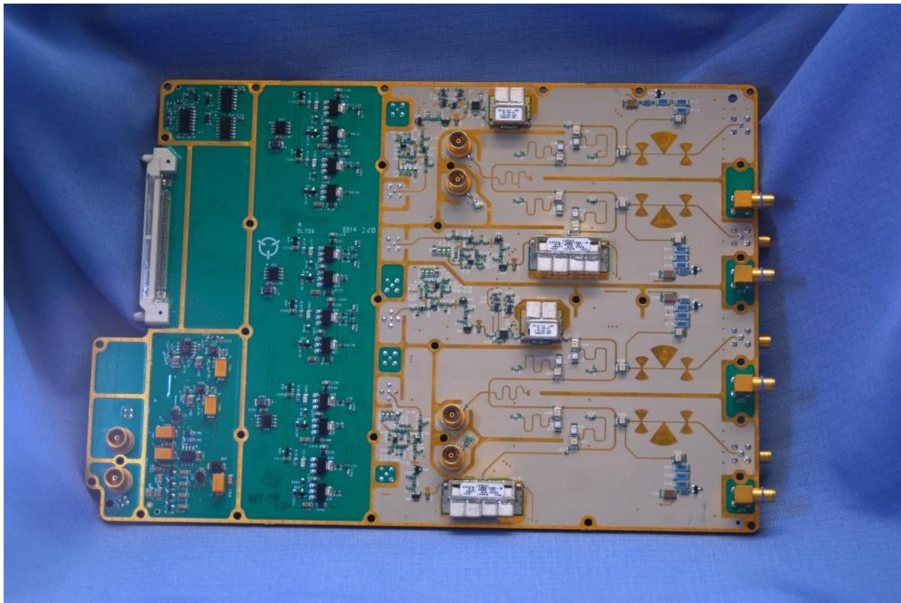
722-4490-007 (2) CCA / PWB, FRONT END, AESU
