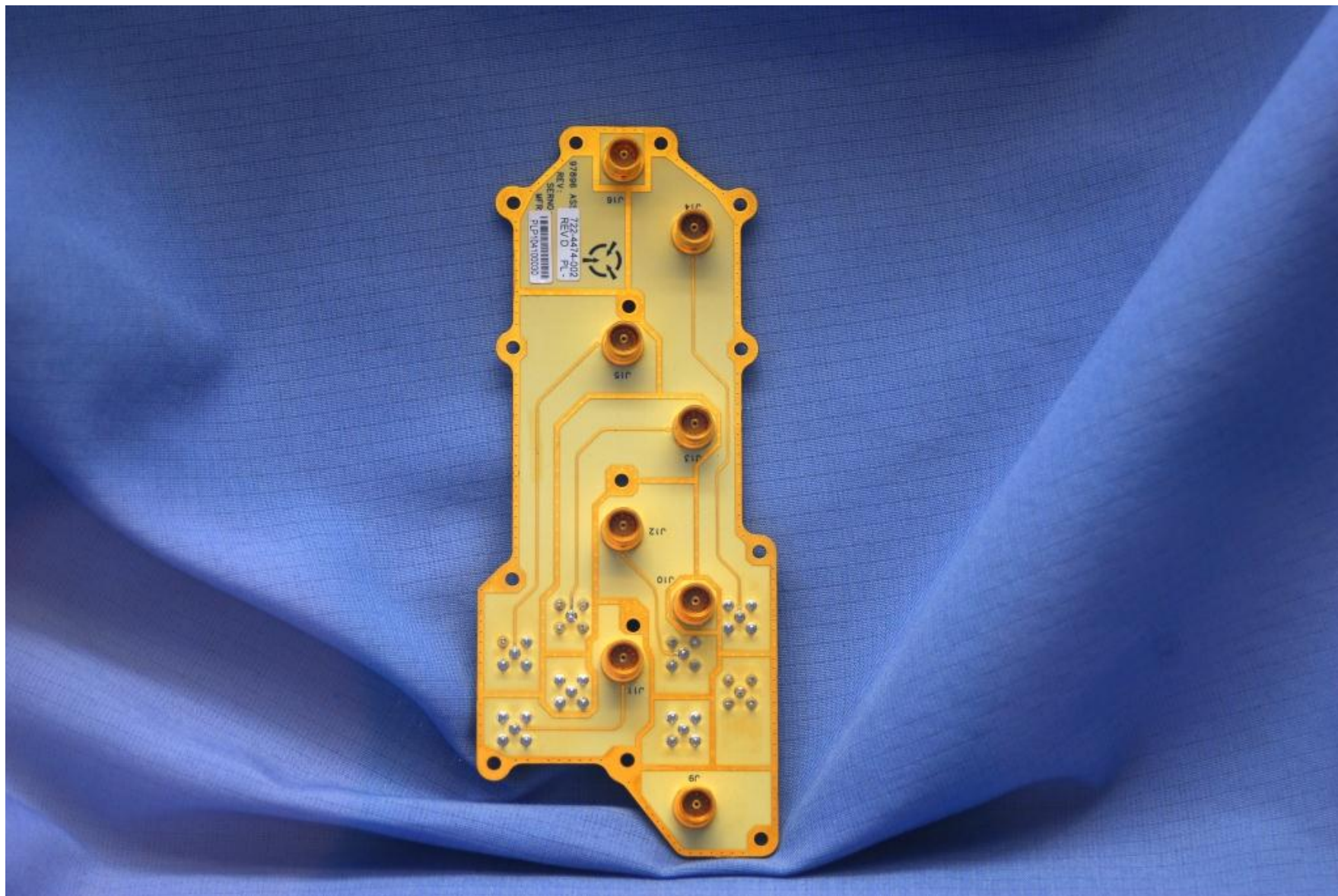
722-4474-002 (2) CCA / PWB, RF INTERCONNECT, AESU
