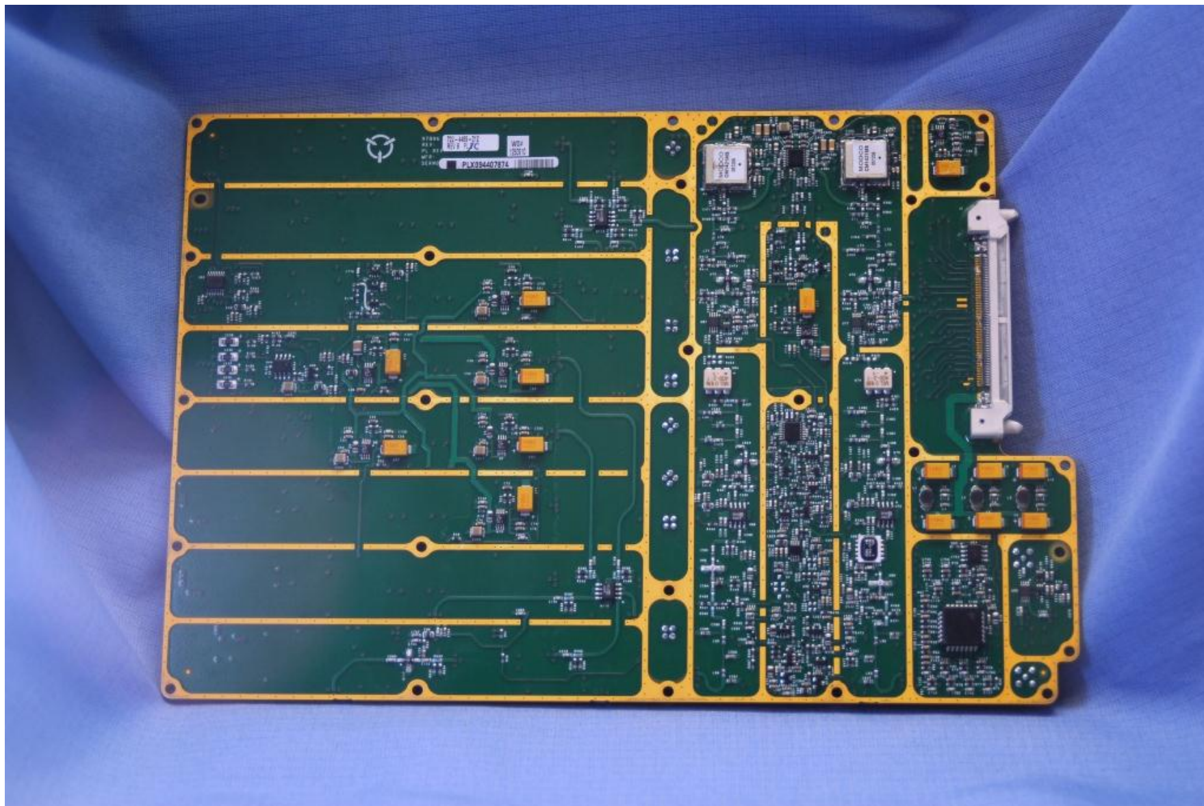
722-4489-012 (2) CCA / PWB, RF SYNTHESIZER-IF, AESU
