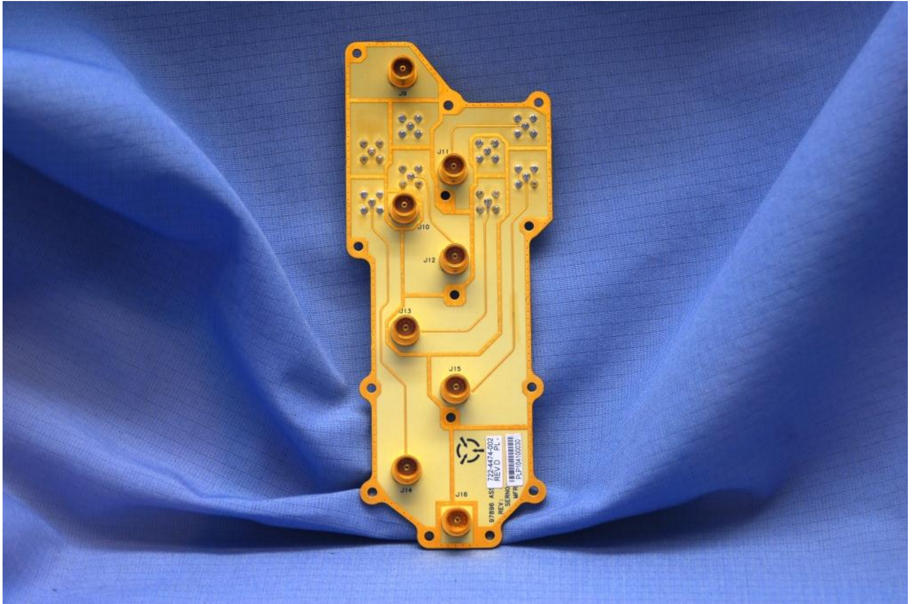
722-4474-002 (1) CCA / PWB, RF INTERCONNECT, AESU
