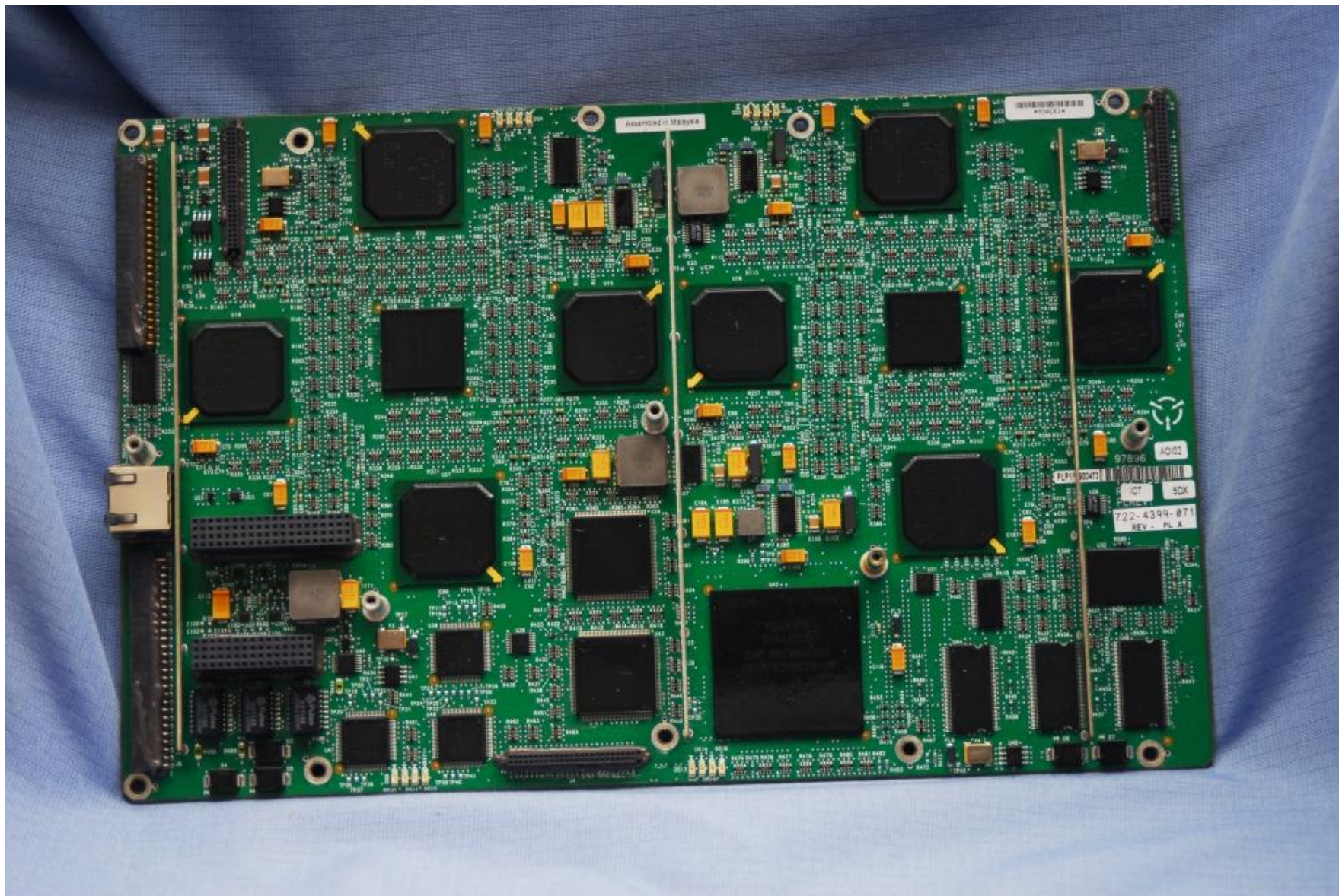
722-4399-024 (1) CCA / PWB, WX RADAR DSP, RP-1
