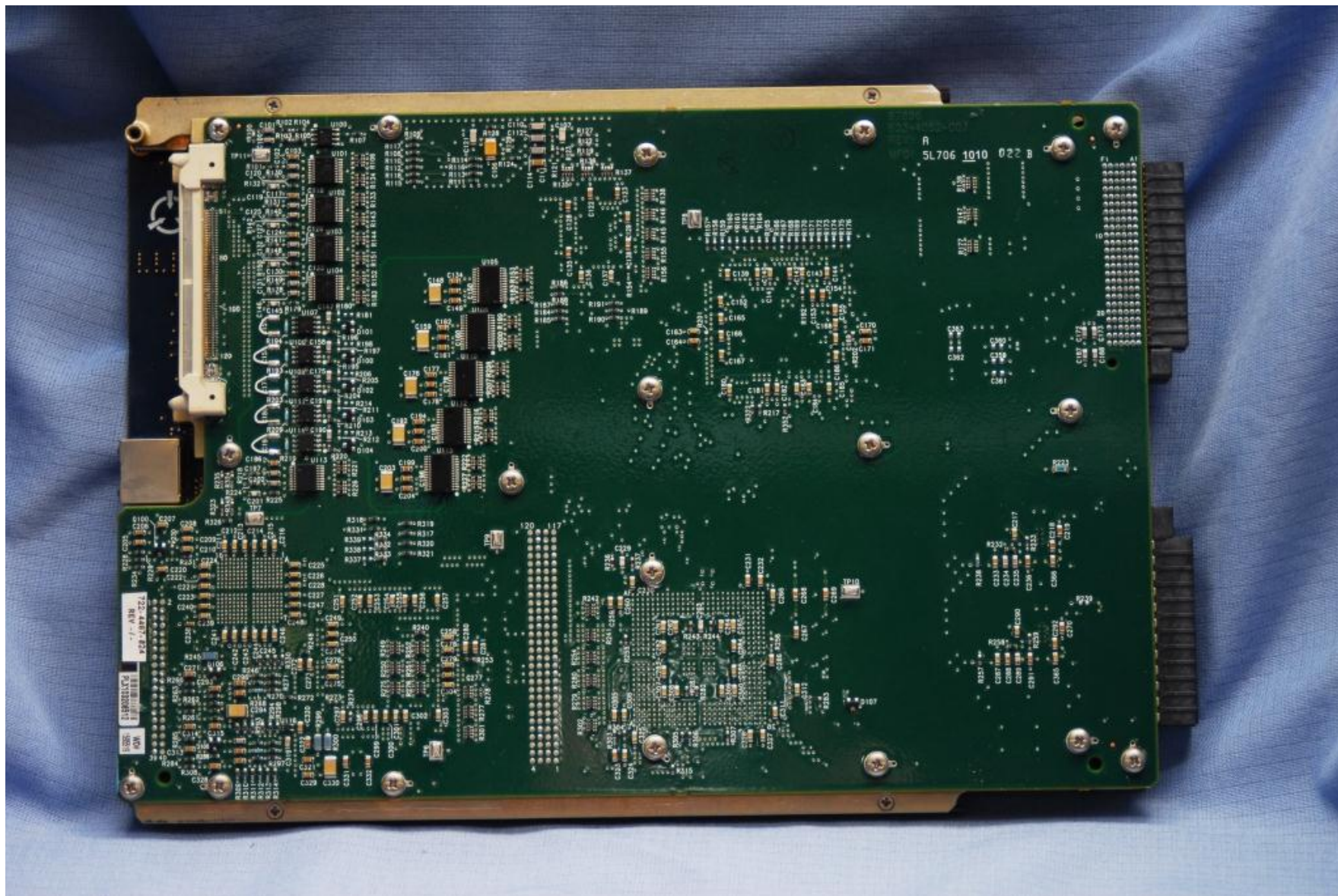
700-1750-022 (2) MODULE ASSEMBLY, TCAS / TRANSPONDER DIGITAL, AESU
