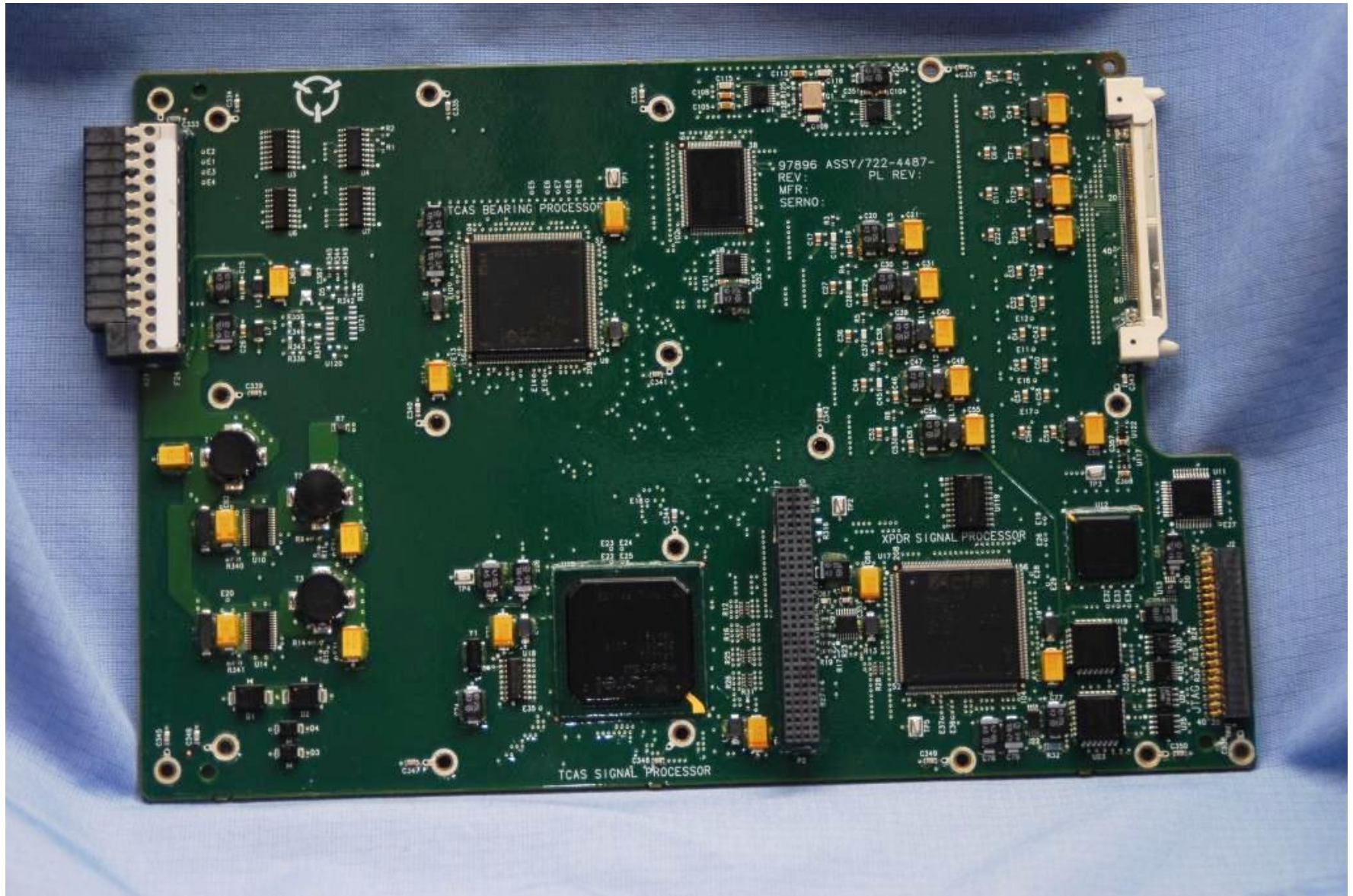
722-4487-024 (2) CCA / PWB, TPL DIGITAL MEZZANINE, AESU
