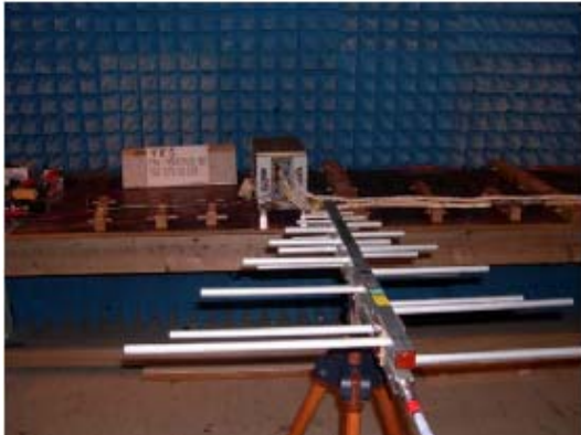
Antenna Test Unit Setup
