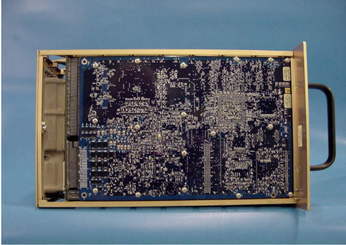
TPL-100A MILACAS-FR, Left Side View, Mezzanine/IO Processor Module (Digital)
