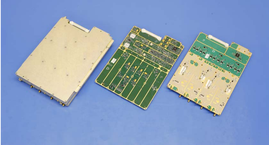
RECEIVER MODULE with two CCAs, side 2
