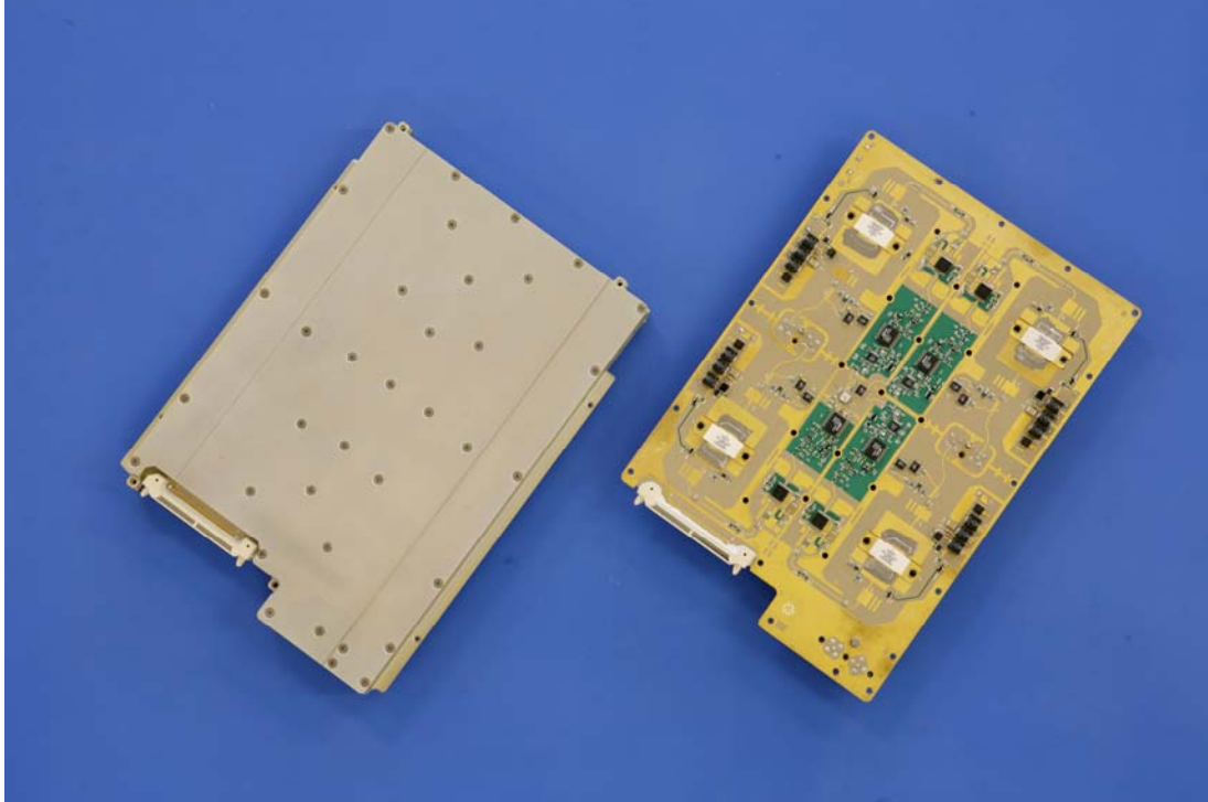
TRANSMITTER MODULE with one CCA, side 2
