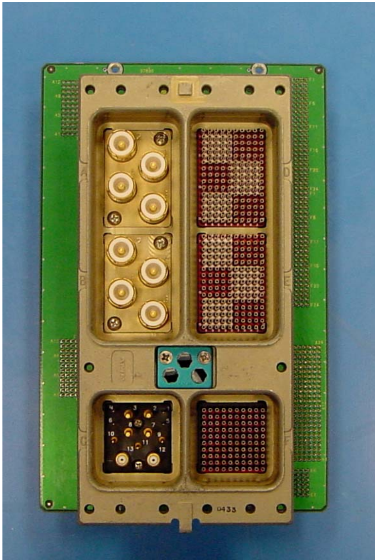
Rear Interconnect Assembly, ARINC 600 Connector, Rear View
