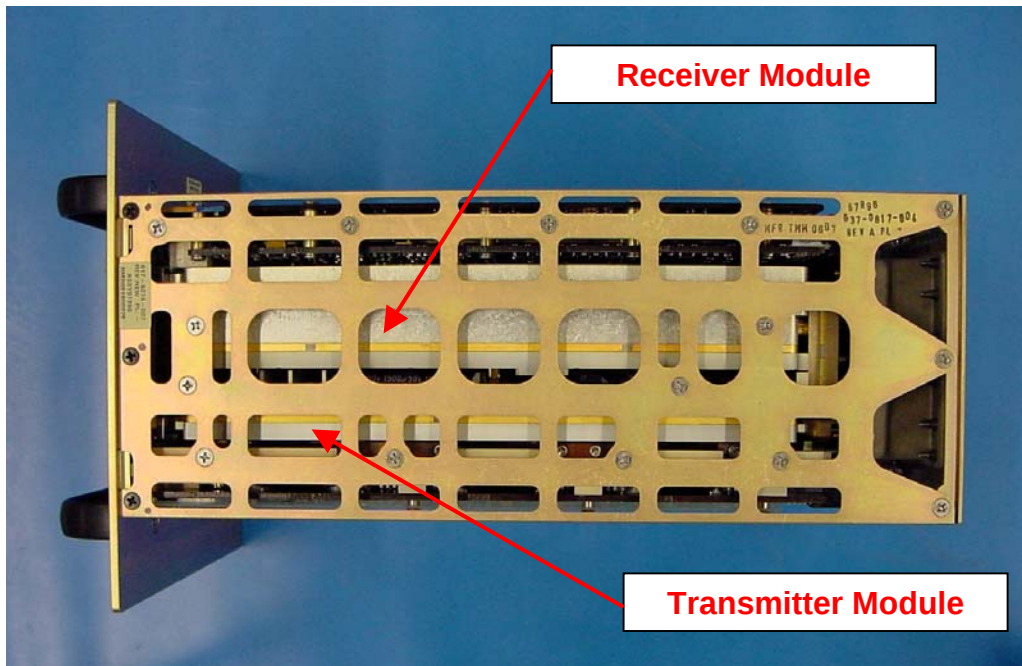
TPL-100A MILACAS-FR, Top View, Module Locations
