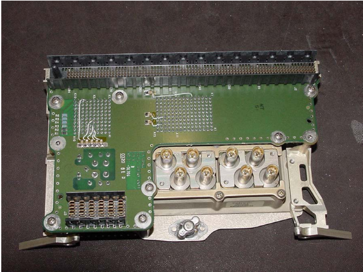
Rear Interconnect 1
