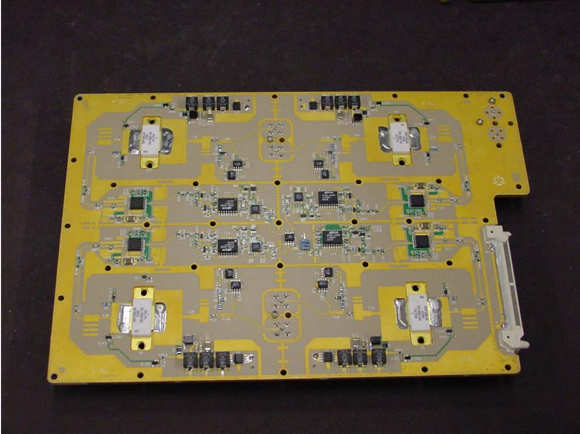
Transmitter 1
