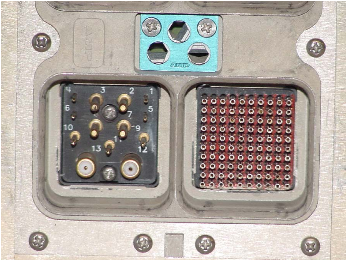
ARINC Shell ID (C) Power / Suppression
