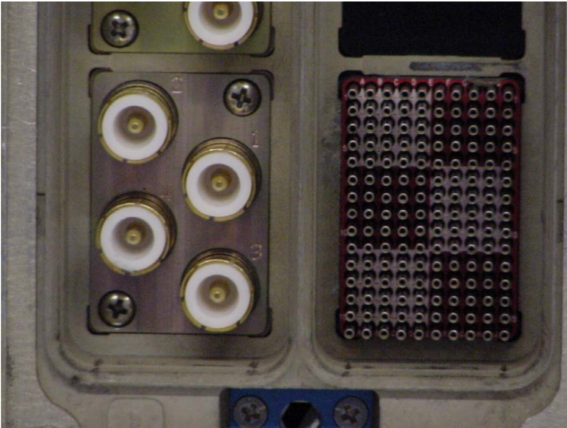
ARINC Shell ID (B) Bottom Antenna coax connections
