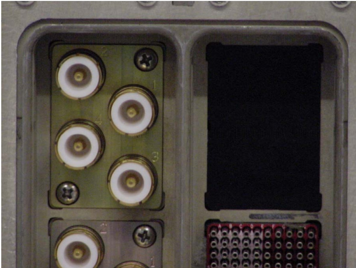
ARINC Shell ID (A) Top antenna coax connectors
