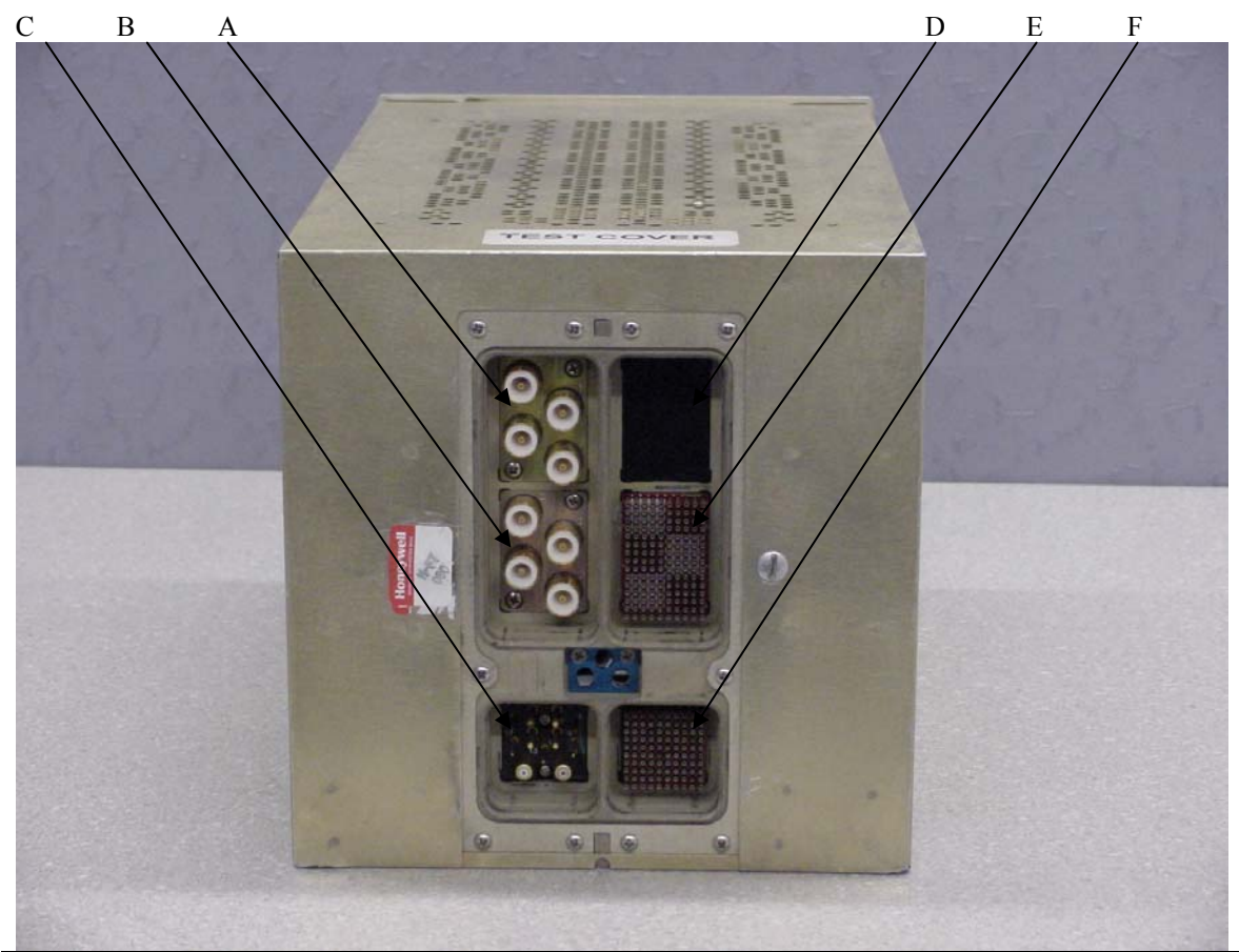
Back side (ARINC Connector)
