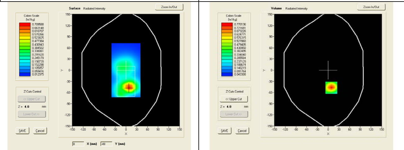
SAR, Z Axis Scan (X = 9, Y = -47)
