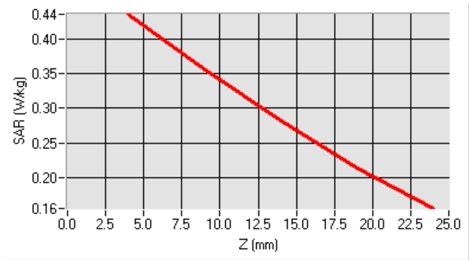
SAR, Z Axis Scan (X = -48, Y = -31)
