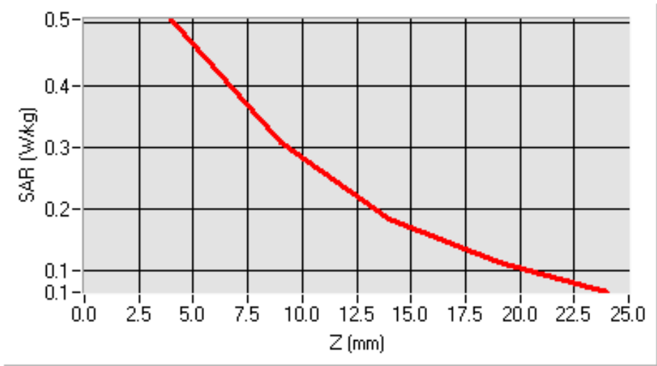
SAR, Z Axis Scan (X = -65, Y = -31)
