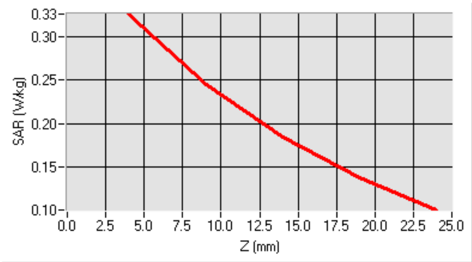
SAR, Z Axis Scan (X = 1, Y = -55)
