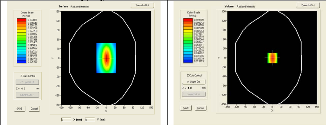
SAR, Z Axis Scan (X = 1, Y = -1)
