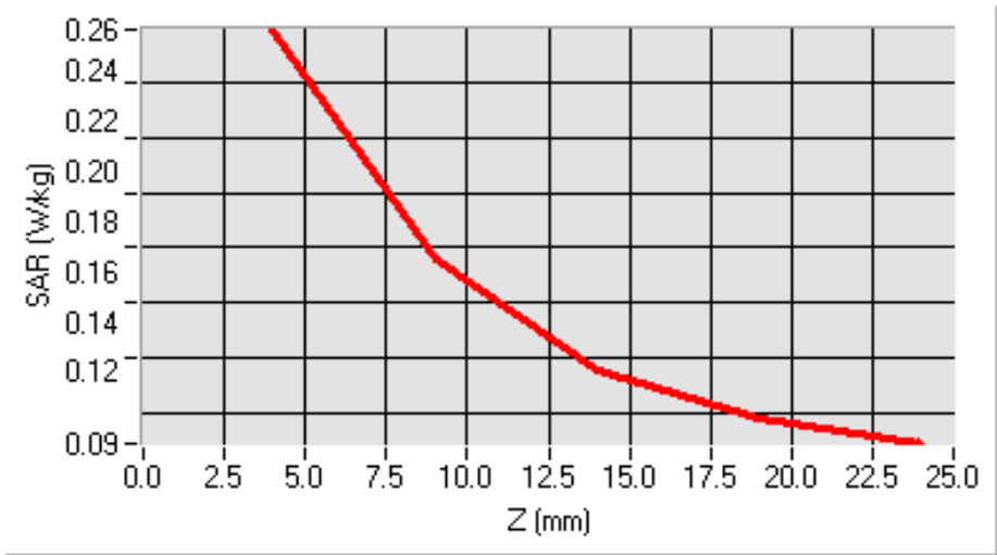
SAR, Z Axis Scan (X = -55, Y = -19)
