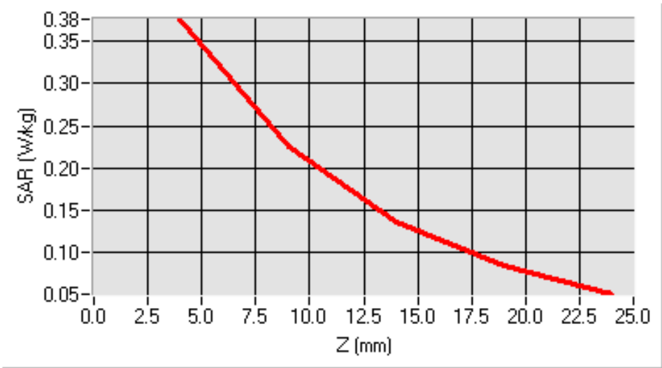
SAR, Z Axis Scan (X = -10, Y = -58)
