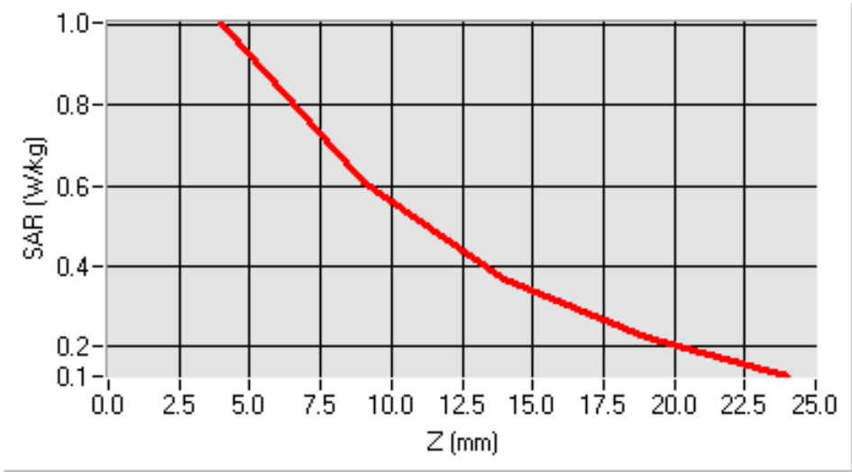
SAR, Z Axis Scan (X = 9, Y = -47)
