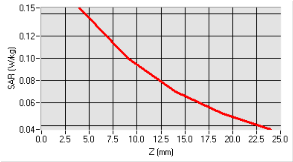
SAR, Z Axis Scan (X = -15, Y = 15)
