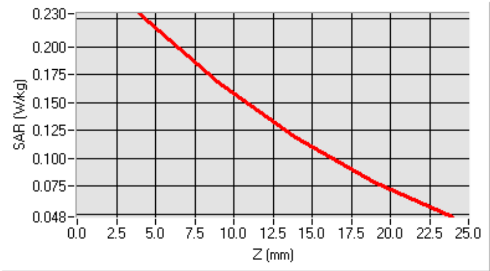
SAR, Z Axis Scan (X = -26, Y = -11)
