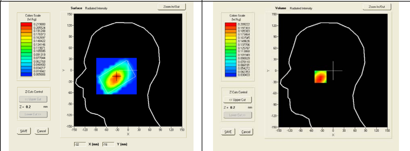
SAR, Z Axis Scan (X = -32, Y = -16)
