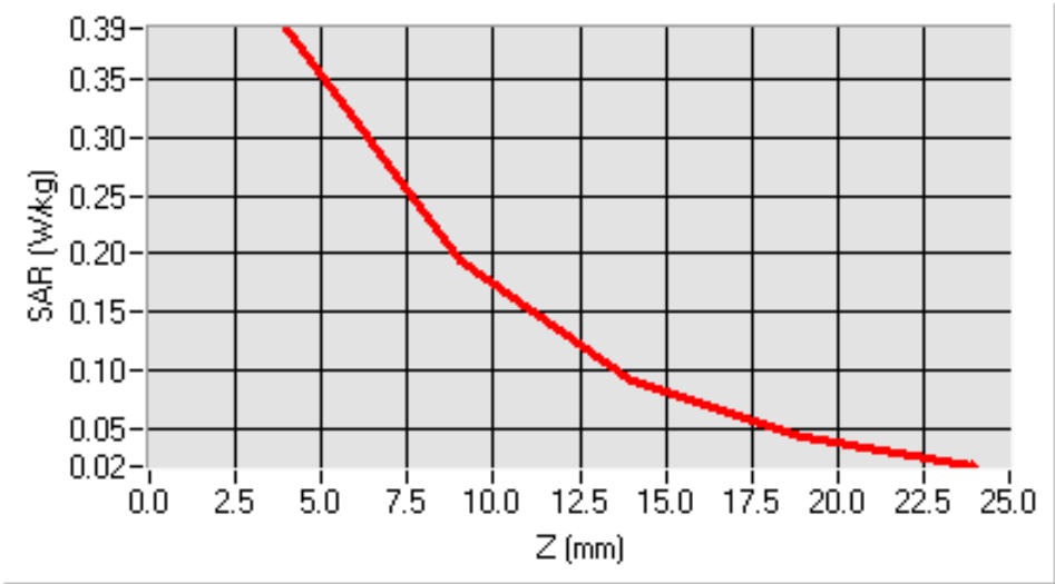
SAR, Z Axis Scan (X = -64, Y = -32)
