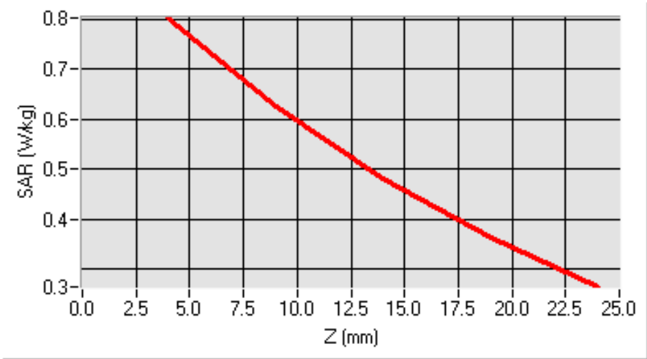
SAR, Z Axis Scan (X = -43, Y = -28)
