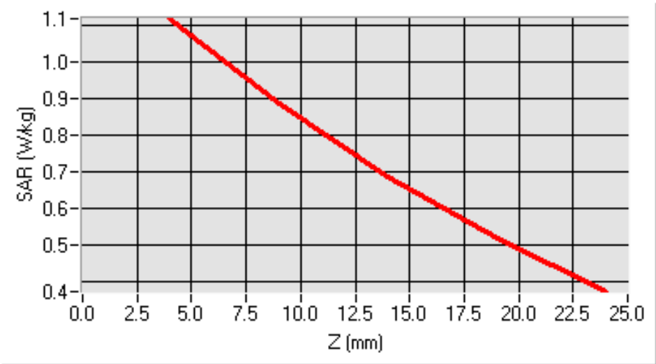
SAR, Z Axis Scan (X = -1, Y = -48)
