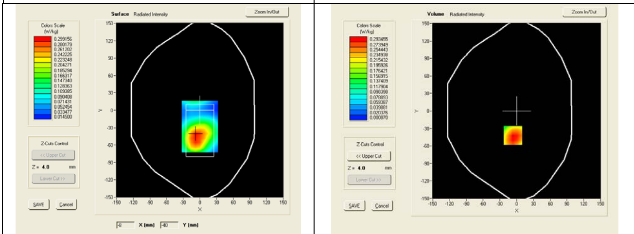
SAR, Z Axis Scan (X = -7, Y = -42)
