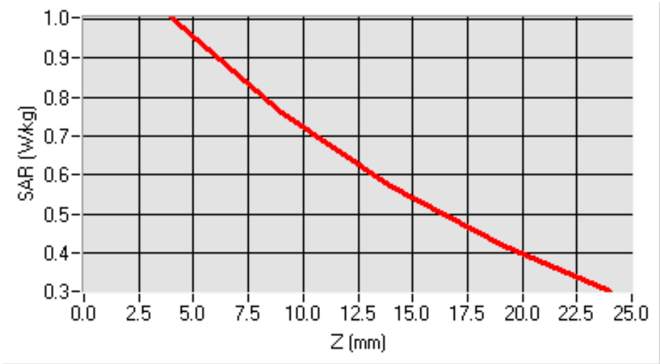
SAR, Z Axis Scan (X = -2, Y = -57)
