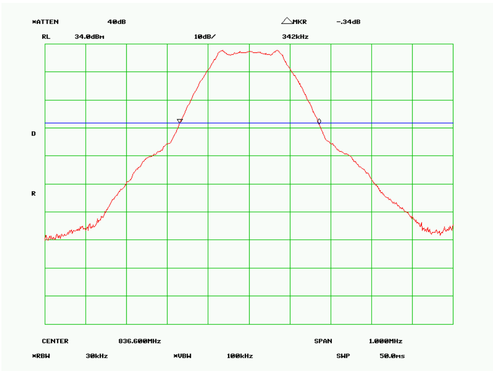
26 dB Bandwidth
