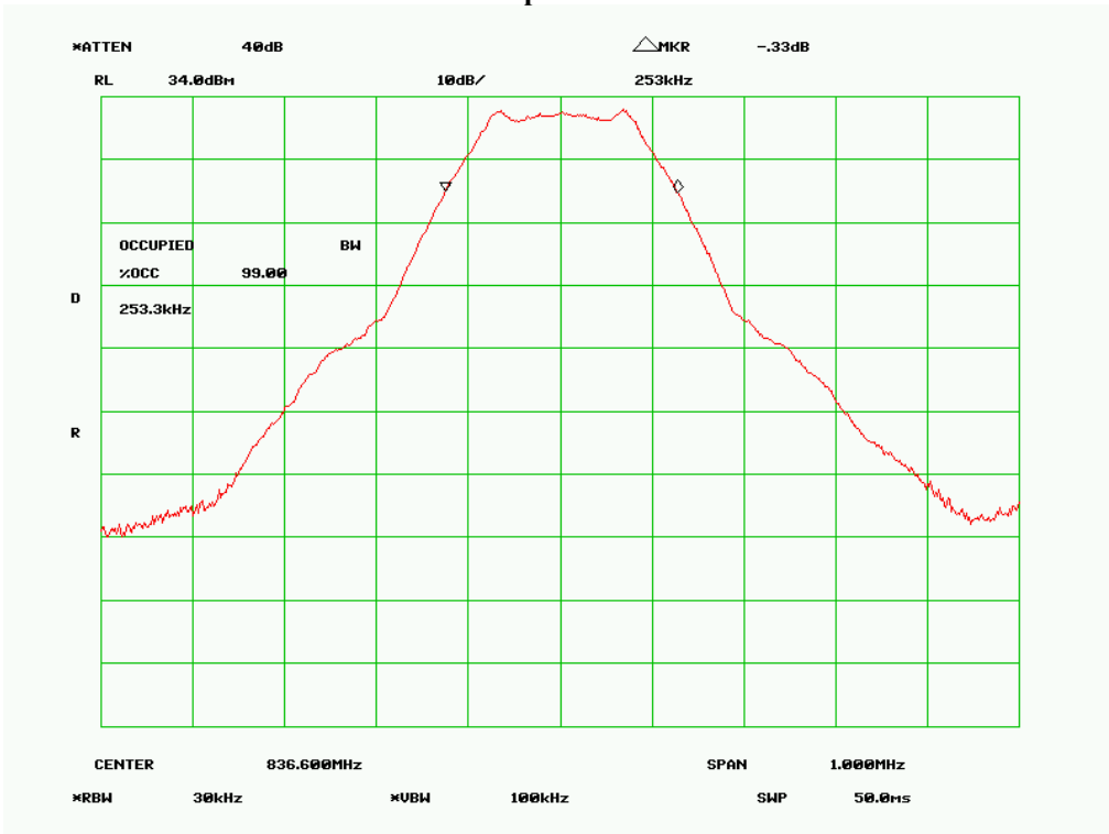
99% Occupied Bandwidth
