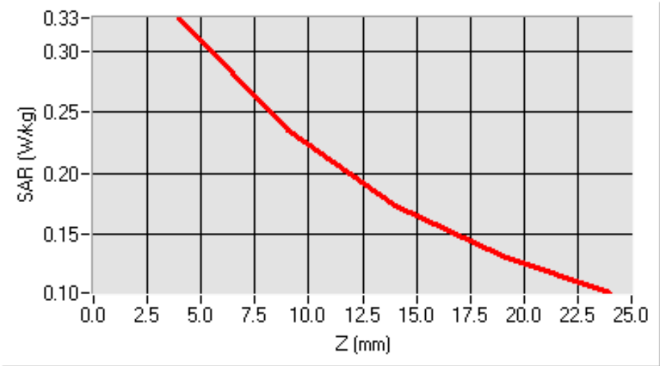
SAR, Z Axis Scan (X = -47, Y = -25)
