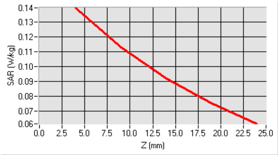
SAR, Z Axis Scan (X = -48, Y = -39)
