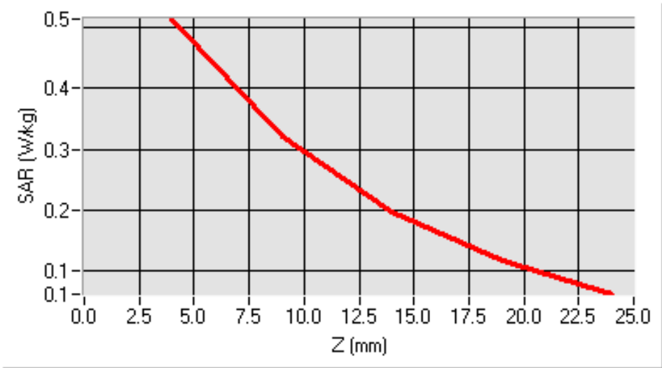
SAR, Z Axis Scan (X = -40, Y = -41)
