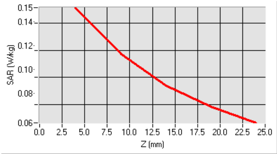
SAR, Z Axis Scan (X = -42, Y = -38)
