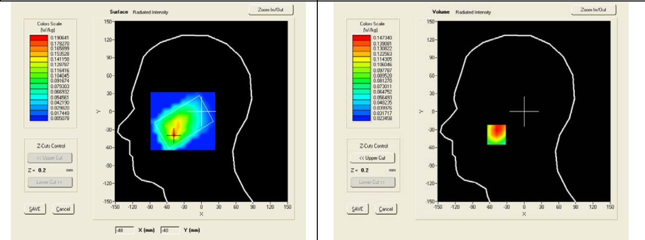
SAR, Z Axis Scan (X = -48, Y = -39)
