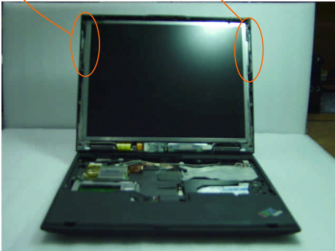
Right side antenna ( Inverted-F type ) for WLAN : Rx only for Bluetooth : Tx / Rx
