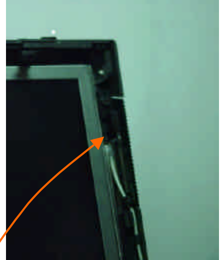
Right side antenna ( Inverted-F type ) for WLAN : Rx only for Bluetooth : Tx / Rx
