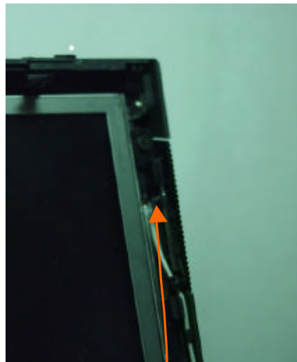
Right side antenna Inverted-F type Rx only
