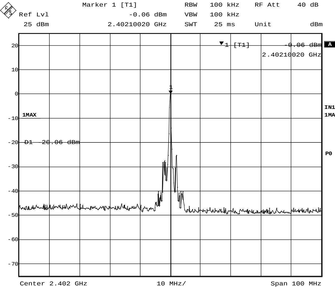
Out of Band Emissions (TX on 2402MHz)
