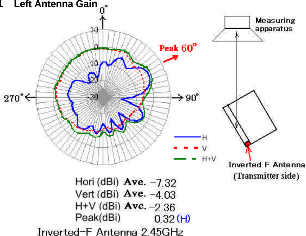
Figure 1 Left Antenna Gain
