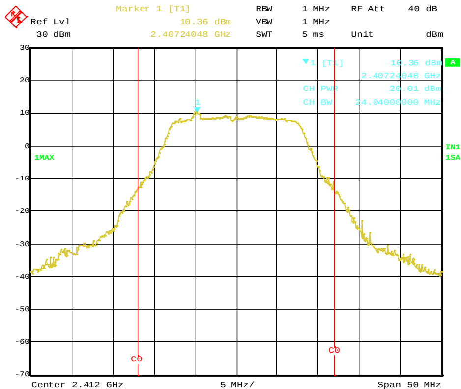
Plot 3-2b. Conducted Peak Output Power of 2412MHz (OFDM, 6Mbps)
