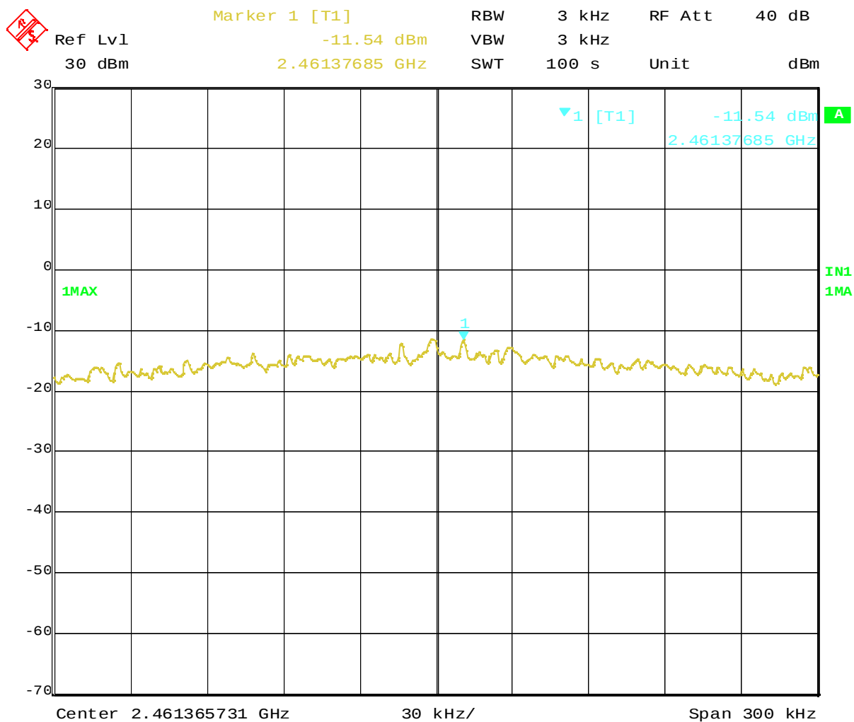
Plot 5-2. Peak Power Spectral Density of 2462MHz (OFDM, 6Mbps)
