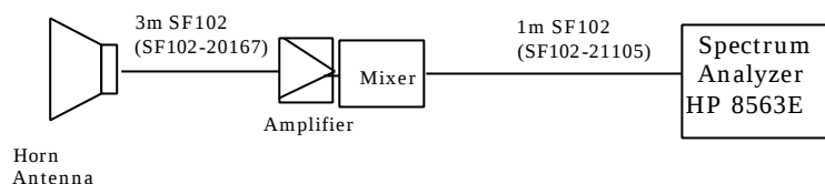
Figure 8-4. Cables for Radiated Emission Test (26.5 - 40GHz)
