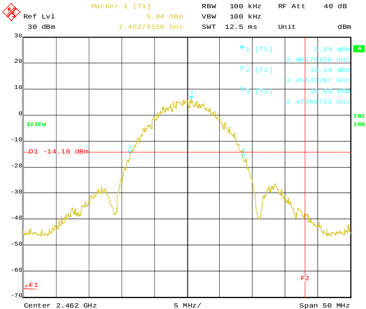
Plot 2-2. 20dB BW at 2462MHz (DSSS, 11Mbps)
