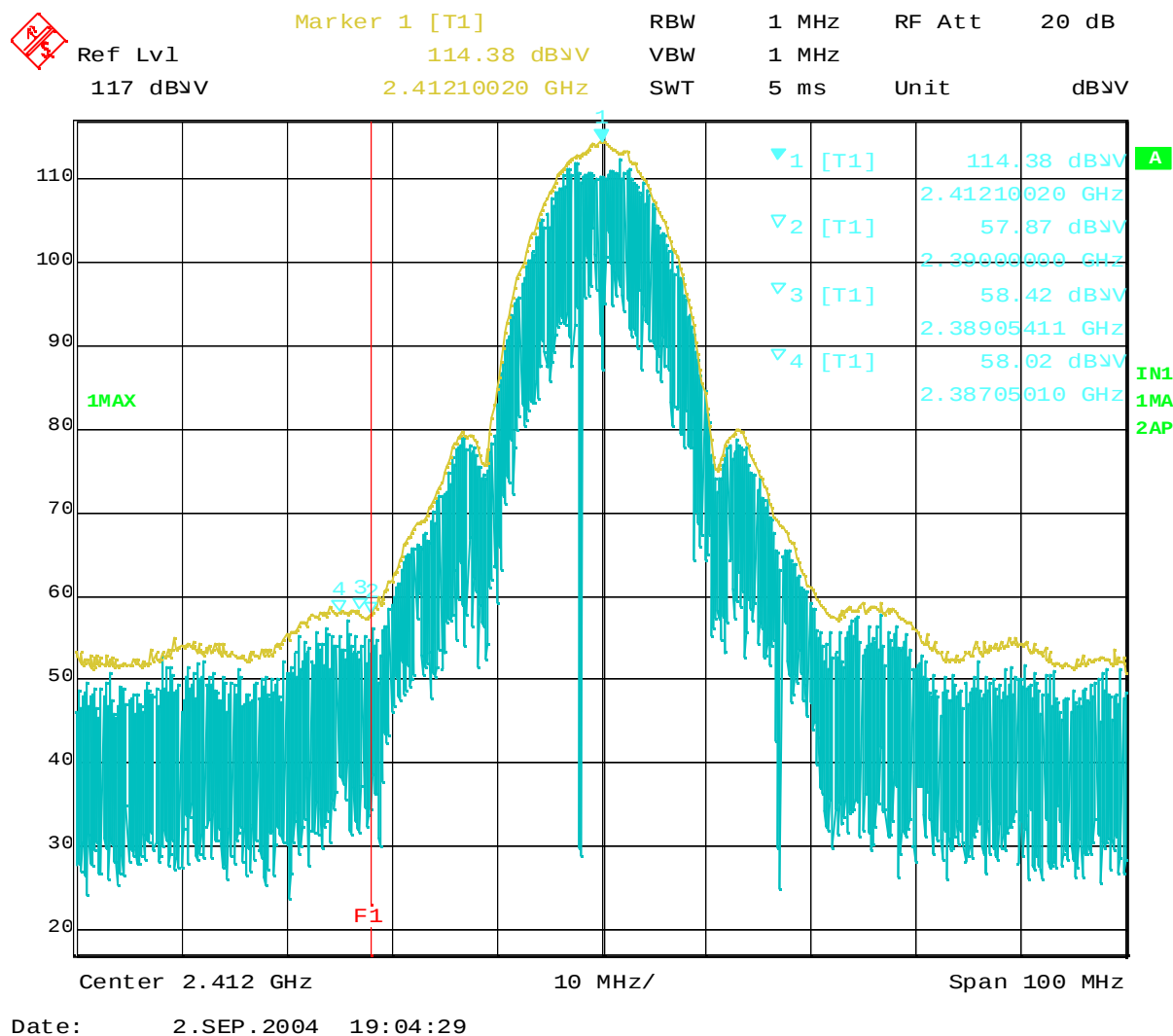
Plot 8-1 Ch.1 2412MHz TX, DSSS 11Mbps (Peak), T40 Series 14" model
