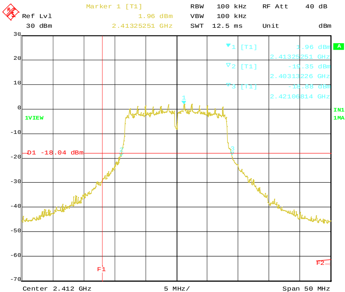
Plot 2-3. 20dB BW at 2412MHz (OFDM, 6Mbps)
