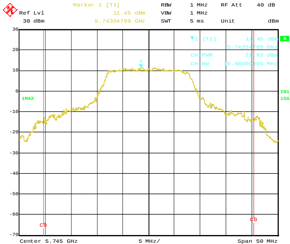
Plot 3-3b. Conducted Peak Output Power of 5745MHz (OFDM, 6Mbps)
