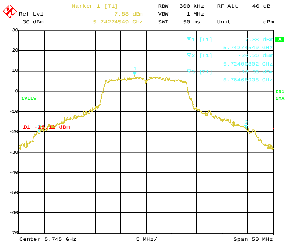
Plot 3-3a. 26dB Bandwidth of 5745MHz (OFDM, 6Mbps)
