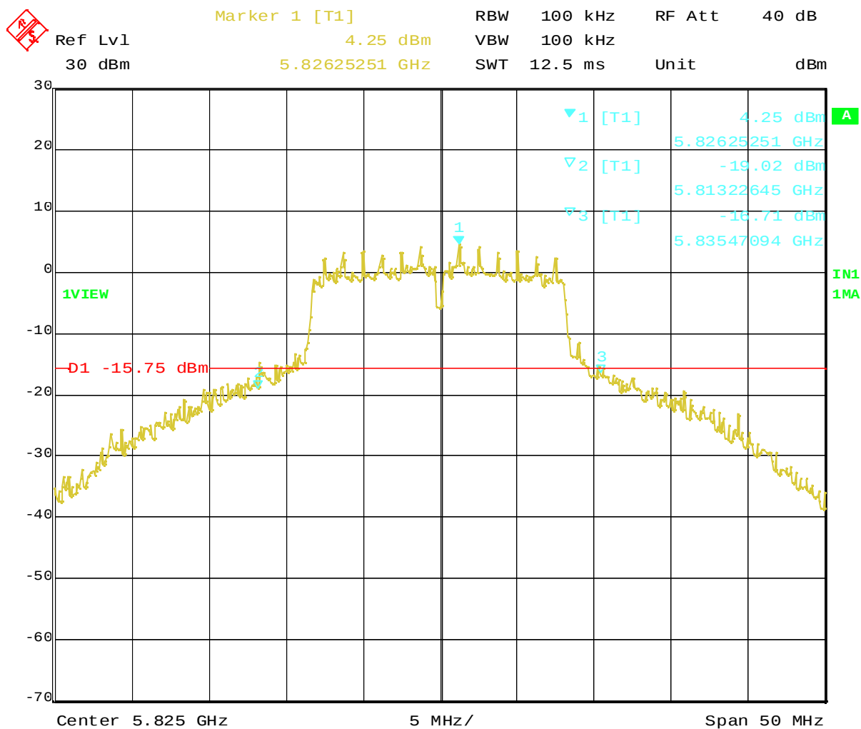
Plot 2-6. 20dB BW at 5825MHz (OFDM, 6Mbps)
