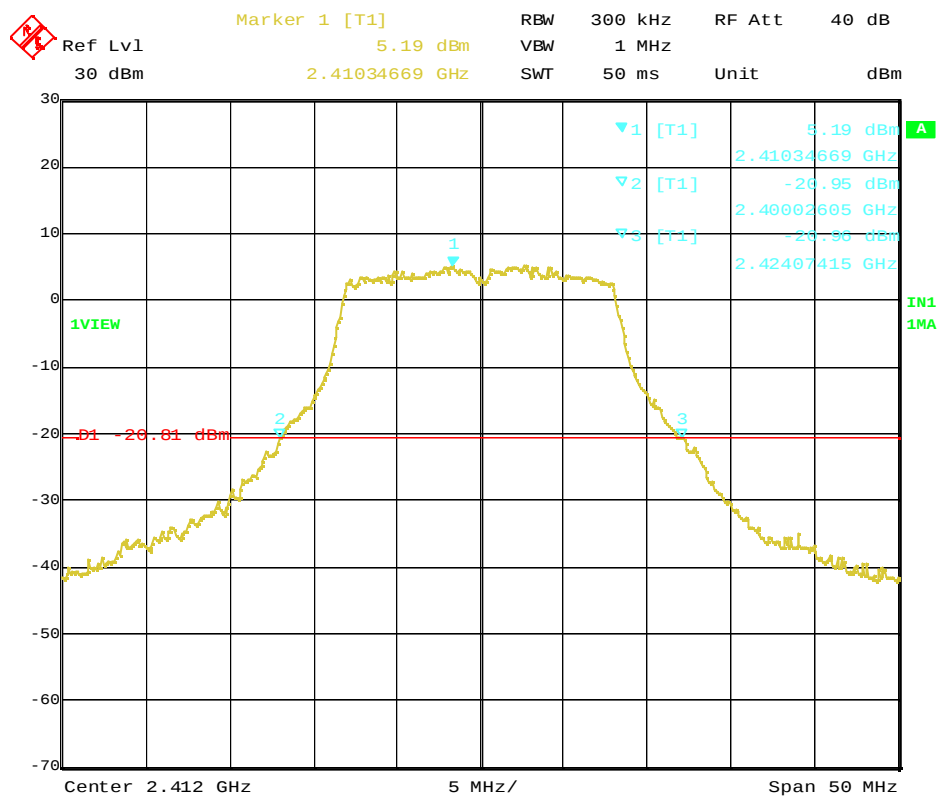
Plot 3-2a. 26dB Bandwidth of 2412MHz (OFDM, 6Mbps)
