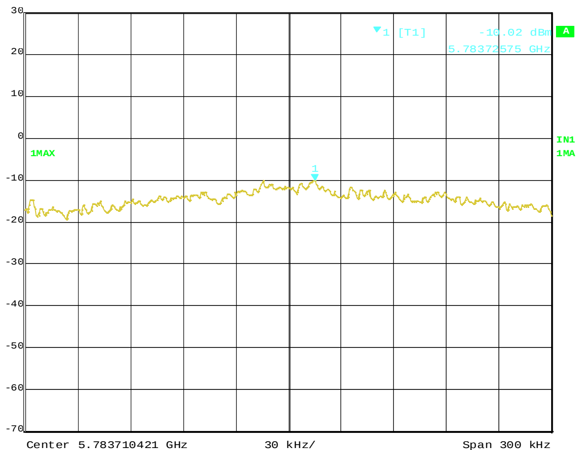
Plot 5-3. Peak Power Spectral Density of 5785MHz (OFDM, 6Mbps)
