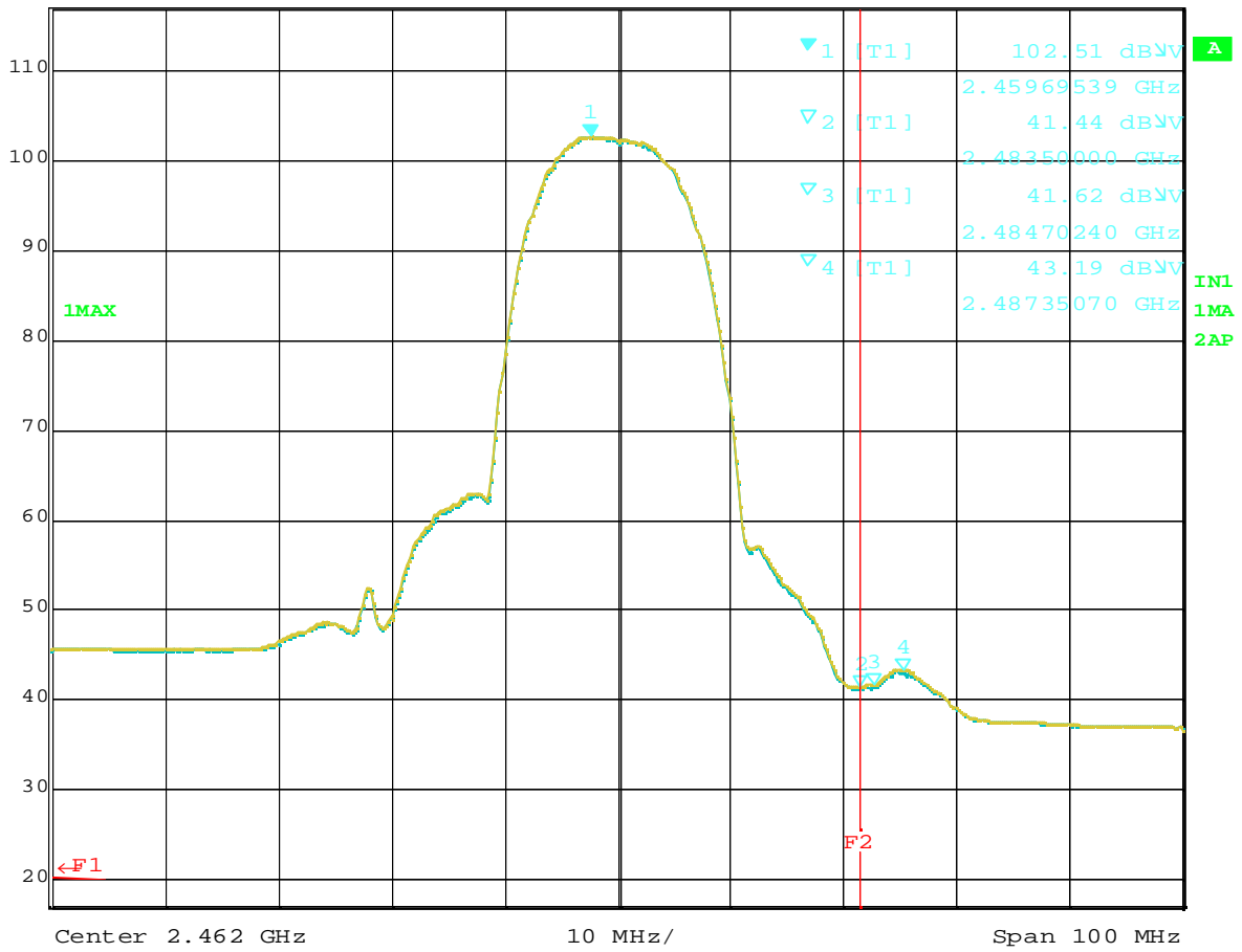
Plot 8-4 Ch.11 2462MHz TX, DSSS 11Mbps (Average), 14" model
