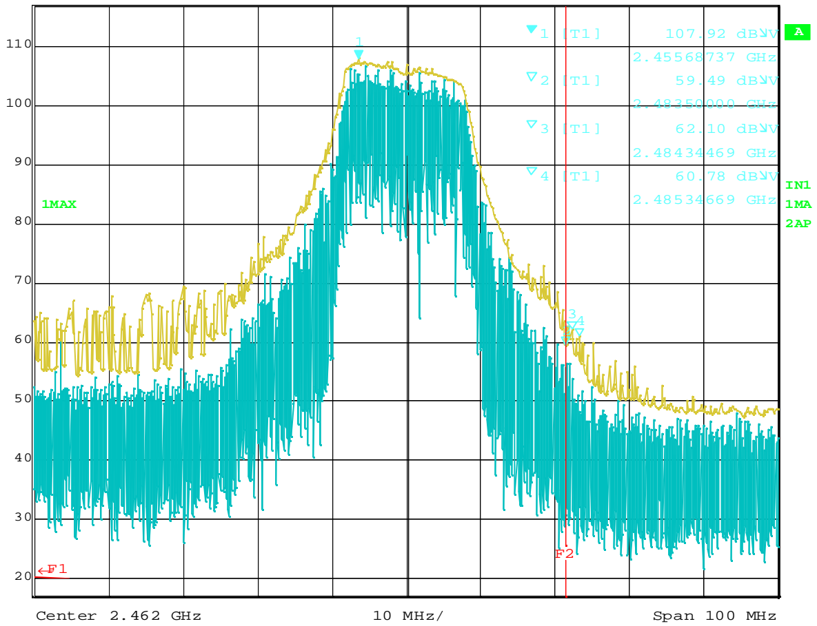
Plot 8-7 Ch.11 2462MHz TX. OFDM 6Mbps (Peak). 14" model
