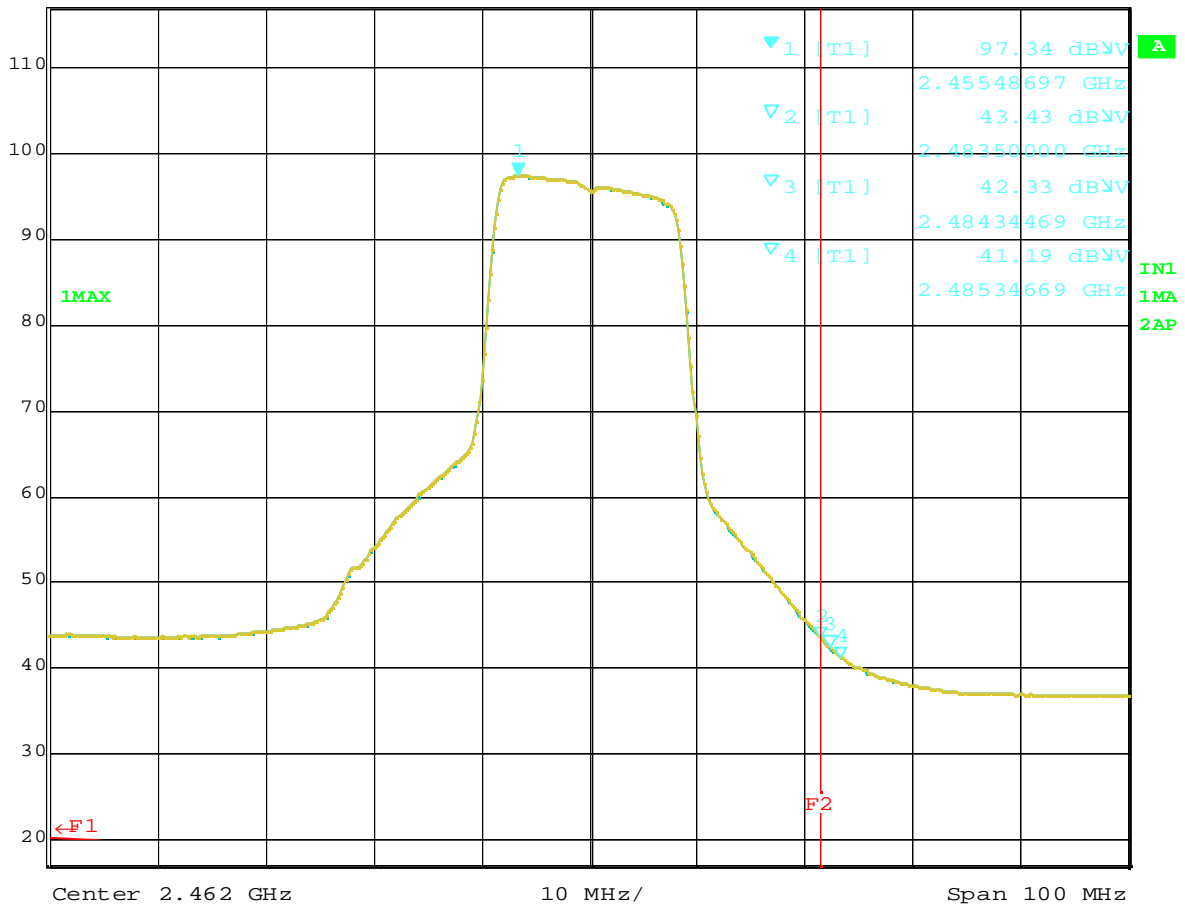
Plot 8-8 Ch.11 2462MHz TX, OFDM 6Mbps (Average), 14" model
