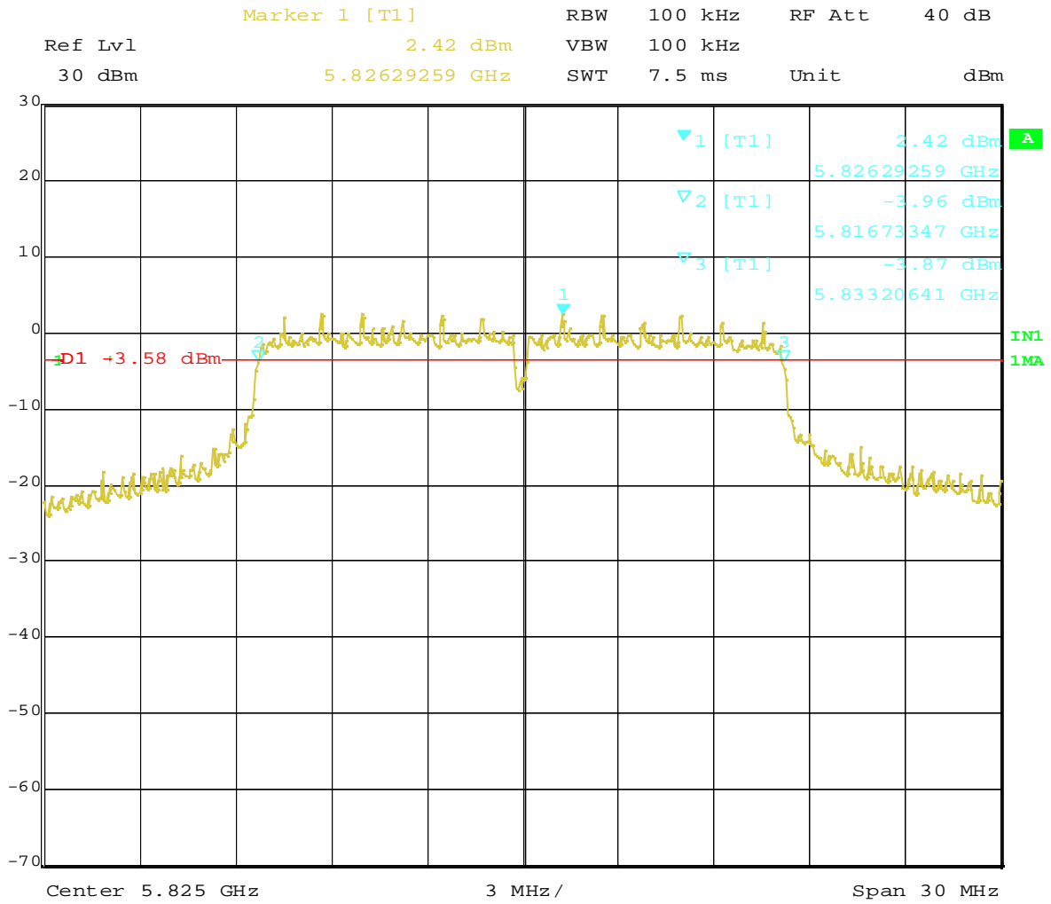
Plot 1-3. 6dB BW at 5825MHz (OFDM, 6Mbps)
