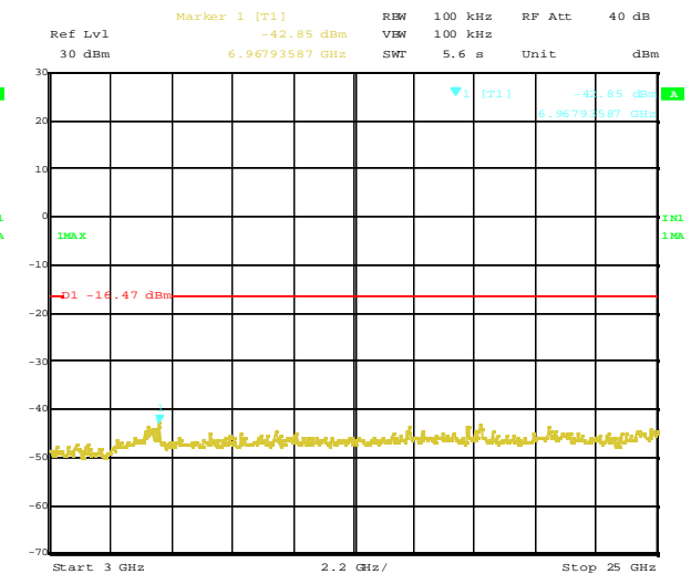
Plot 4-5. Out of band emissions around 2437MHz (OFDM, 6Mbps)
