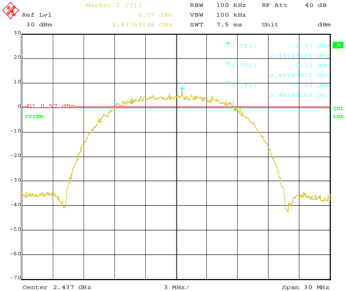
Plot 1-1. 6dB BW at 2437MHz (DSSS, 11Mbps)
