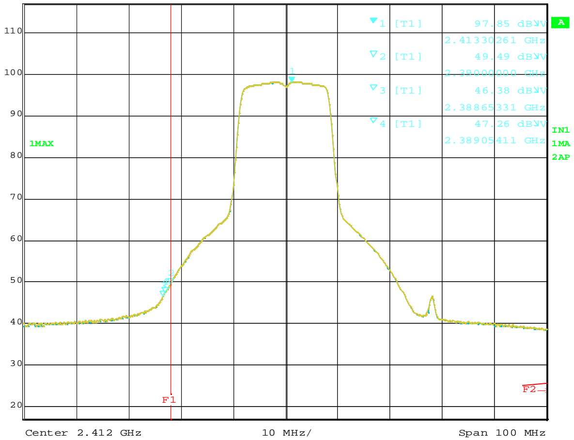
Plot 8-6 Ch.1 2412MHz TX. OFDM 6Mbps (Average). 14" model
