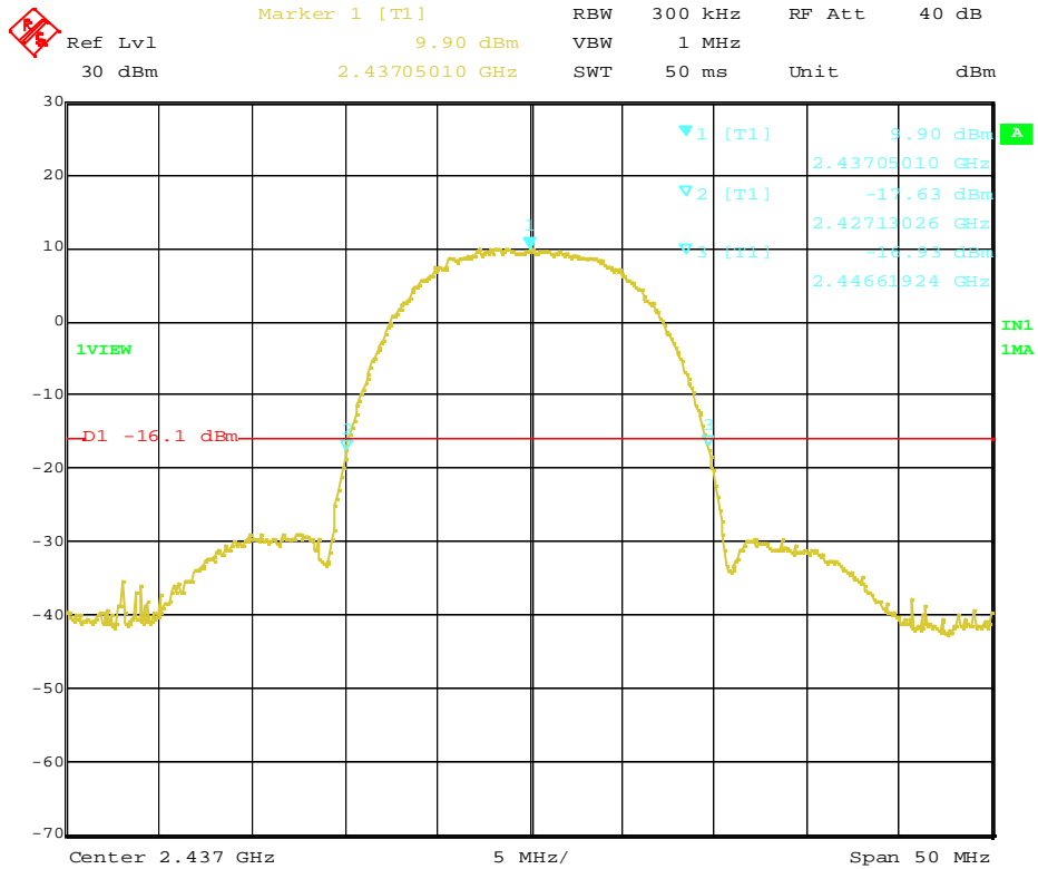
Plot 3-1a. 26dB Bandwidth of 2437MHz (DSSS, 11Mbps)
