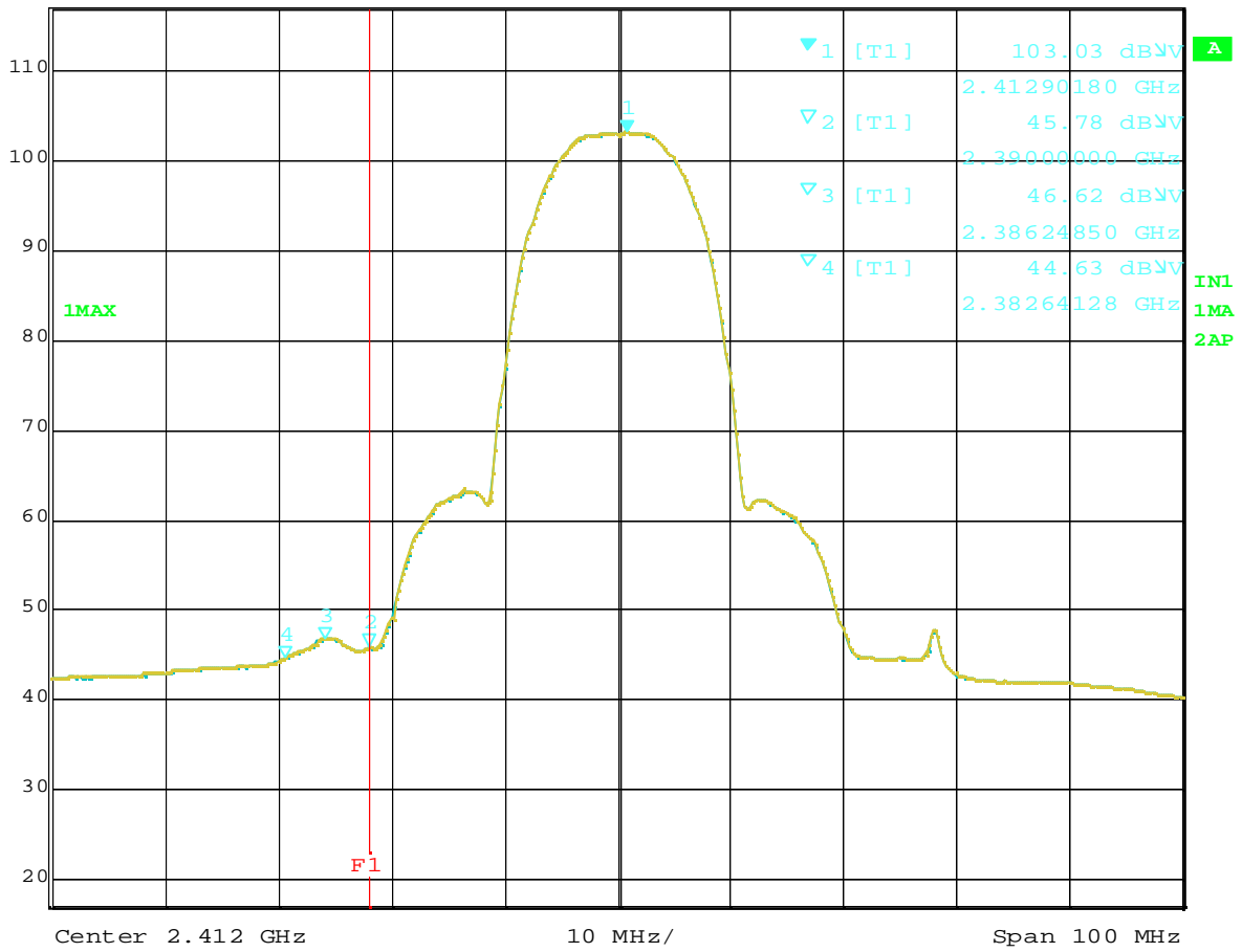
Plot 8-2 Ch.1 2412MHz TX, DSSS 11Mbps (Average), 14" model
