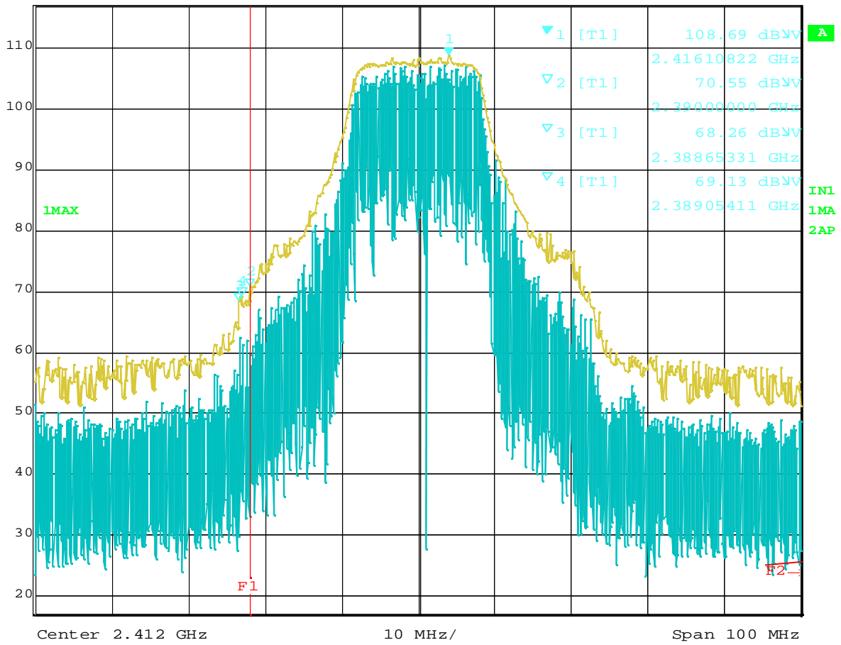
Plot 8-5 Ch.1 2412MHz TX, OFDM 6Mbps (Peak), 14" model
