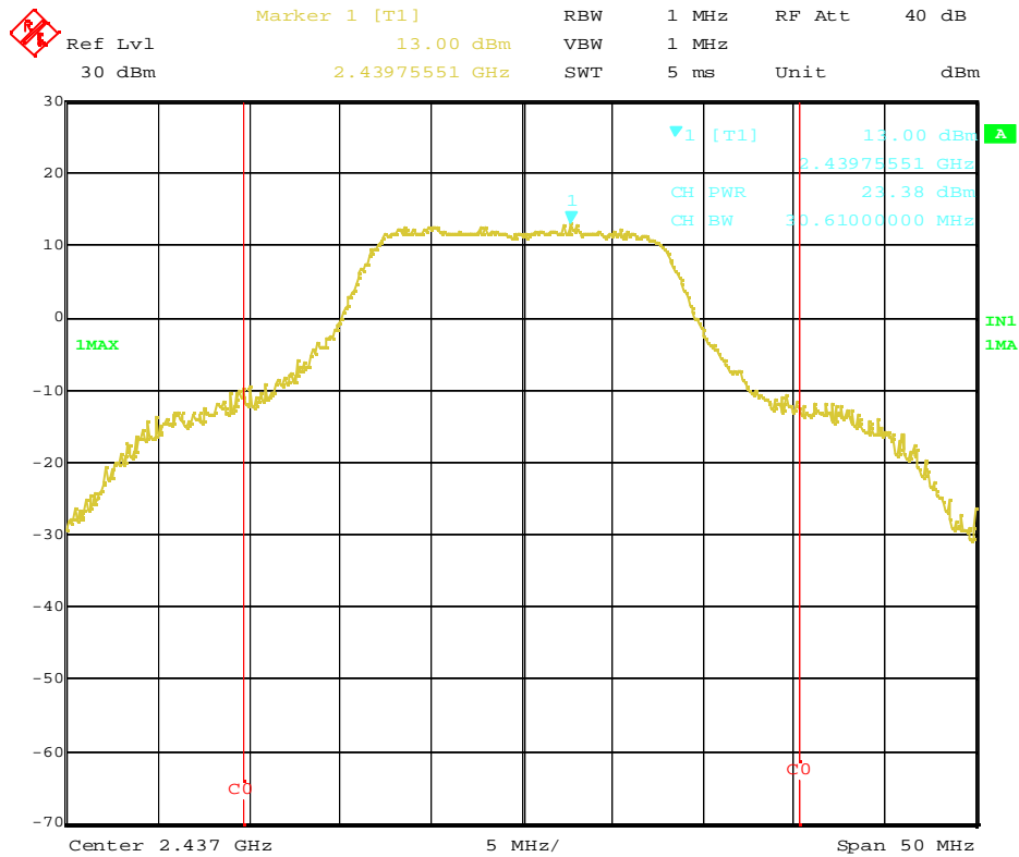
Plot 3-2b. Conducted Peak Output Power of 2437MHz (OFDM, 6Mbps)
