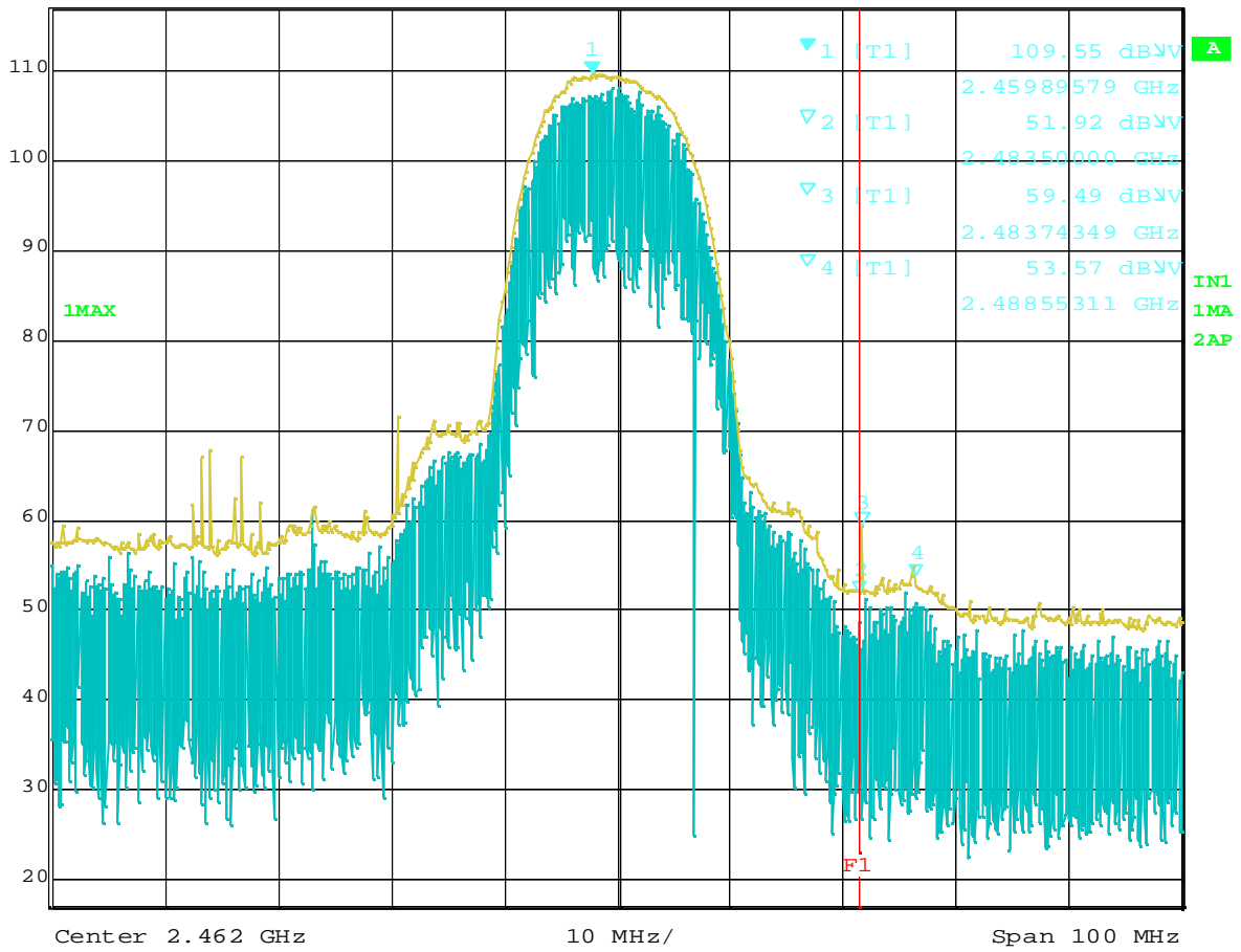
Plot 8-3 Ch.11 2462MHz TX, DSSS 11Mbps (Peak), 14" mode
