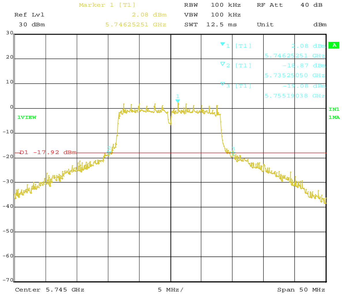
Plot 2-3. 20dB BW at 5745MHz (OFDM, 6Mbps)
