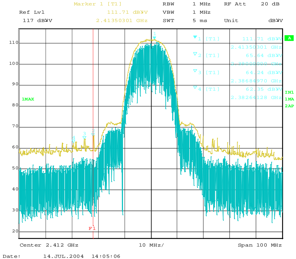
Plot 8-1 Ch.1 2412MHz TX, DSSS 11Mbps (Peak), 14" model
