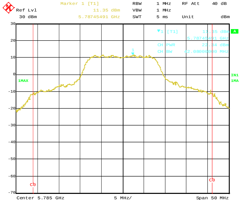
Plot 3-3b. Conducted Peak Output Power of 5785MHz (OFDM, 6Mbps)
