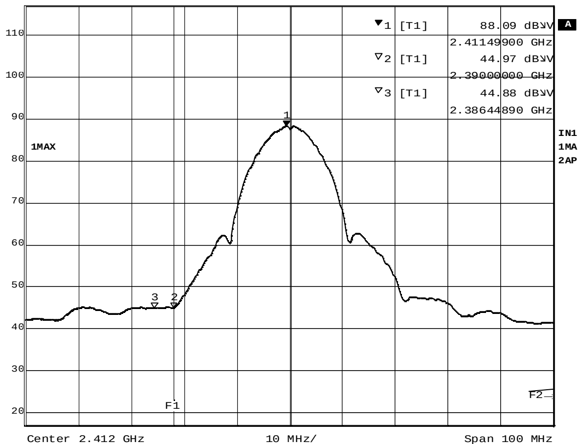
Plot 8-3-2 Ch.1 2412MHz TX. DSSS 11Mbps (Average). T40 Series
