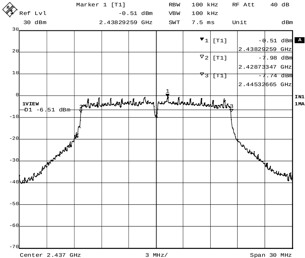
Plot 1-5. 6dB BW at 2437MHz (OFDM, 18Mbps)
