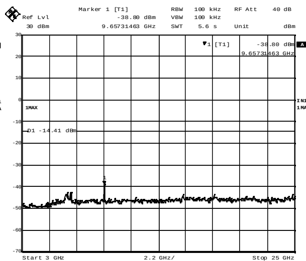
Plot 4-1. Out of band emissions around 2412MHz (DSSS, 5.5Mbps)
