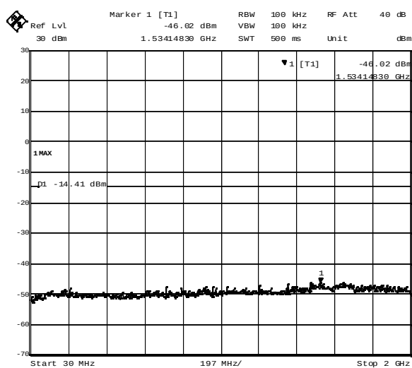
Plot 4-1. Out of band emissions around 2412MHz (DSSS, 5.5Mbps)
