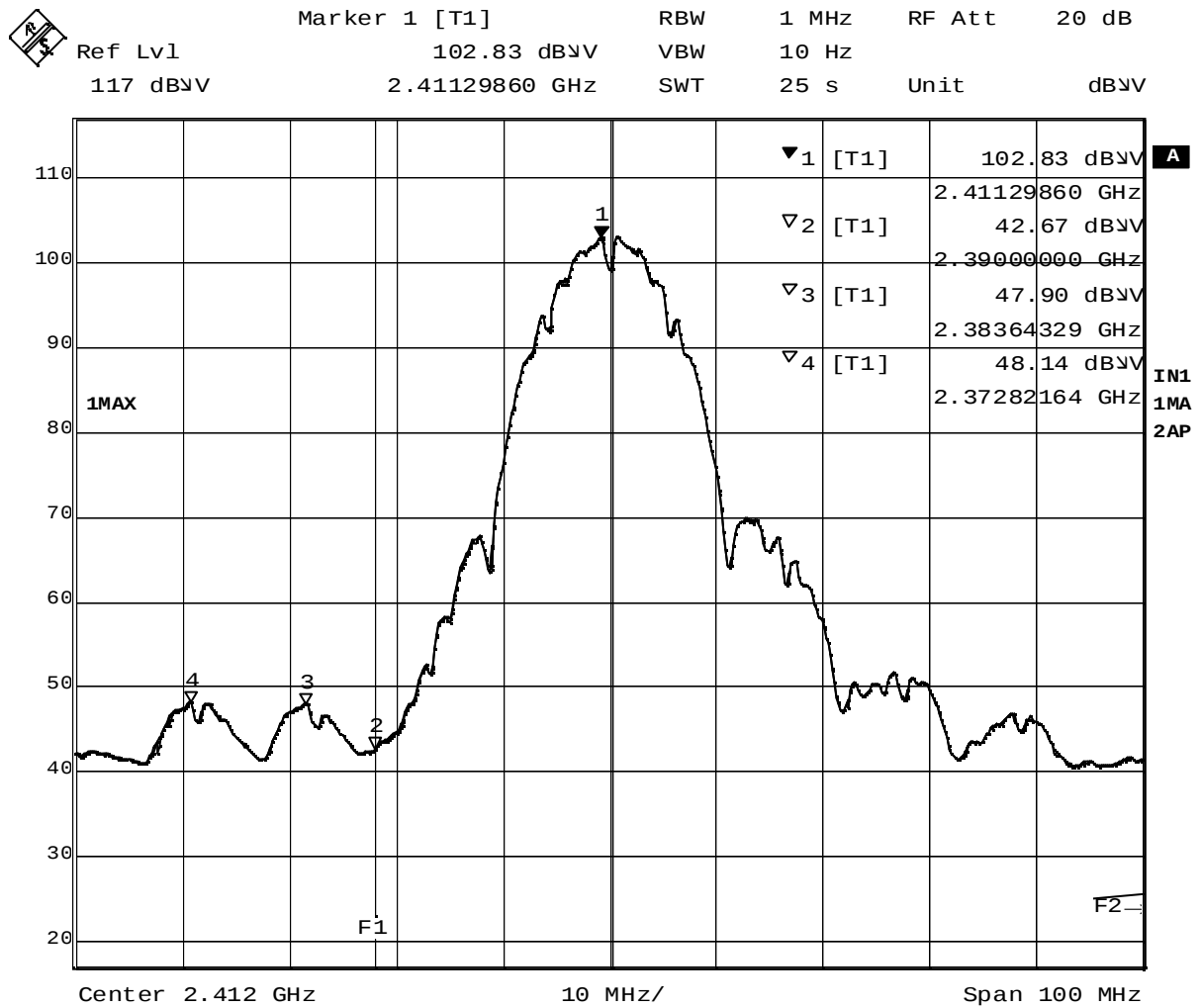
Plot 8-1-2 Ch.1 2412MHz TX, DSSS 1Mbps (Average), X30 Series
