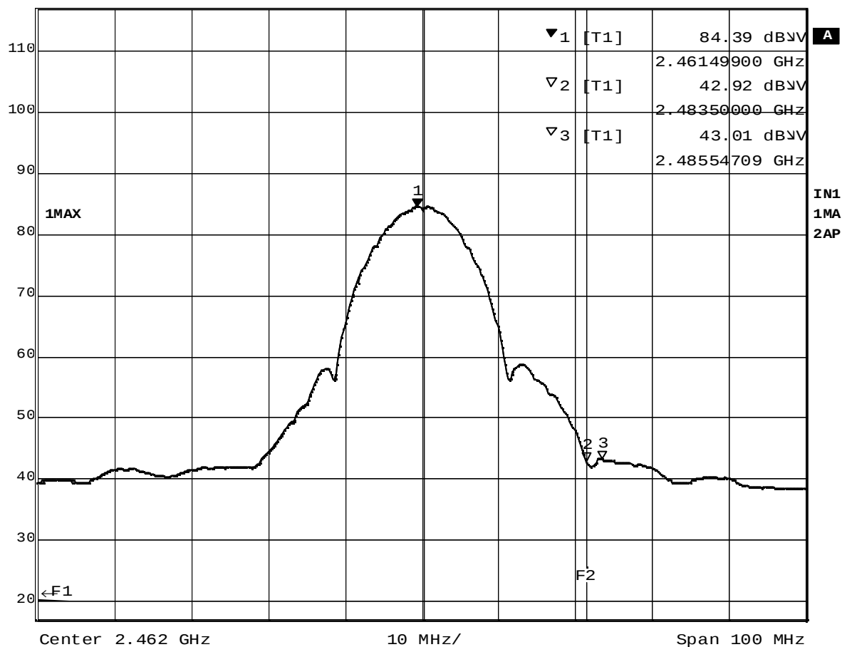
Plot 8-3-4 Ch.11 2462MHz TX, DSSS 11Mbps (Average), X30 Series
