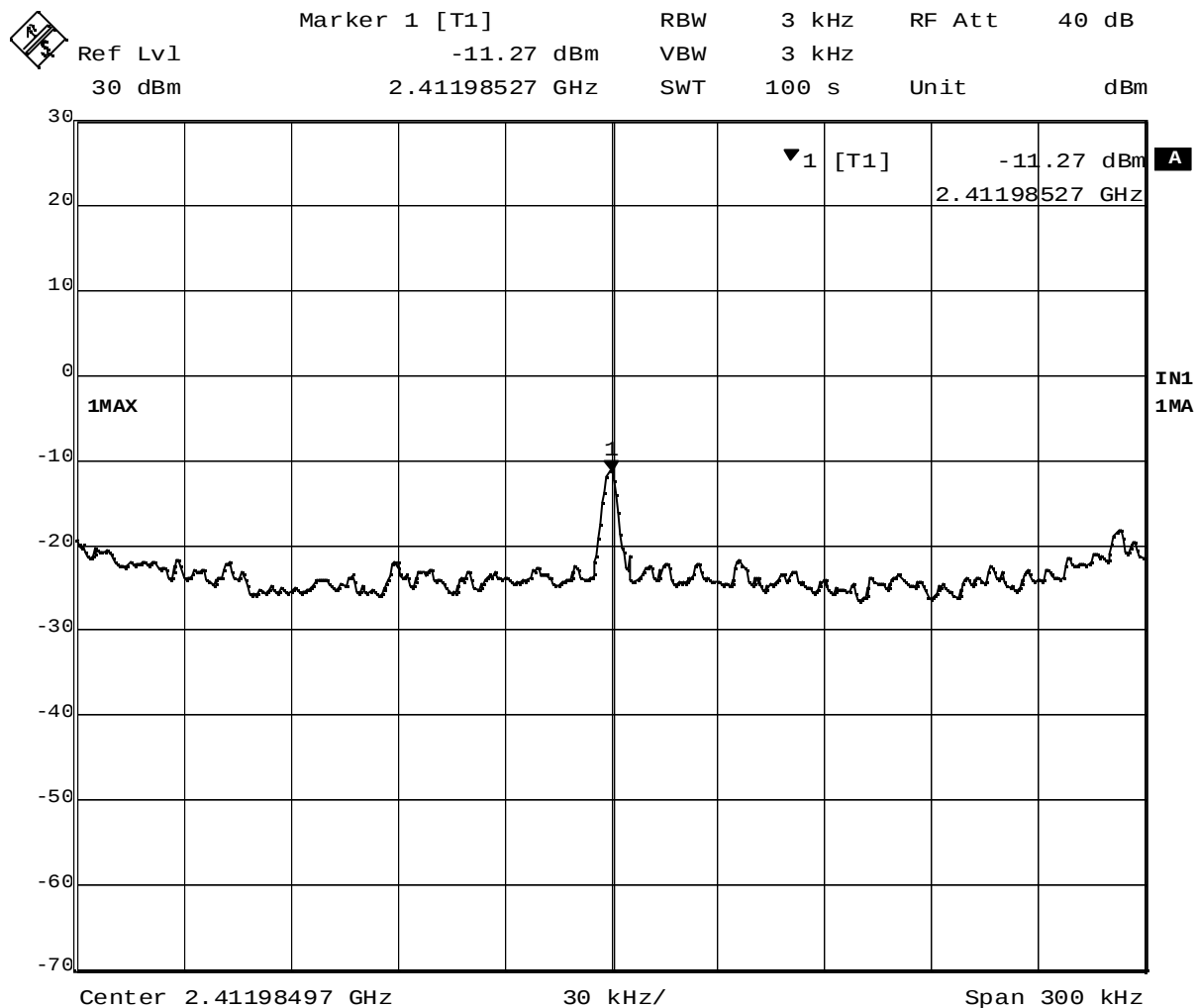
Plot 5-4. Peak Power Spectral Density of 2412MHz (OFDM, 18Mbps)
