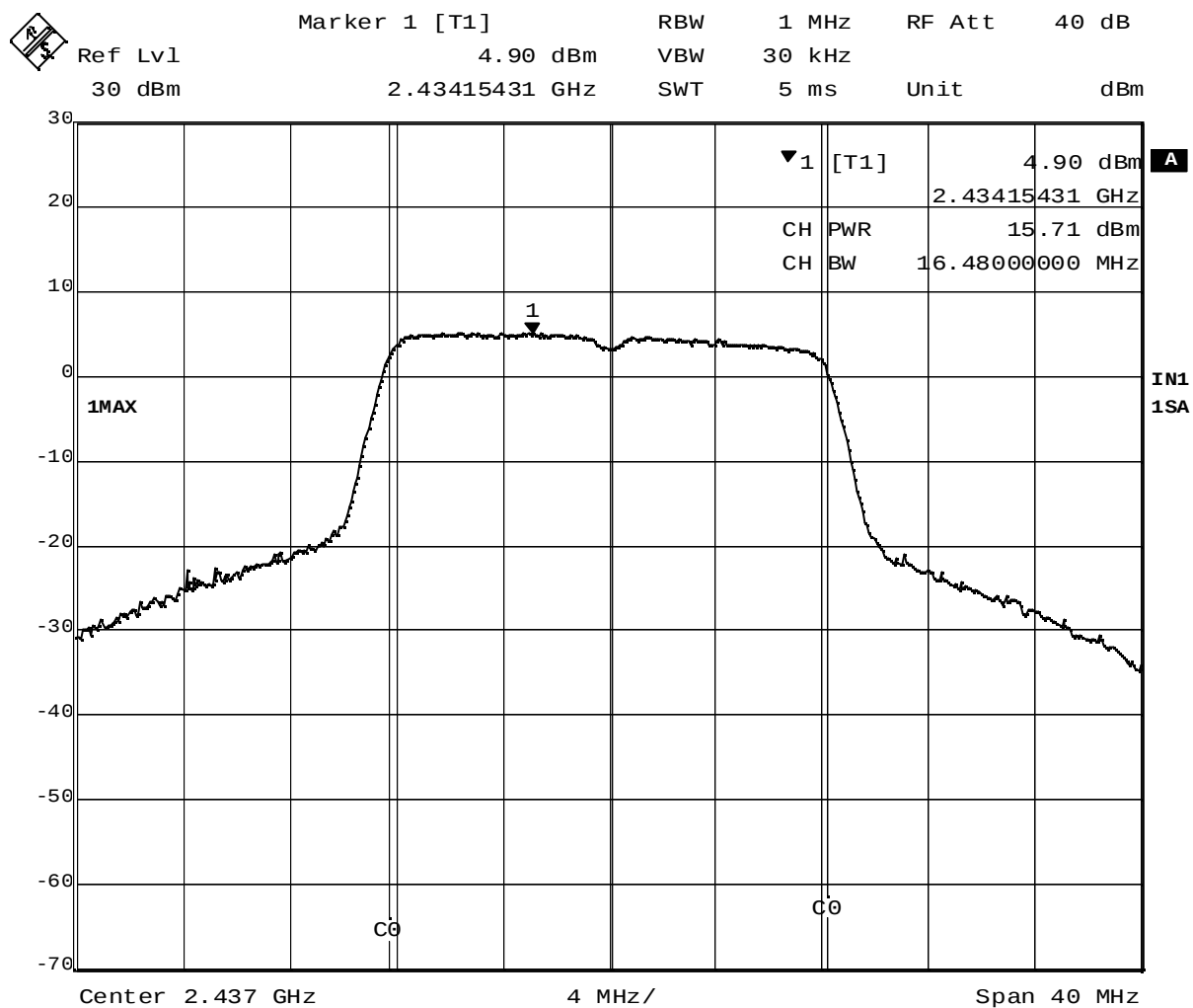
Plot 3-5. Conducted Peak Output Power of 2437MHz (OFDM, 18Mbps)
