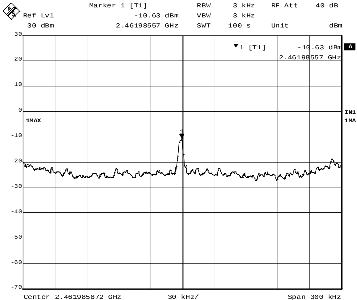
Plot 5-6. Peak Power Spectral Density of 2462MHz (OFDM, 18Mbps)
