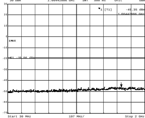
Plot 4-6. Out of band emissions around 2462MHz (OFDM, 18Mbps)
