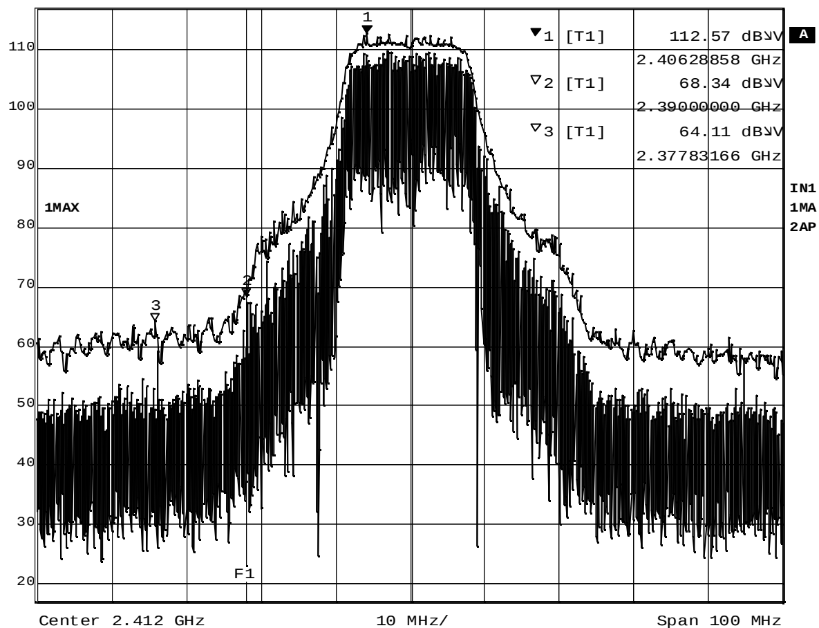
Plot 8-5 Ch.1 2412MHz TX, OFDM 18Mbps (Peak)
