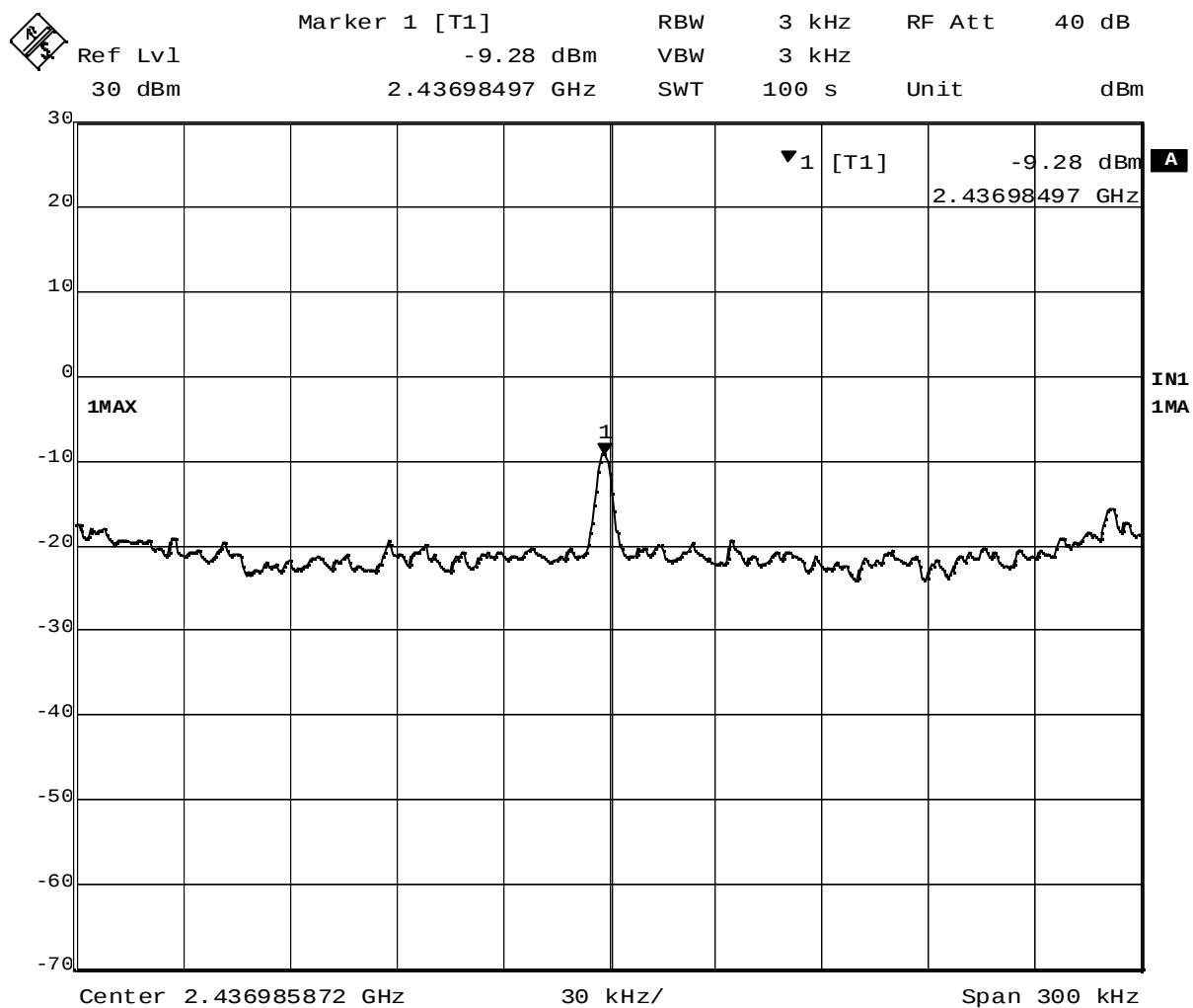
Plot 5-5. Peak Power Spectral Density of 2437MHz (OFDM, 18Mbps)
