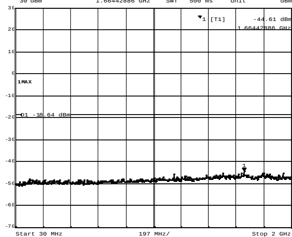
Plot 4-4. Out of band emissions around 2412MHz (OFDM, 18Mbps)
