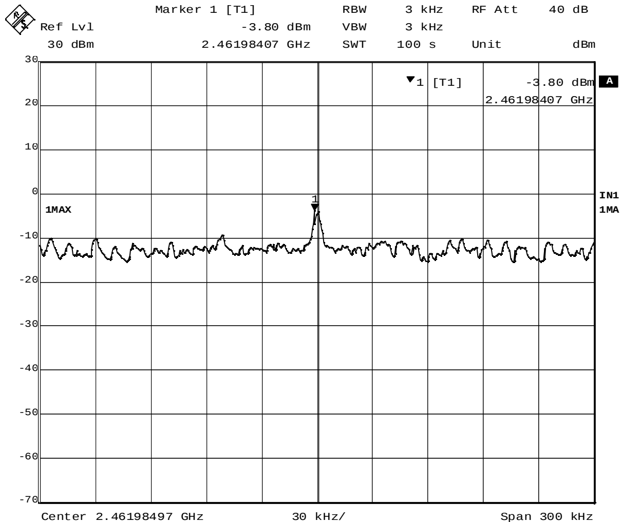
Plot 5-3. Peak Power Spectral Density of 2462MHz (DSSS, 11Mbps)
