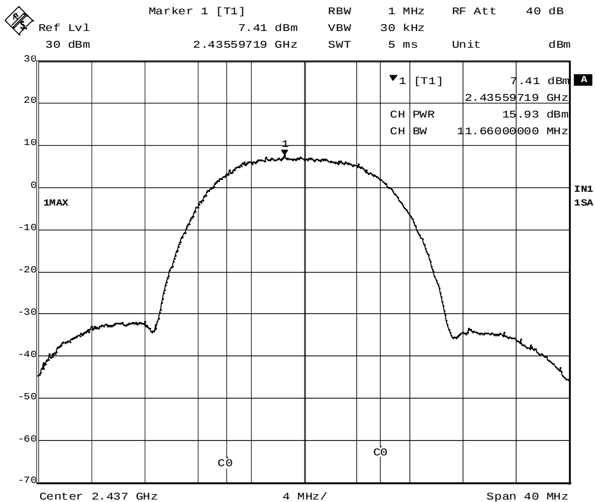
Plot 3-2. Conducted Peak Output Power of 2437MHz (DSSS, 11Mbps)
