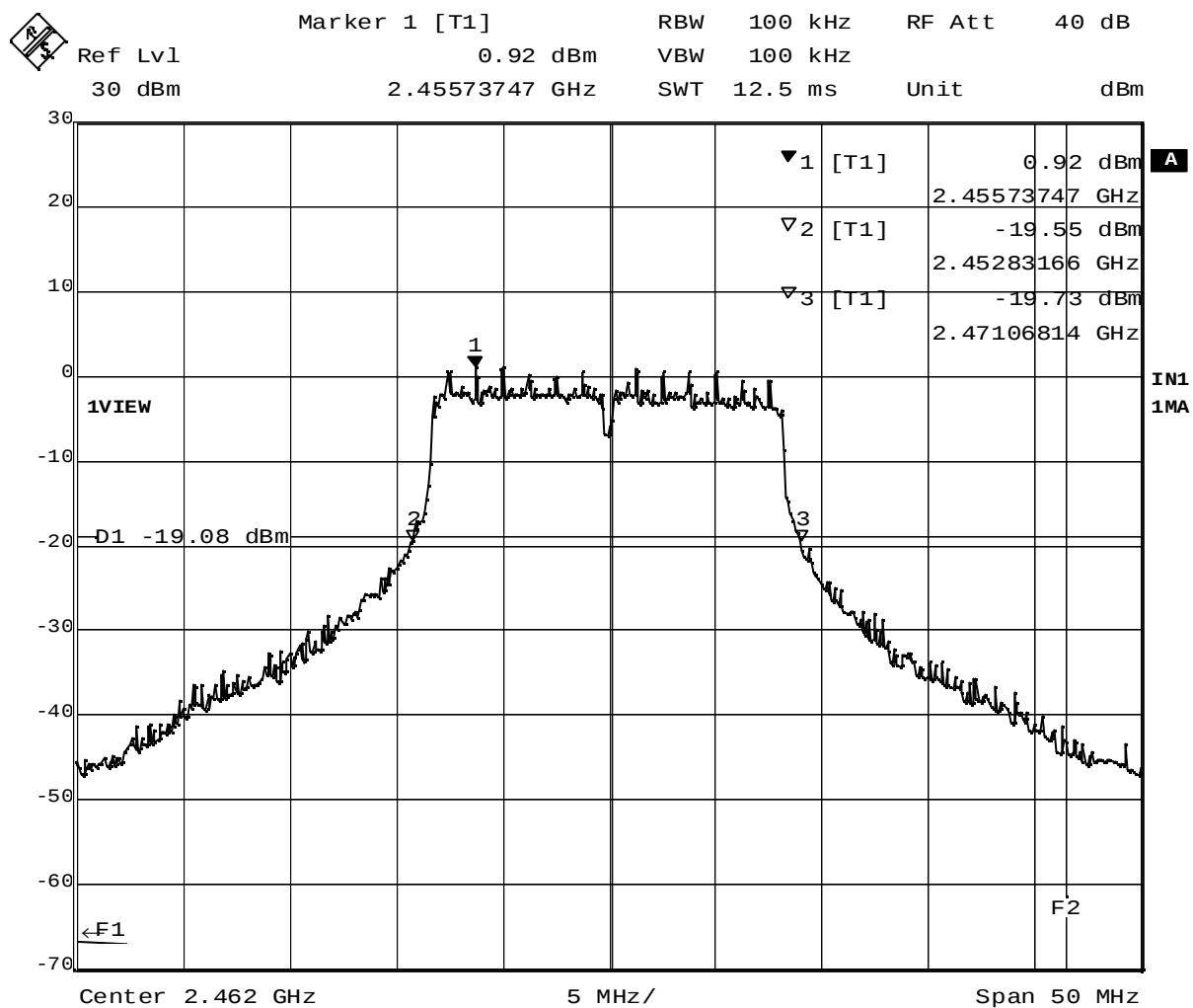
Plot 2-2. 20dB BW at 2462MHz (OFDM, 18Mbps)
