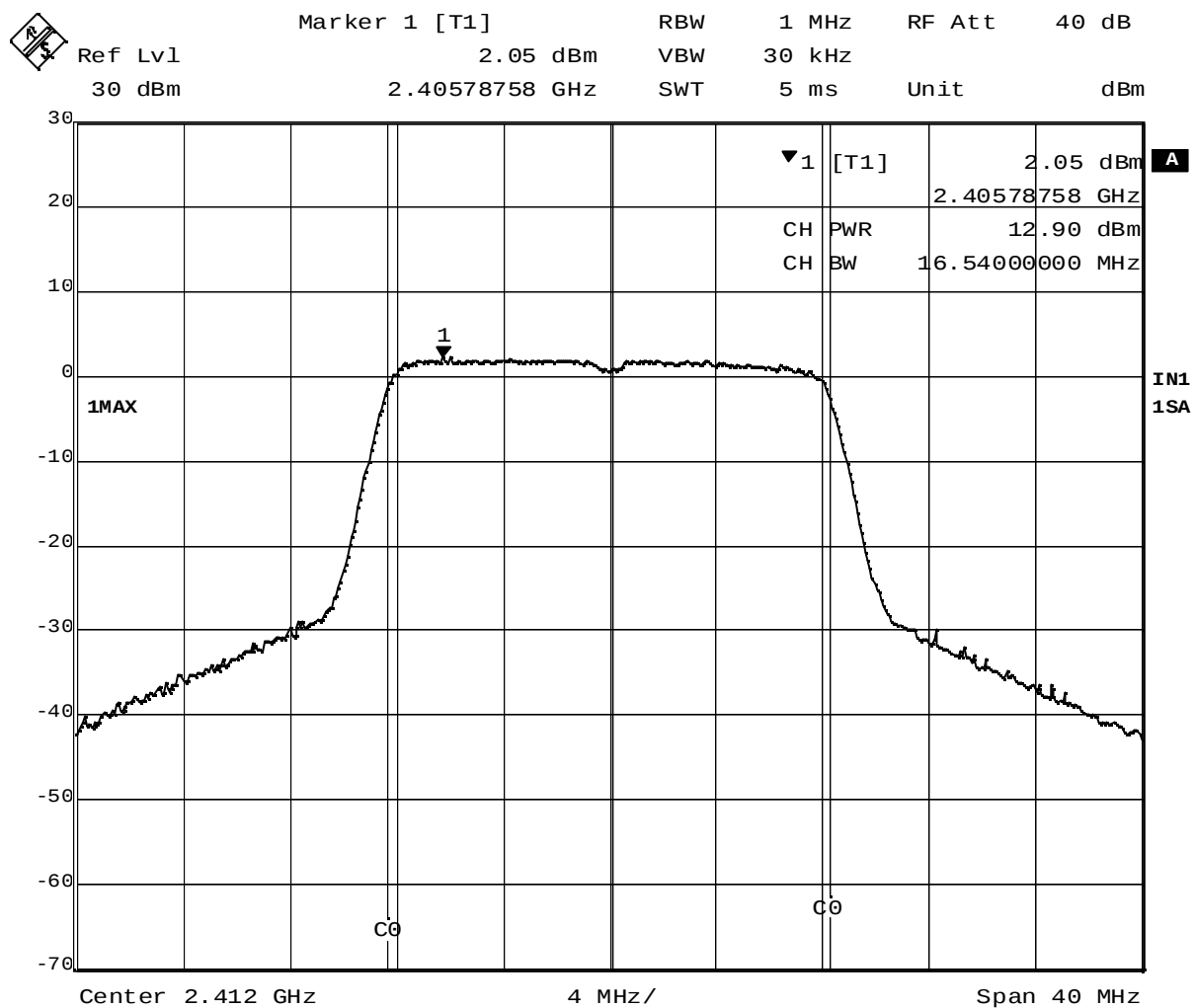
Plot 3-4. Conducted Peak Output Power of 2412MHz (OFDM, 18Mbps)
