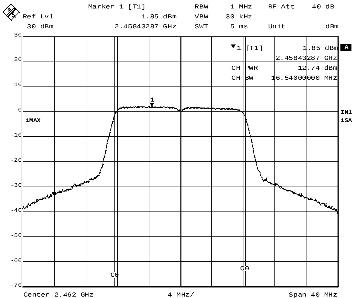
Plot 3-6. Conducted Peak Output Power of 2462MHz (OFDM, 18Mbps)
