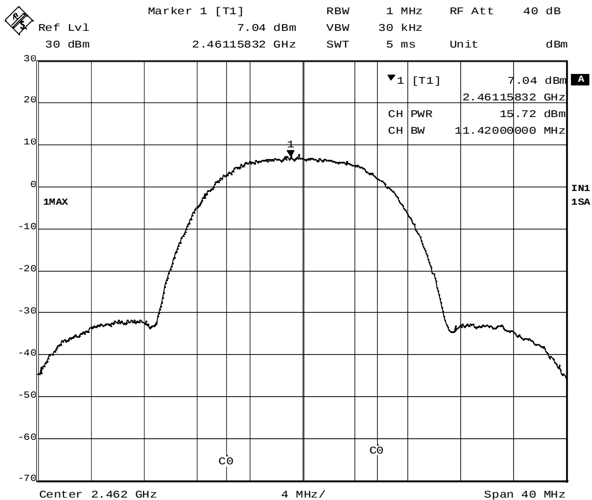
Plot 3-3. Conducted Peak Output Power of 2462MHz (DSSS, 11Mbps)
