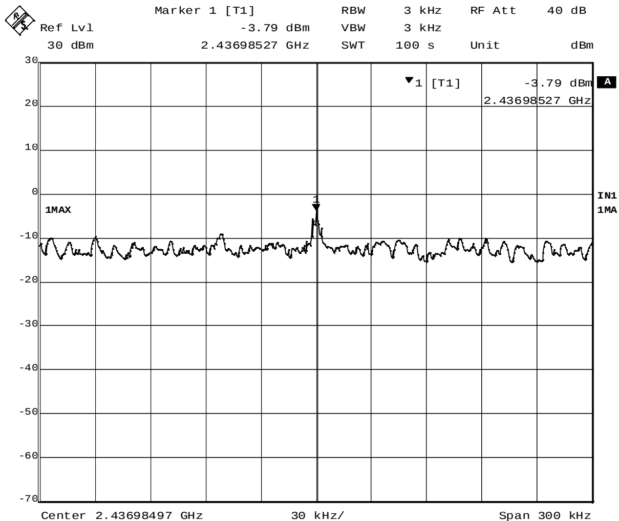
Plot 5-2. Peak Power Spectral Density of 2437MHz (DSSS, 11Mbps)
