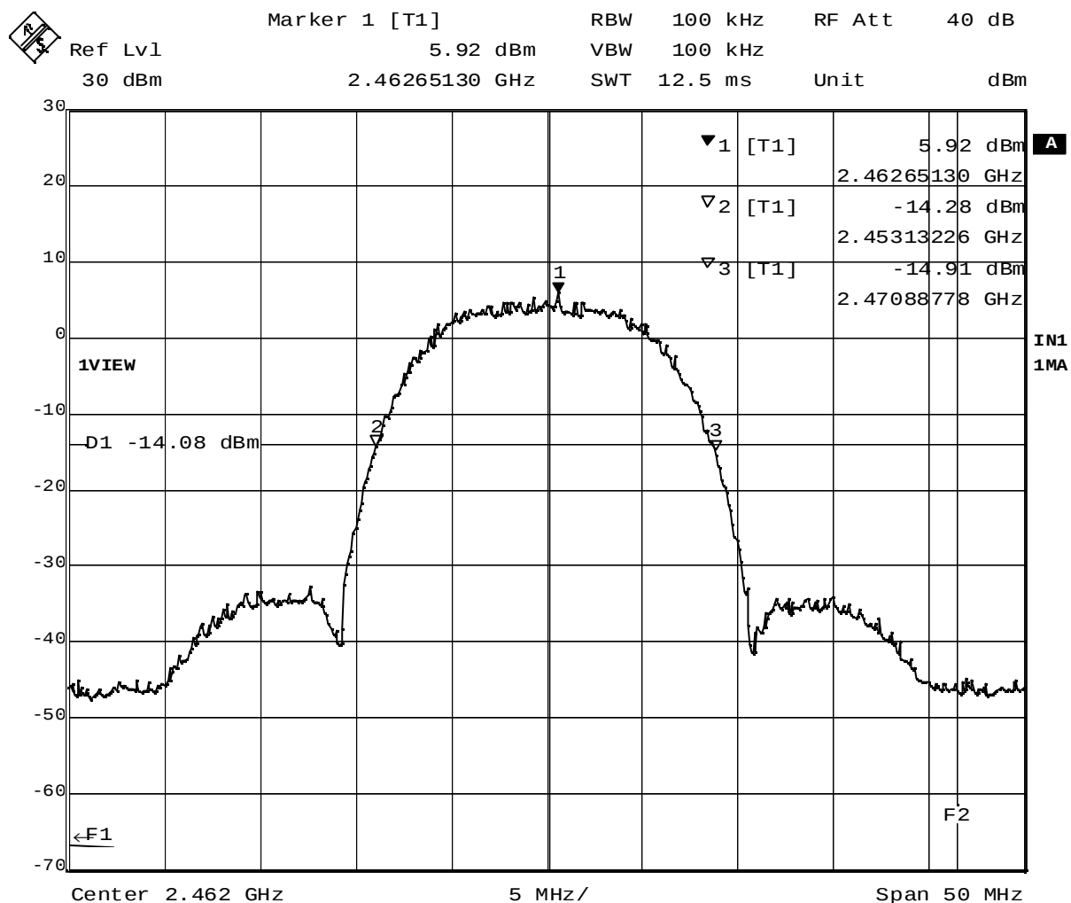
Plot 2-1. 20dB BW at 2462MHz (DSSS, 11Mbps)
