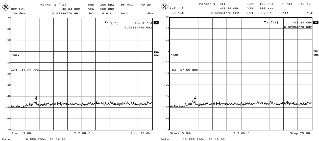
Plot 4-5. Conducted Spurious (OFDM, 18Mbps, ch. 6)
