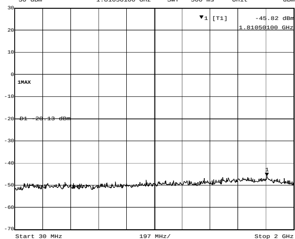
Plot 4-6. Conducted Spurious (OFDM, 18Mbps, ch. 11)
