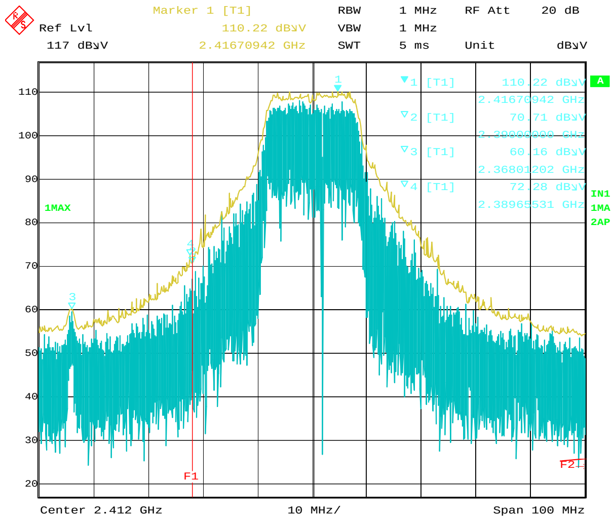
Plot 8-5 Ch.1 2412MHz TX, OFDM 18Mbps (Peak)
