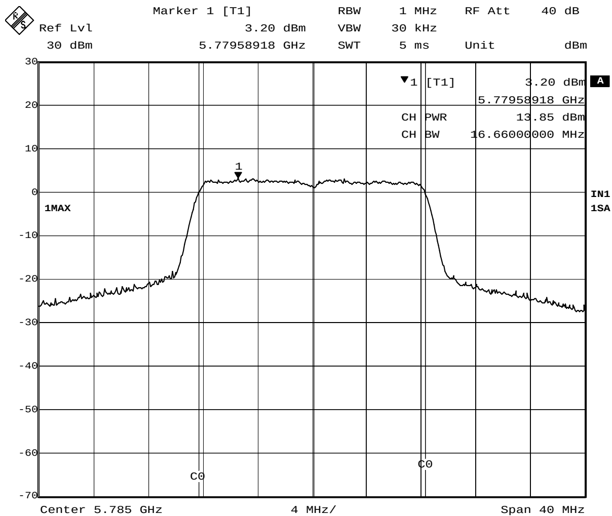
Plot 3-8. Conducted Peak Output Power of 5785MHz (OFDM, 24Mbps)
