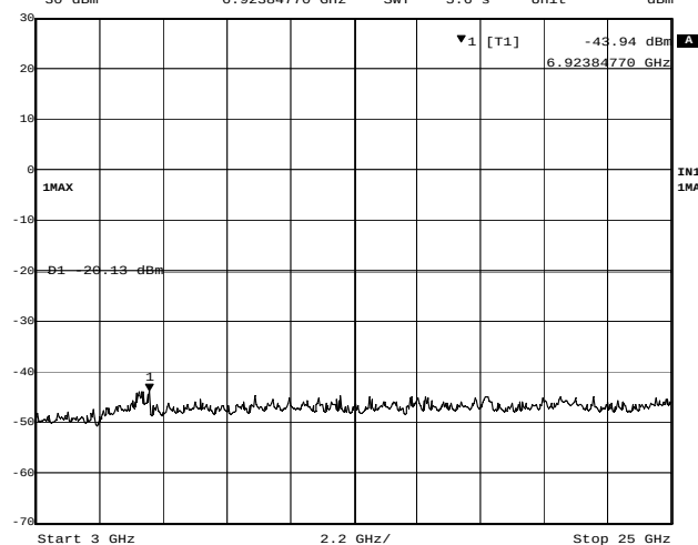
Plot 4-6. Conducted Spurious (OFDM, 18Mbps, ch. 11)
