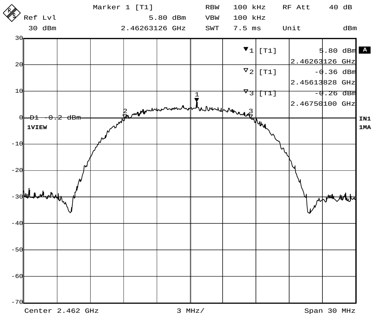
Plot 1-2. 6dB BW at 2462MHz (DSSS, 11Mbps)
