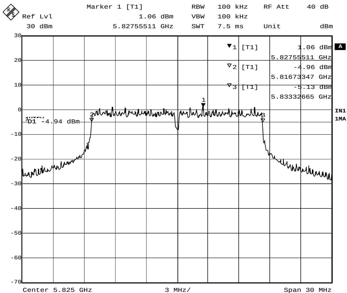
Plot 1-6. 6dB BW at 5825MHz (OFDM, 24Mbps)
