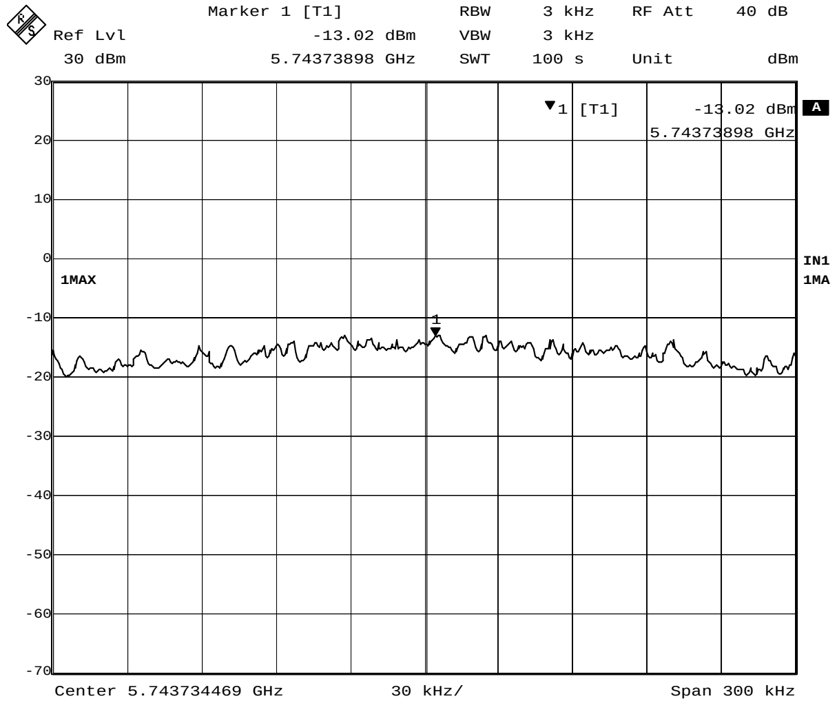
Plot 5-7. Peak Power Spectral Density of 5745MHz (OFDM, 24Mbps)
