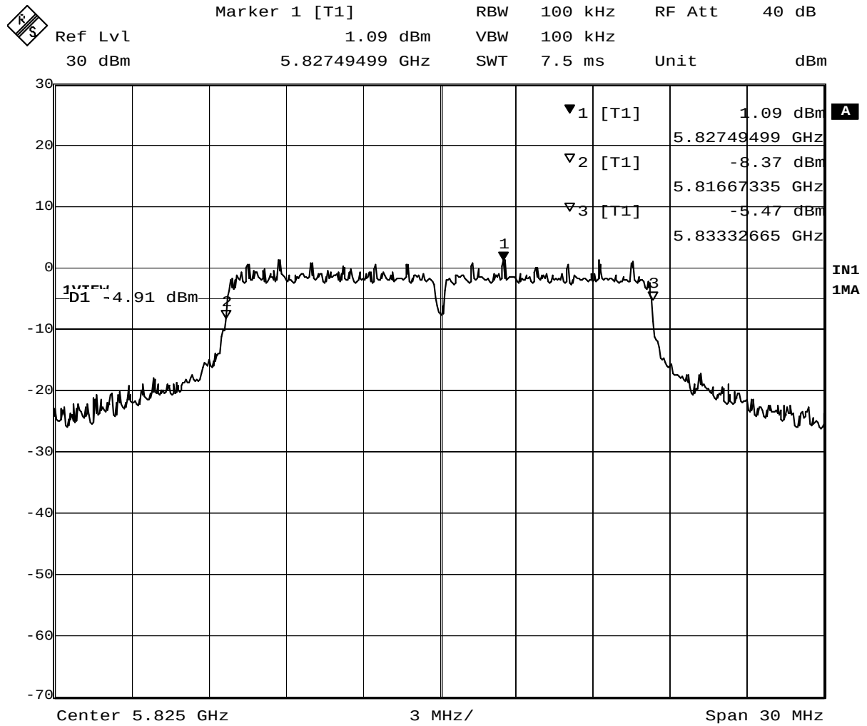
Plot 1-5. 6dB BW at 5825MHz (OFDM, 6Mbps)
