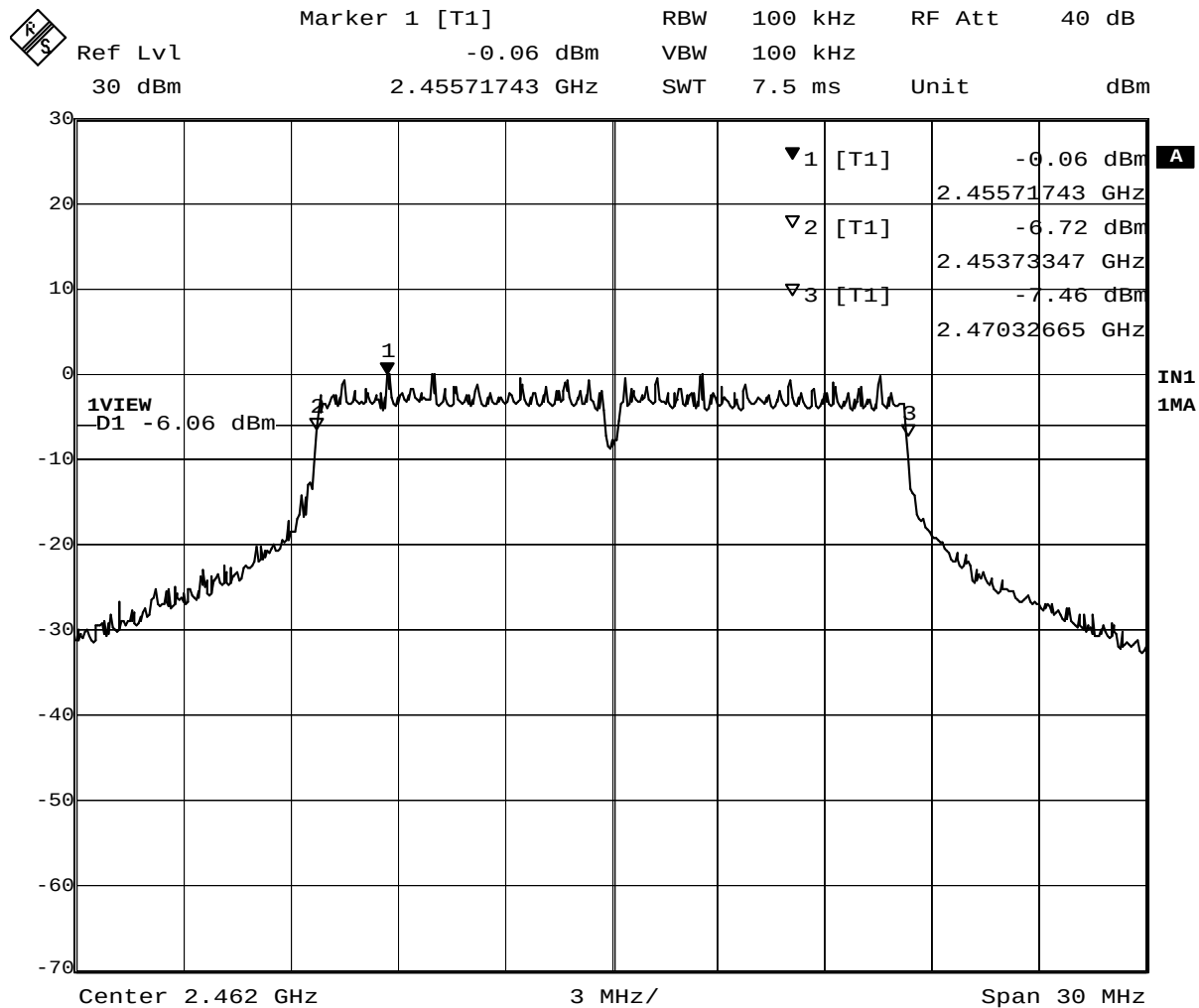
Plot 1-4. 6dB BW at 2462MHz (OFDM, 18Mbps)
