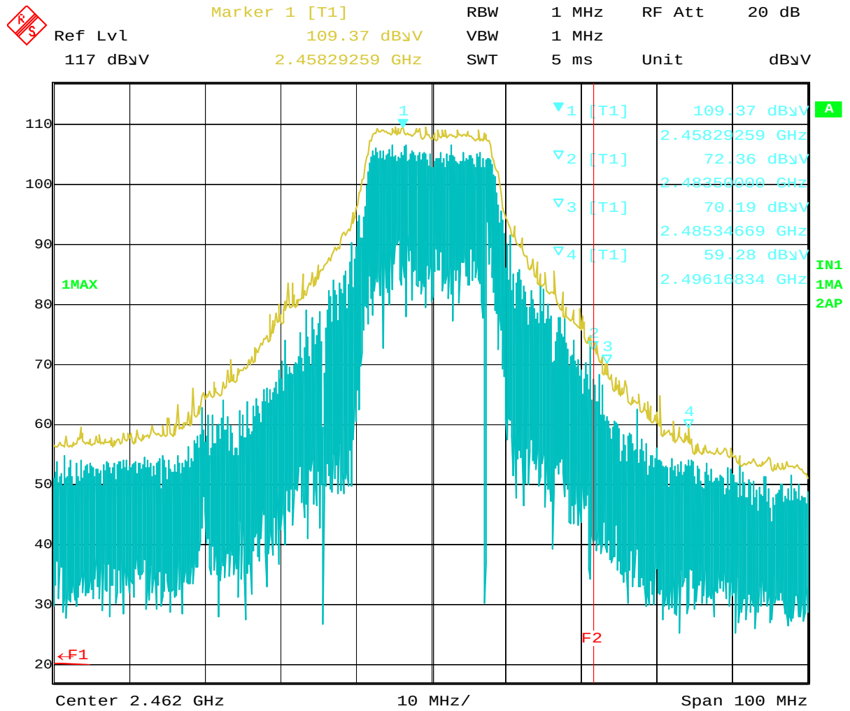
Plot 8-7 Ch.11 2462MHz TX, OFDM 18Mbps (Peak)
