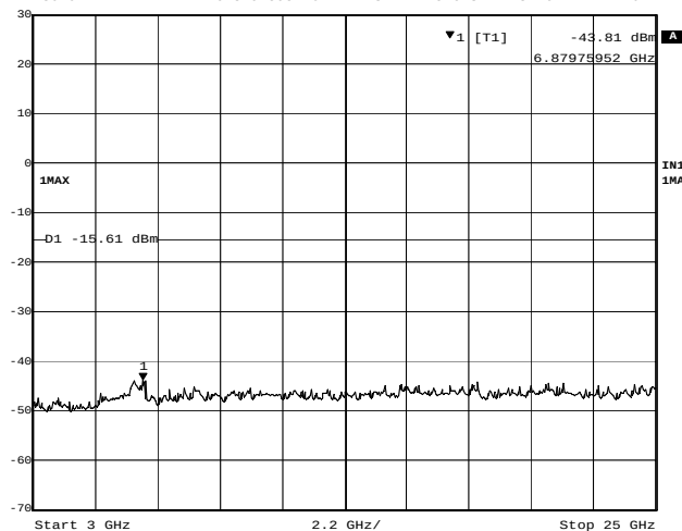
Plot 4-2. Conducted Spurious (DSSS, 11Mbps, ch. 6)
