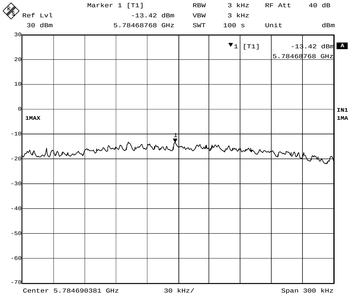
Plot 5-8. Peak Power Spectral Density of 5785MHz (OFDM, 24Mbps)
