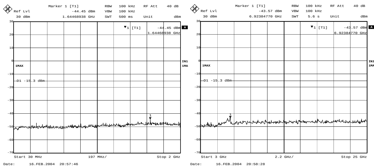
Plot 4-1. Conducted Spurious (DSSS, 11Mbps, ch.1)
