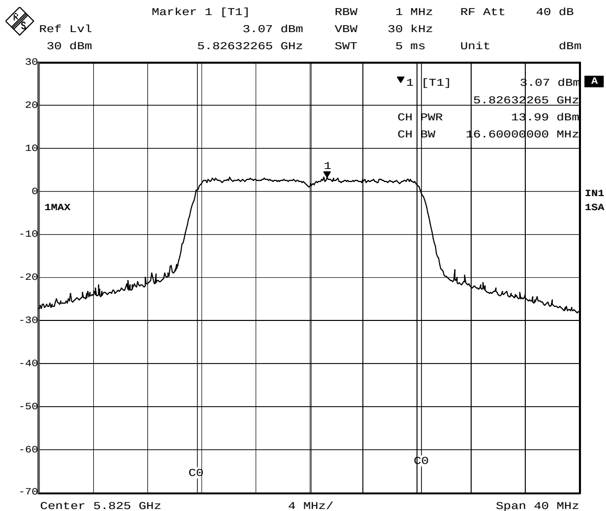
Plot 3-9. Conducted Peak Output Power of 5825MHz (OFDM, 24Mbps)
