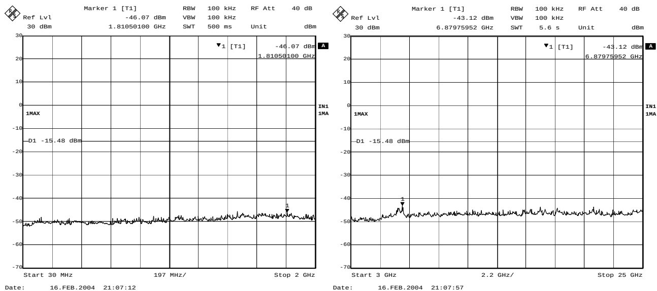
Plot 4-3. Conducted Spurious (DSSS, 11Mbps, ch. 11)
