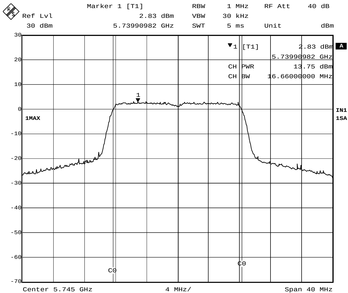
Plot 3-7. Conducted Peak Output Power of 5745MHz (OFDM, 24Mbps)
