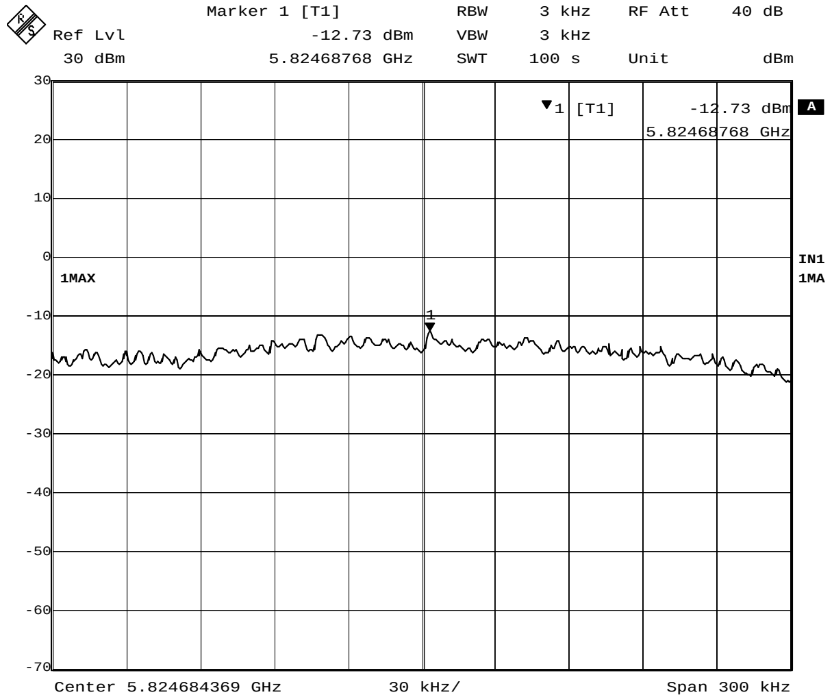
Plot 5-9. Peak Power Spectral Density of 5825MHz (OFDM, 24Mbps)
