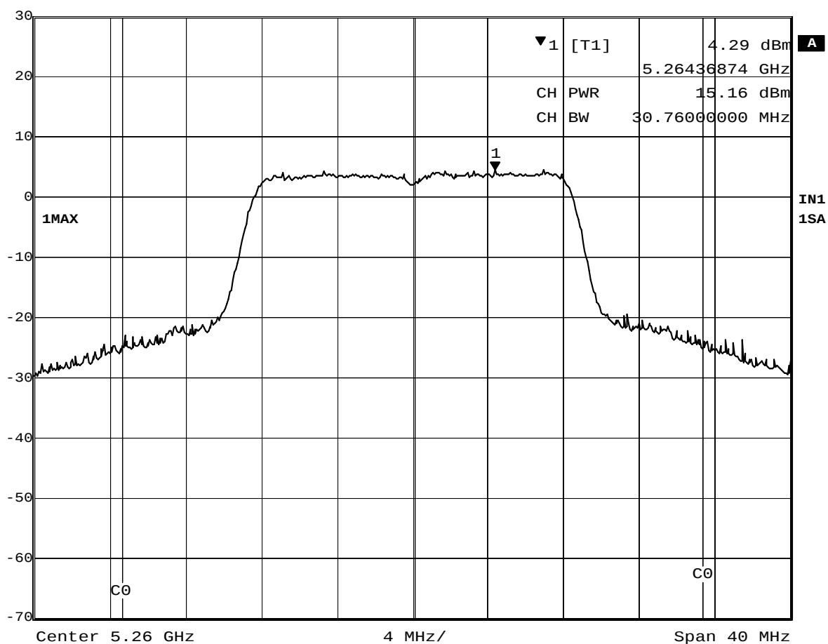
Plot 2-2 Conducted Peak Power at 5260MHz
