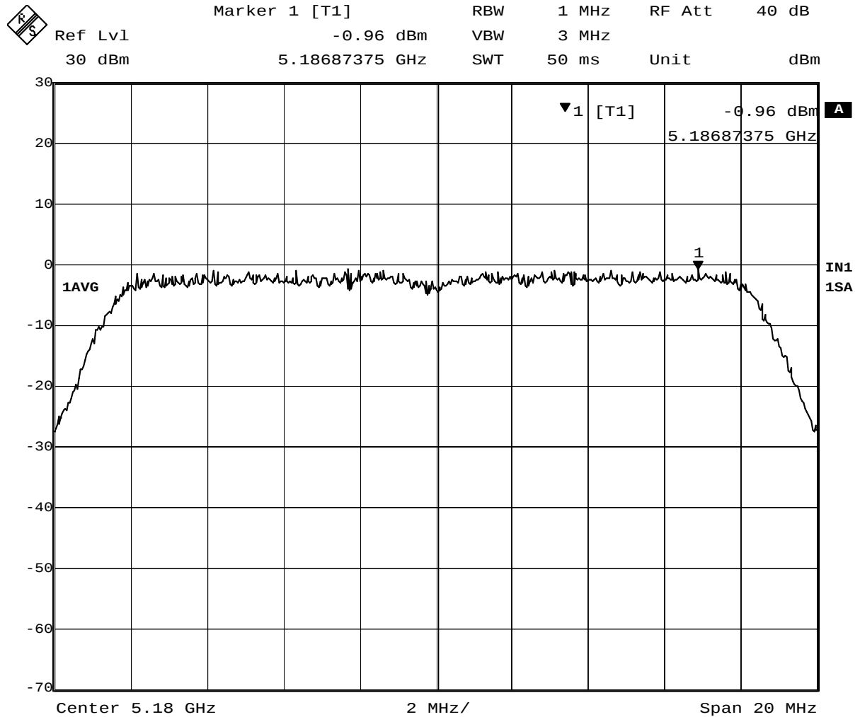
Plot 3-1 Peak Power Spectral Density at 5180MHz
