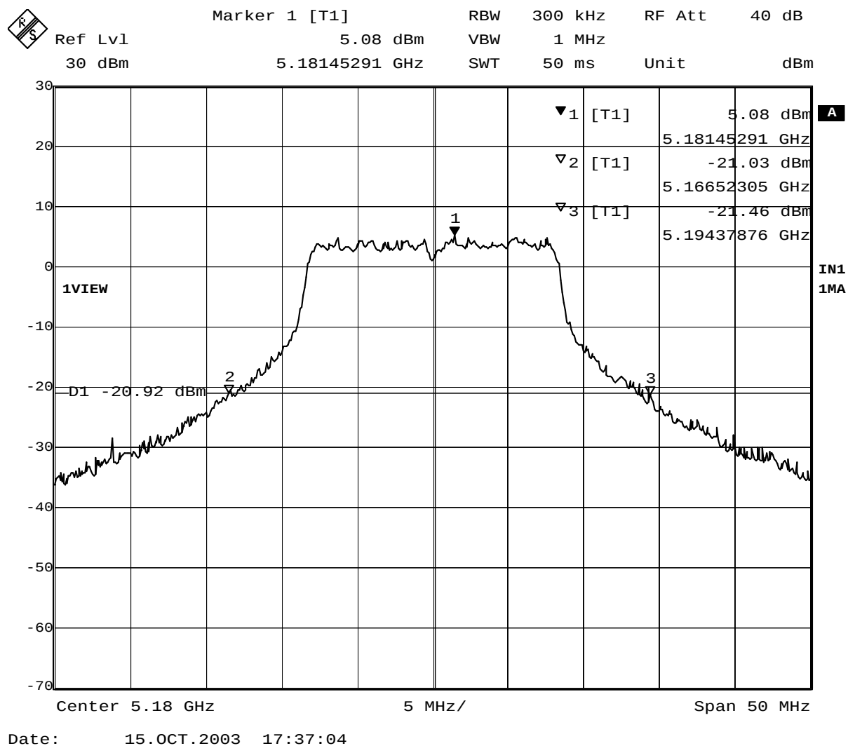
Plot 1-1. 26dB BW at 5180MHz
