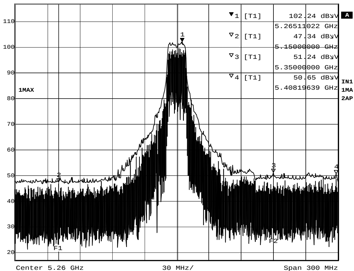
Plot 7-2-1 5260MHz TX mode (Peak)
