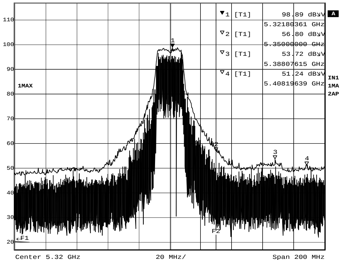
Plot 7-3-1 5320MHz TX mode (Peak)
