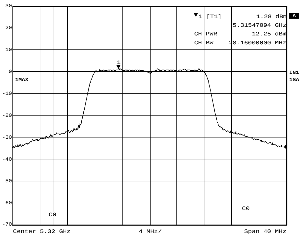
Plot 2-3 Conducted Peak Power at 5320MHz
