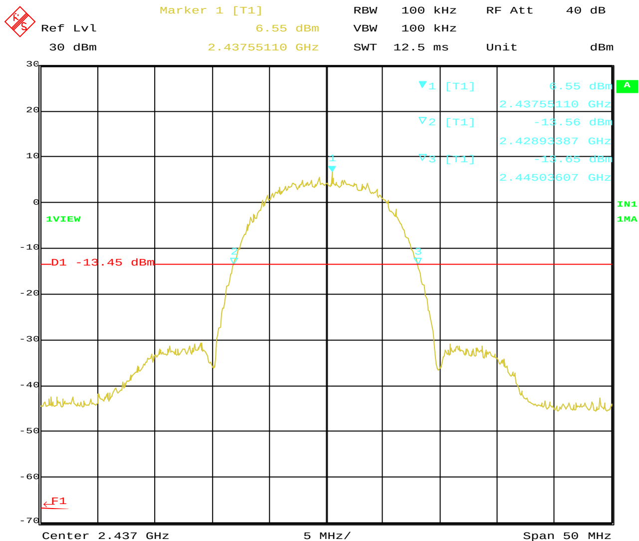
Plot 2-2. 20dB BW at 2437MHz
