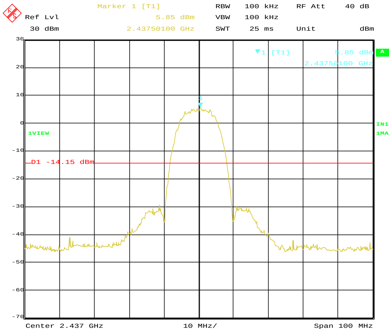
Plot 2-8. Out of band emissions around 2437MHz
