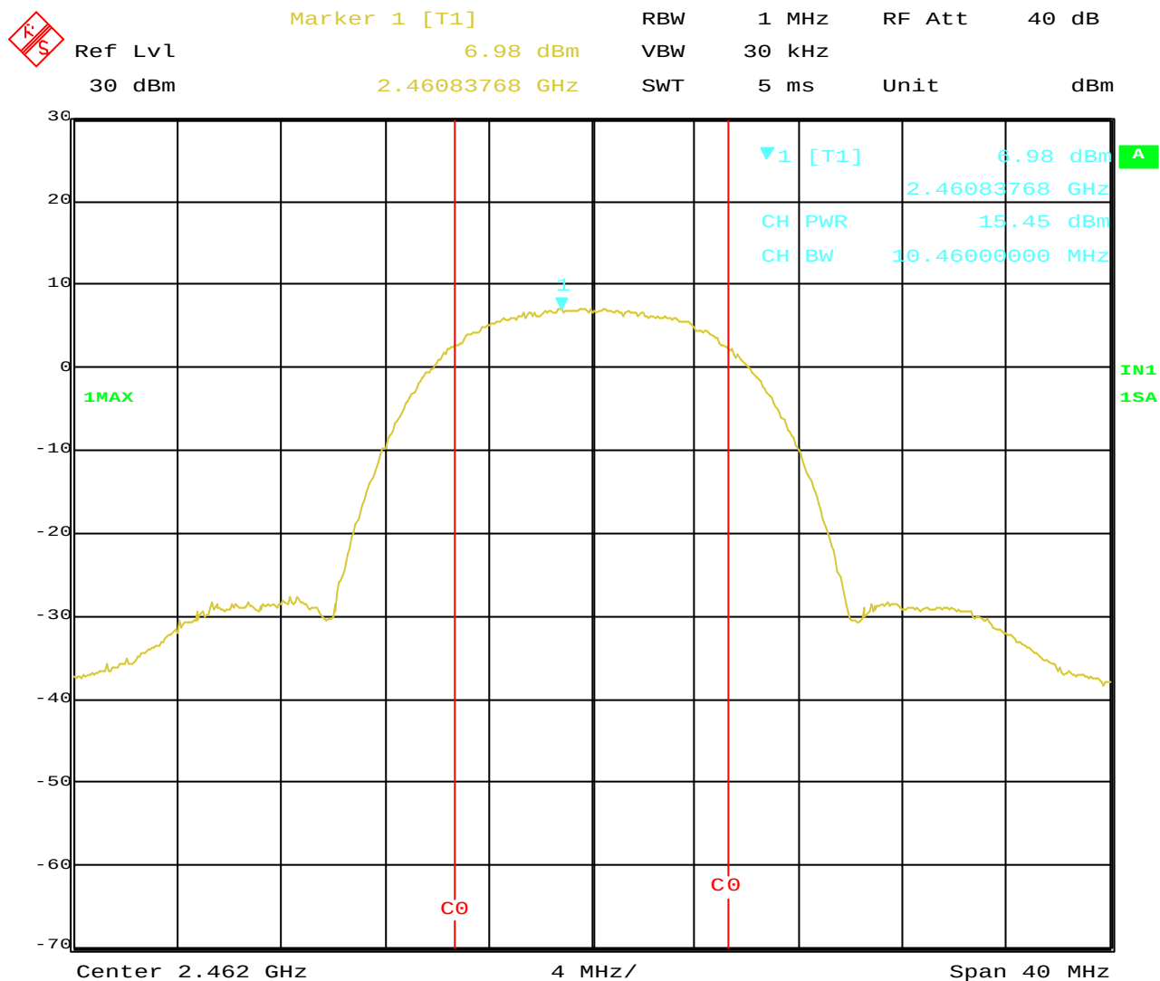
Plot 3-3. Conducted Peak Output Power of 2462MHz
