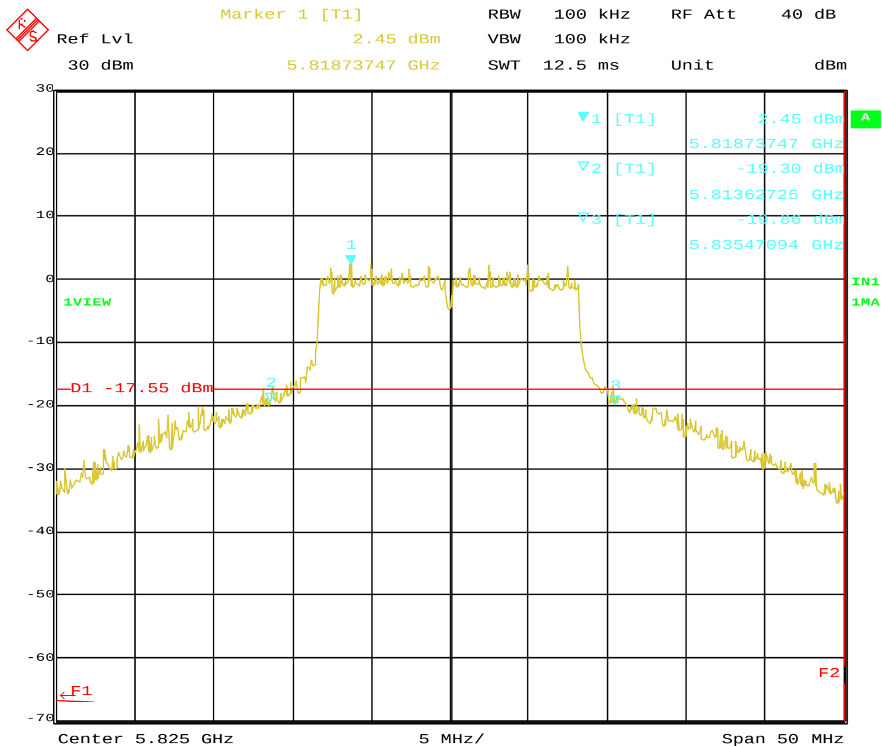
Plot 2-6. 20dB BW at 5825MHz
