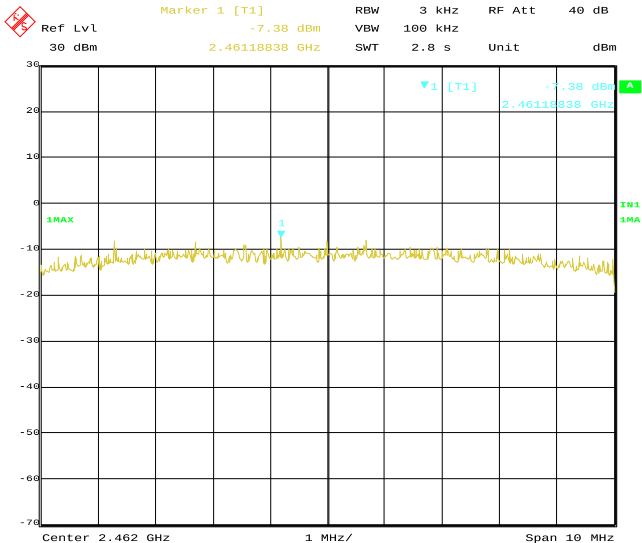
Plot 4-3. Peak Power Spectral Density of 2462MHz
