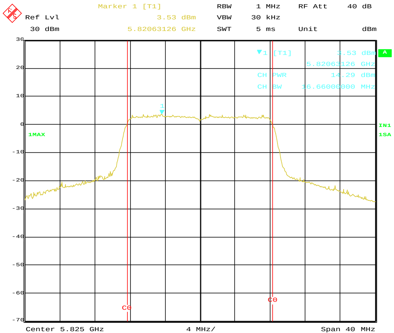
Plot 3-6. Conducted Peak Output Power of 5825MHz
