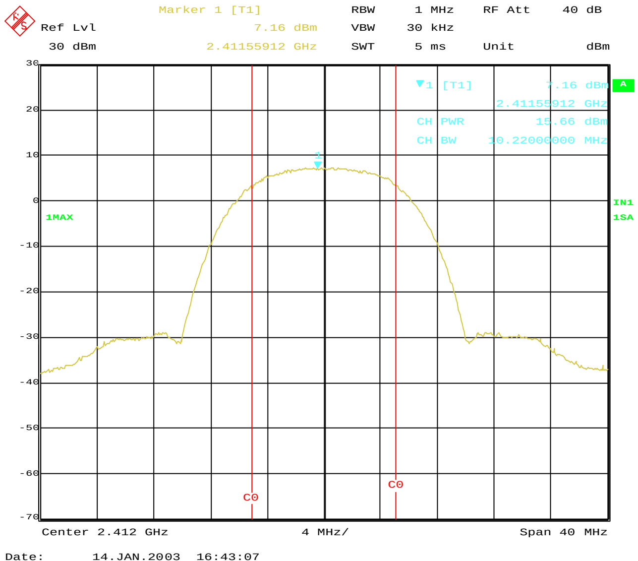
Plot 3-1. Conducted Peak Output Power of 2412MHz
