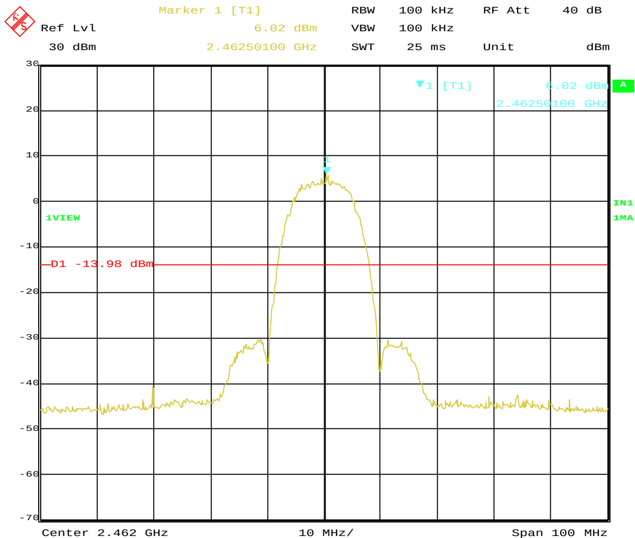
Plot 2-9. Out of band emissions around 2462MHz
