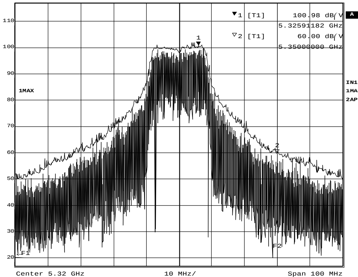
Plot 7-3-1 5320MHz TX mode (Peak)
