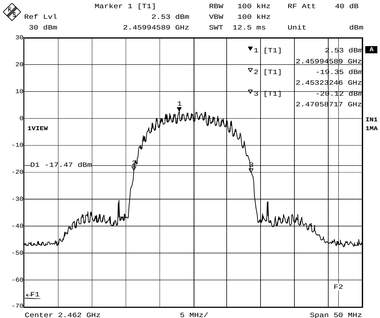
Plot 2-1. 20dB BW at 2462MHz (11Mbps)
