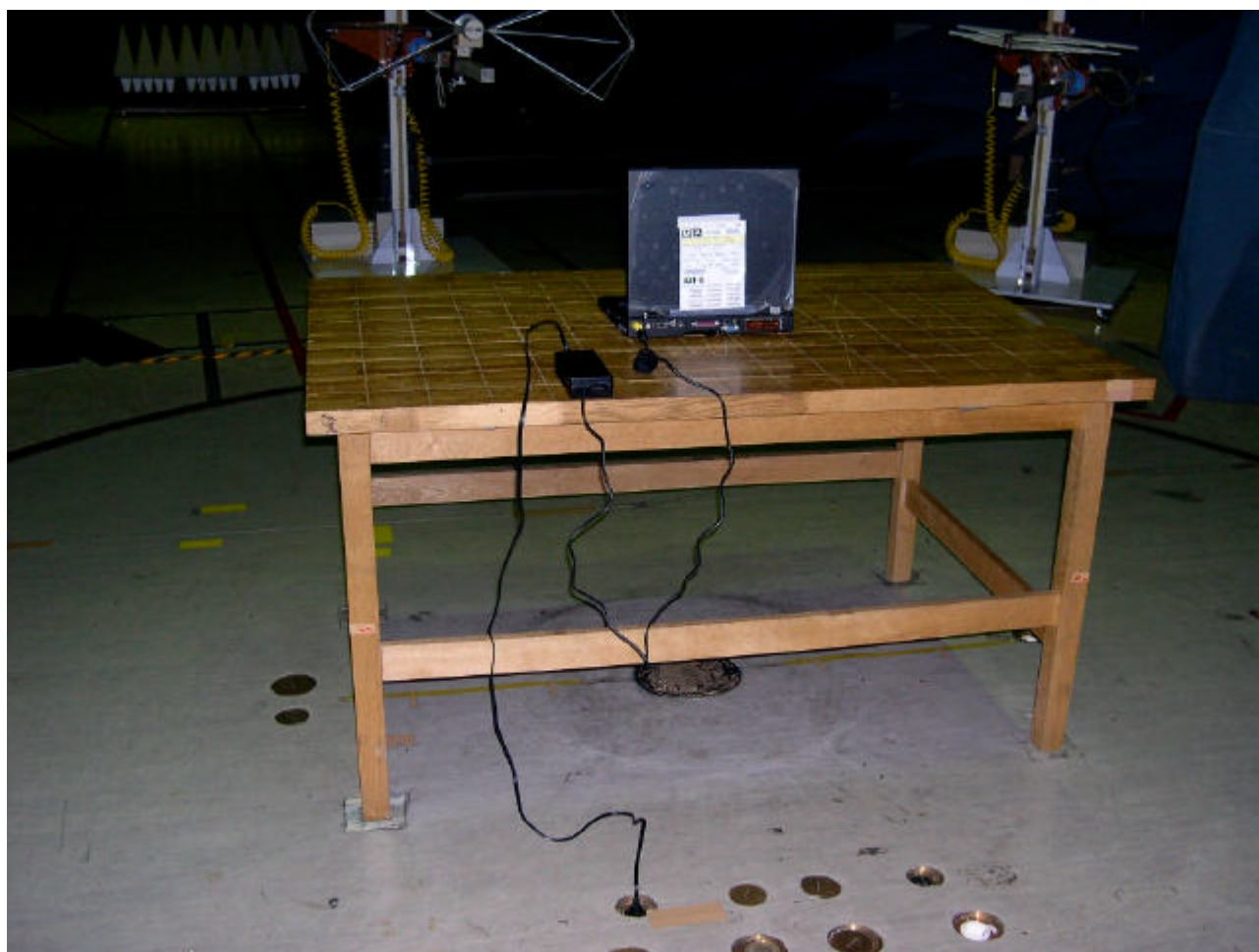
EMI-Radiation, Rear view
