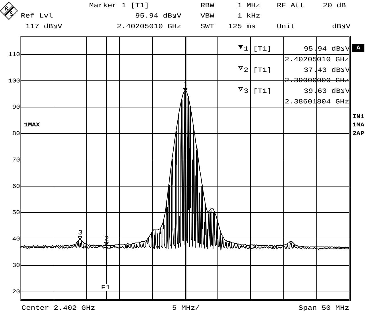
Plot 11-2-2 Ch.1 2402MHz TX (Average)
