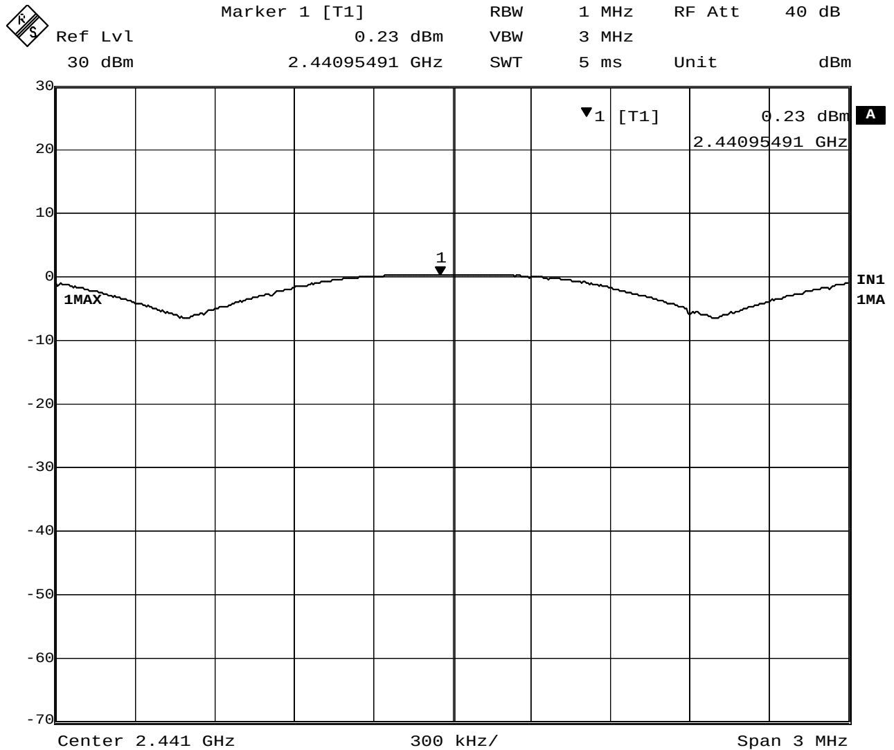
Plot 5-5. Peak Output Power (Paging)
