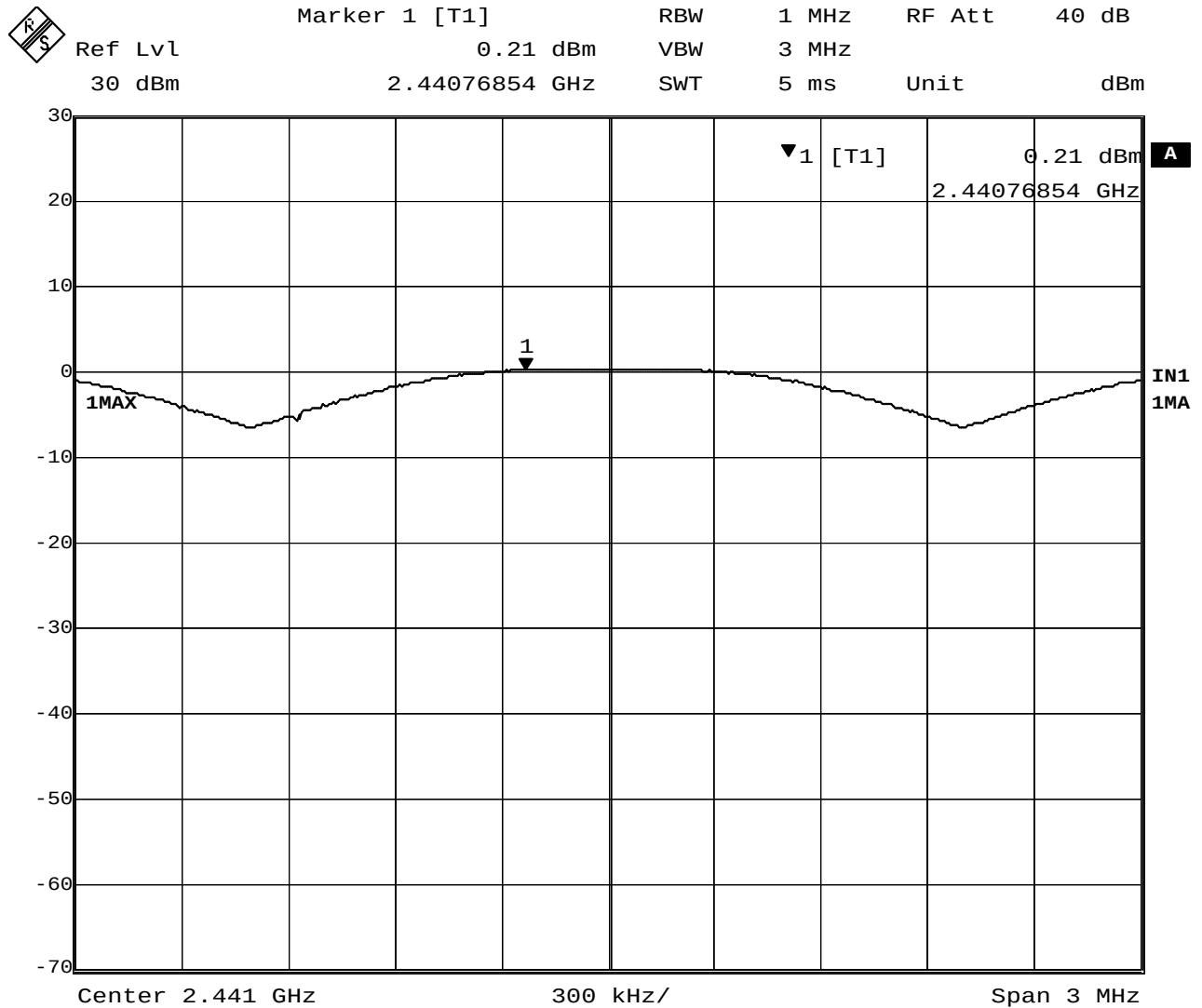
Plot 5-4. Peak Output Power (Inquiry)
