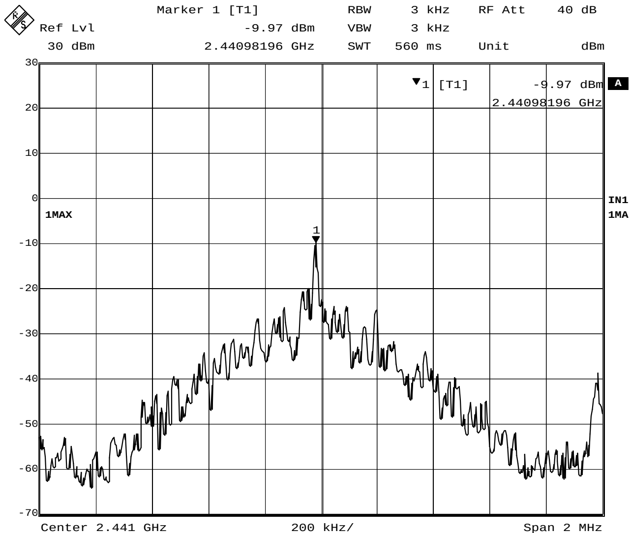
Plot 8-1. Transmitter Power Spectral Density (Inquiry)
