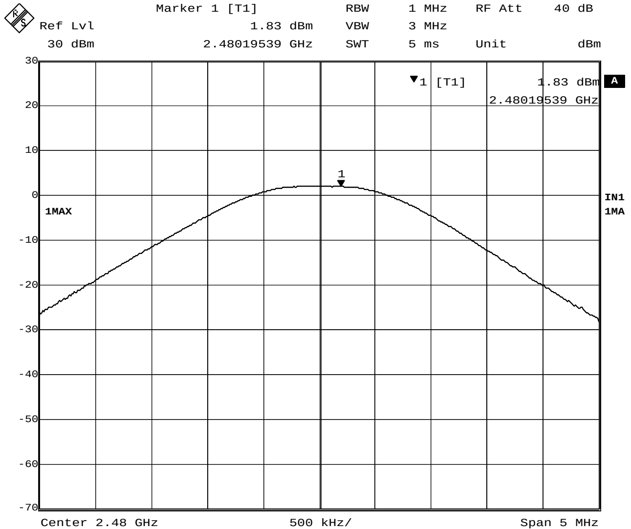
Plot 5-3. Peak Output Power (TX on 2480MHz)
