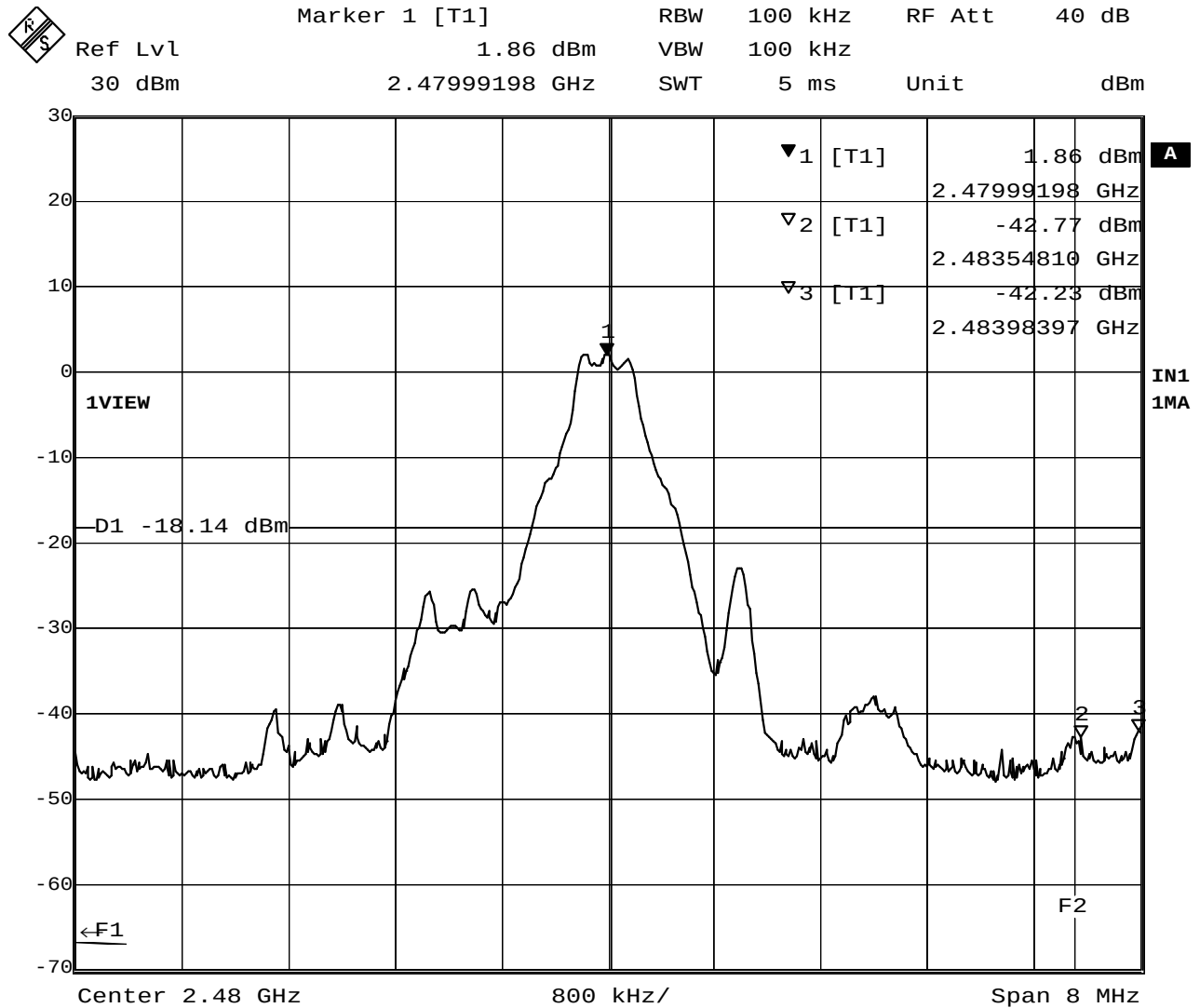
Plot 6-2. Band-edge (TX on 2480MHz)
