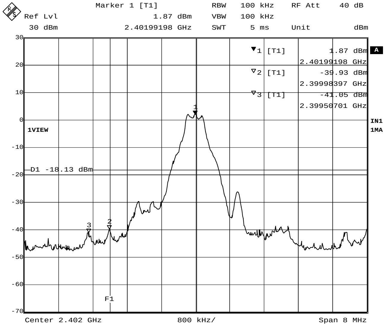
Plot 6-1. Band-edge (TX on 2402MHz)
