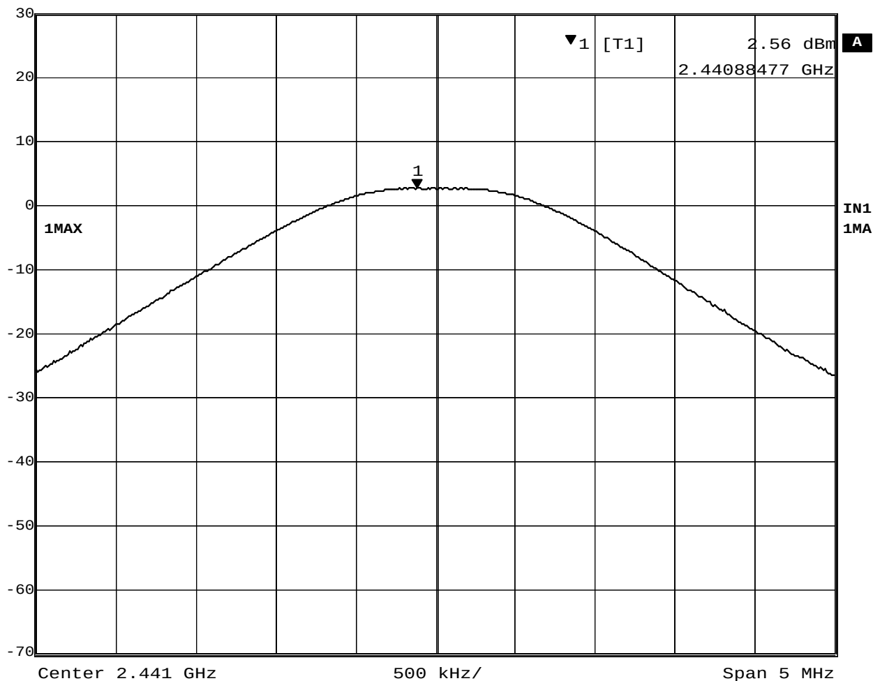
Plot 5-2. Peak Output Power (TX on 2441MHz)
