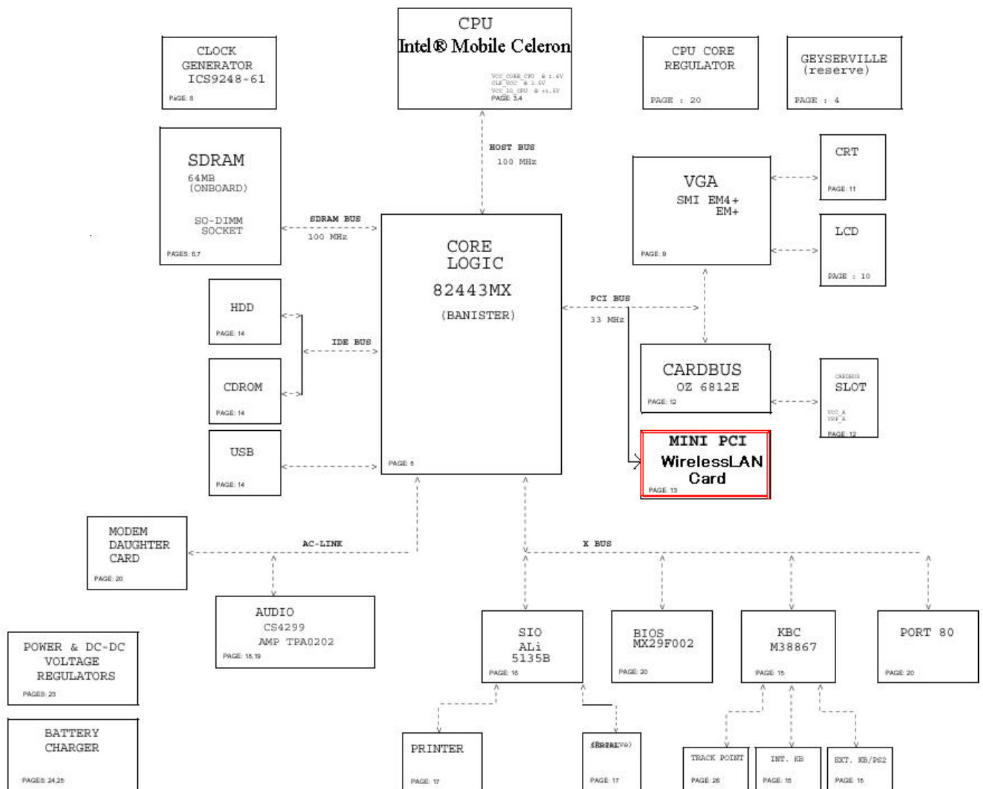
Figure 14 Block diagram of ThinkPad i 1300 and ThinkPad 130
