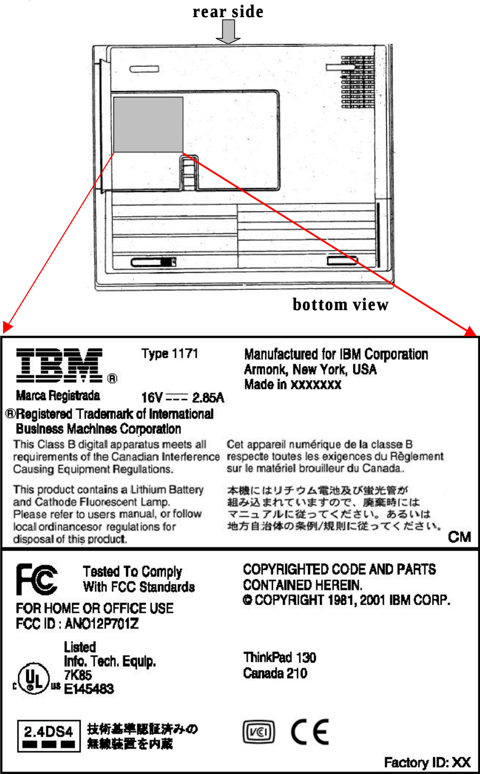
Figure 3: Labeling of ThinkPad 130
