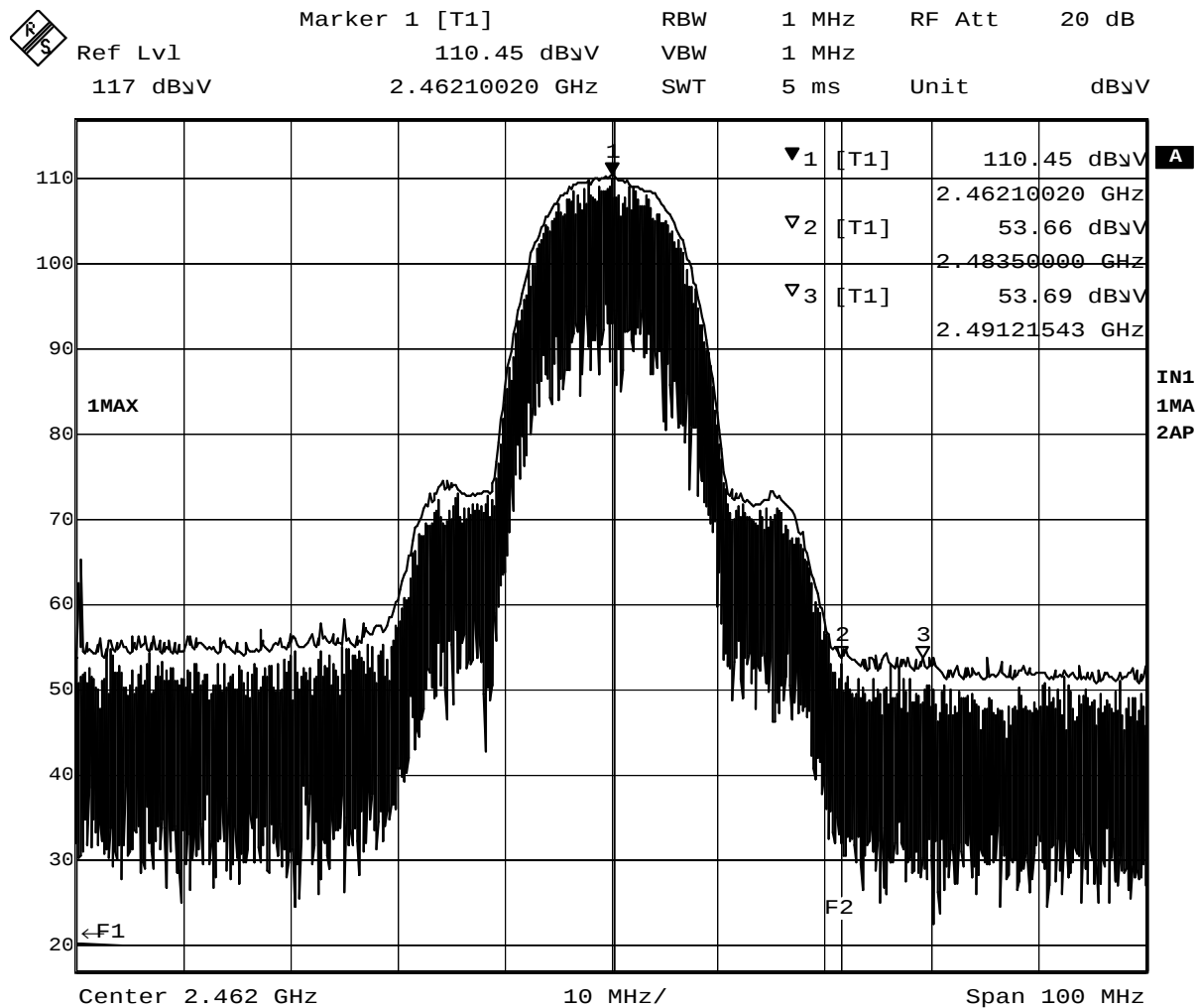
Plot 8-3 Ch.11 2462MHz TX, DSSS 11Mbps (Peak)
