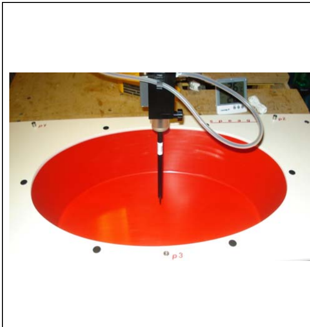
DASY4 SAR System with ELI Planar Phantom
