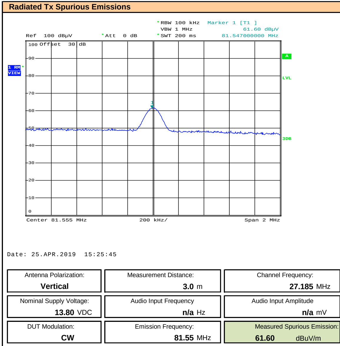
Plot 11.13 – Radiated Spurious Emissions OATS, 3 rd Harmonic, Vertical
