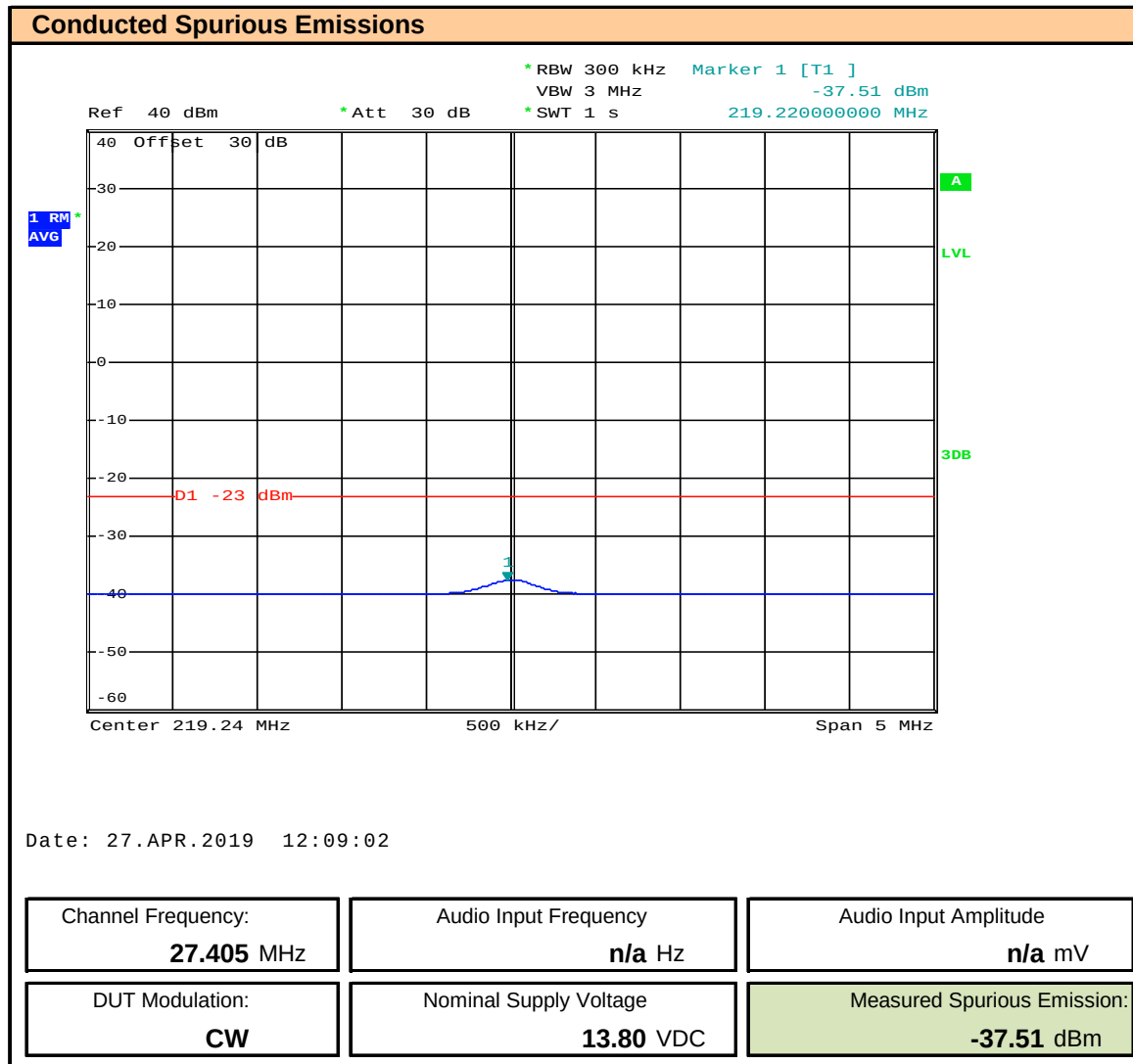
Plot 10.9 – Conducted Out of Band Emissions, Channel 40, 8th Harmonic
