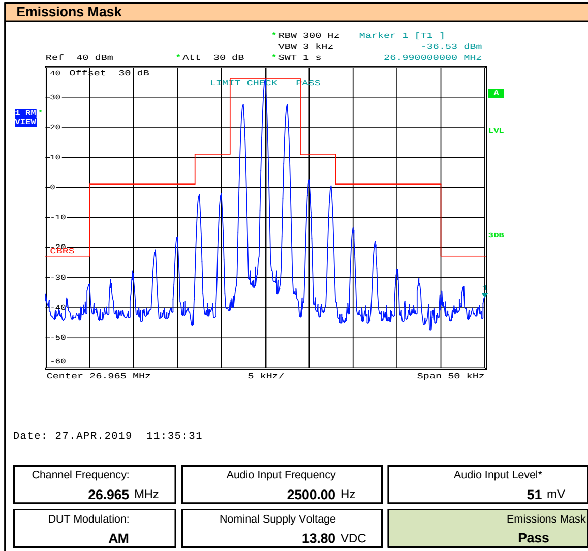
Plot 9.4 – Emissions Mask Channel 1
