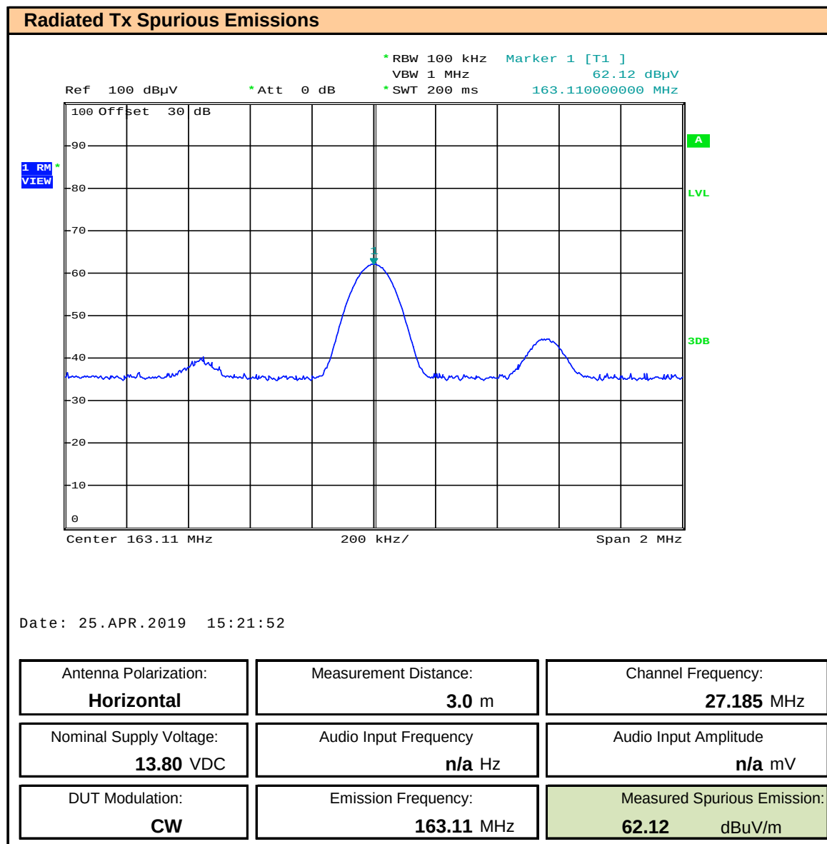
Plot 11.7 – Radiated Spurious Emissions OATS, 6 th Harmonic, Horizontal
