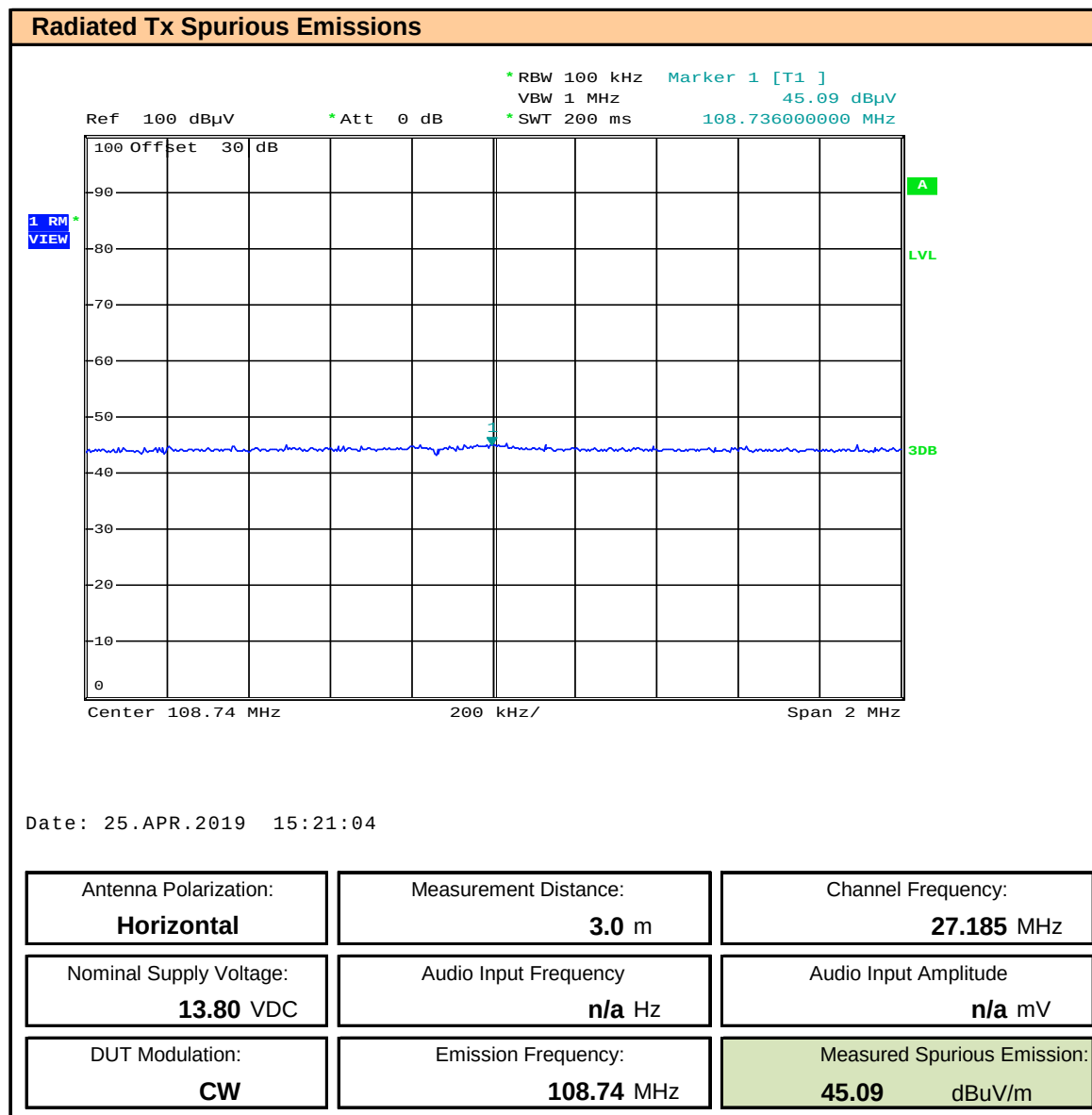
Plot 11.5 – Radiated Spurious Emissions OATS, 4 th Harmonic, Horizontal
