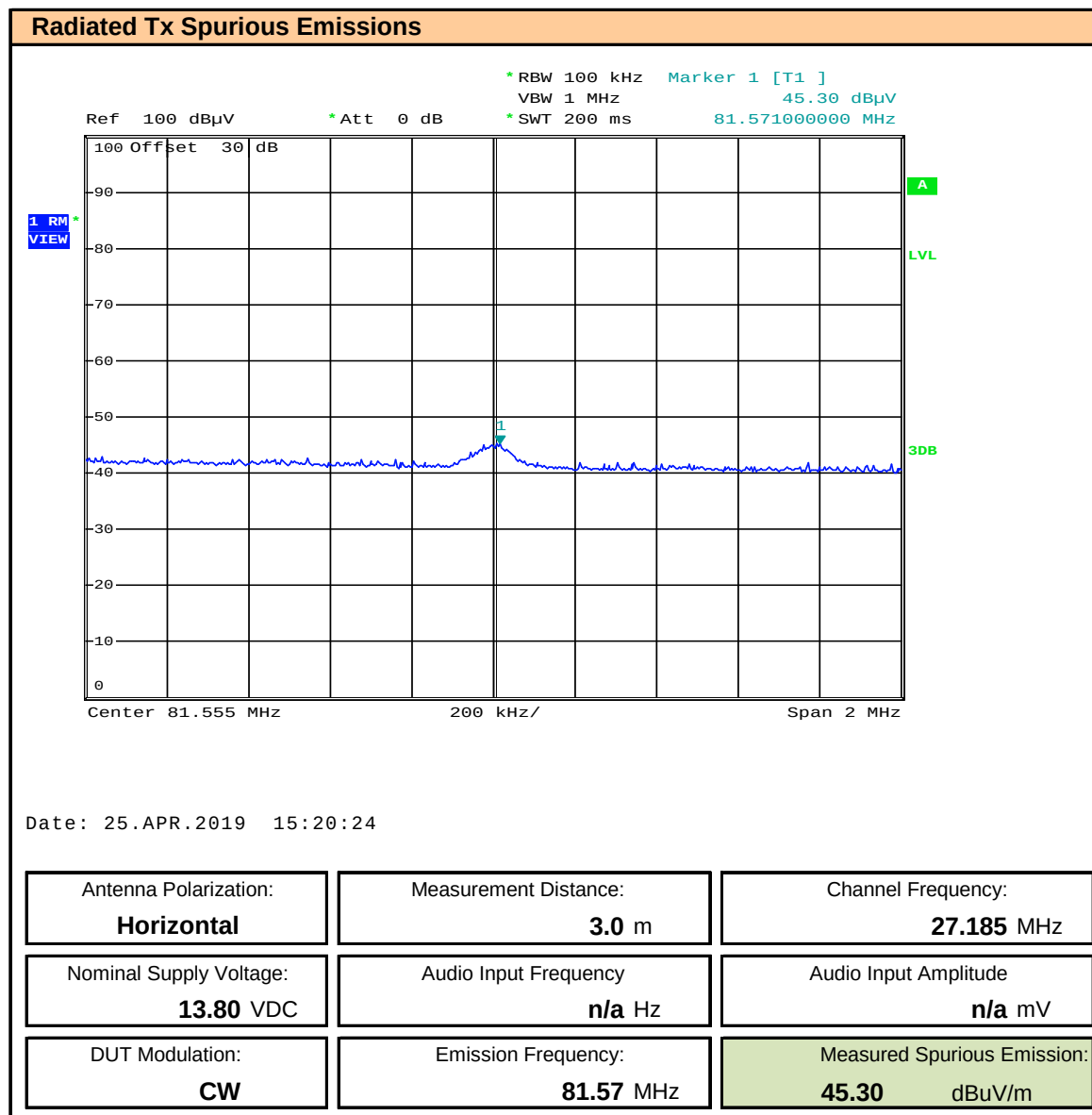
Plot 11.4 – Radiated Spurious Emissions OATS, 3 rd Harmonic, Horizontal
