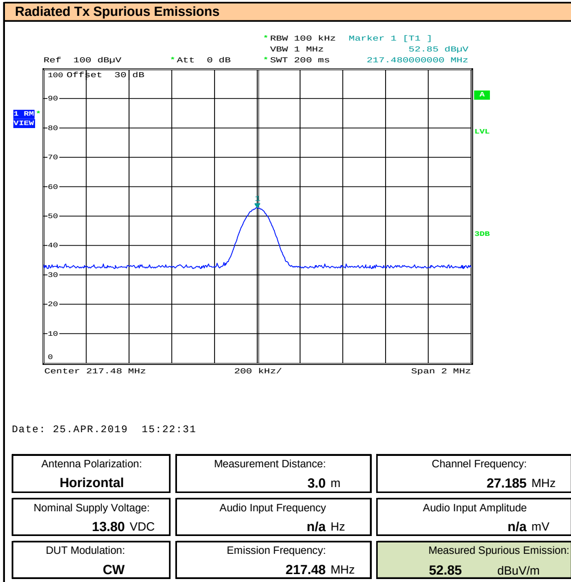
Plot 11.9 – Radiated Spurious Emissions OATS, 8 th Harmonic, Horizontal
