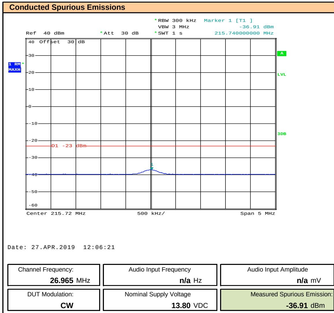
Plot 10.3 – Conducted Out of Band Emissions, Channel 1, 8th Harmonic
