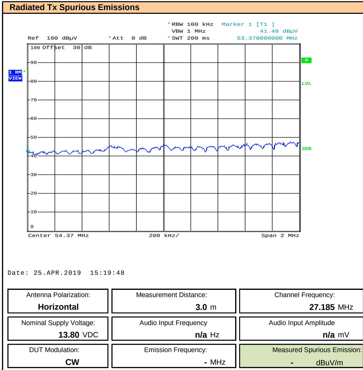
Plot 11.3 – Radiated Spurious Emissions OATS, 2 nd Harmonic, Horizontal
