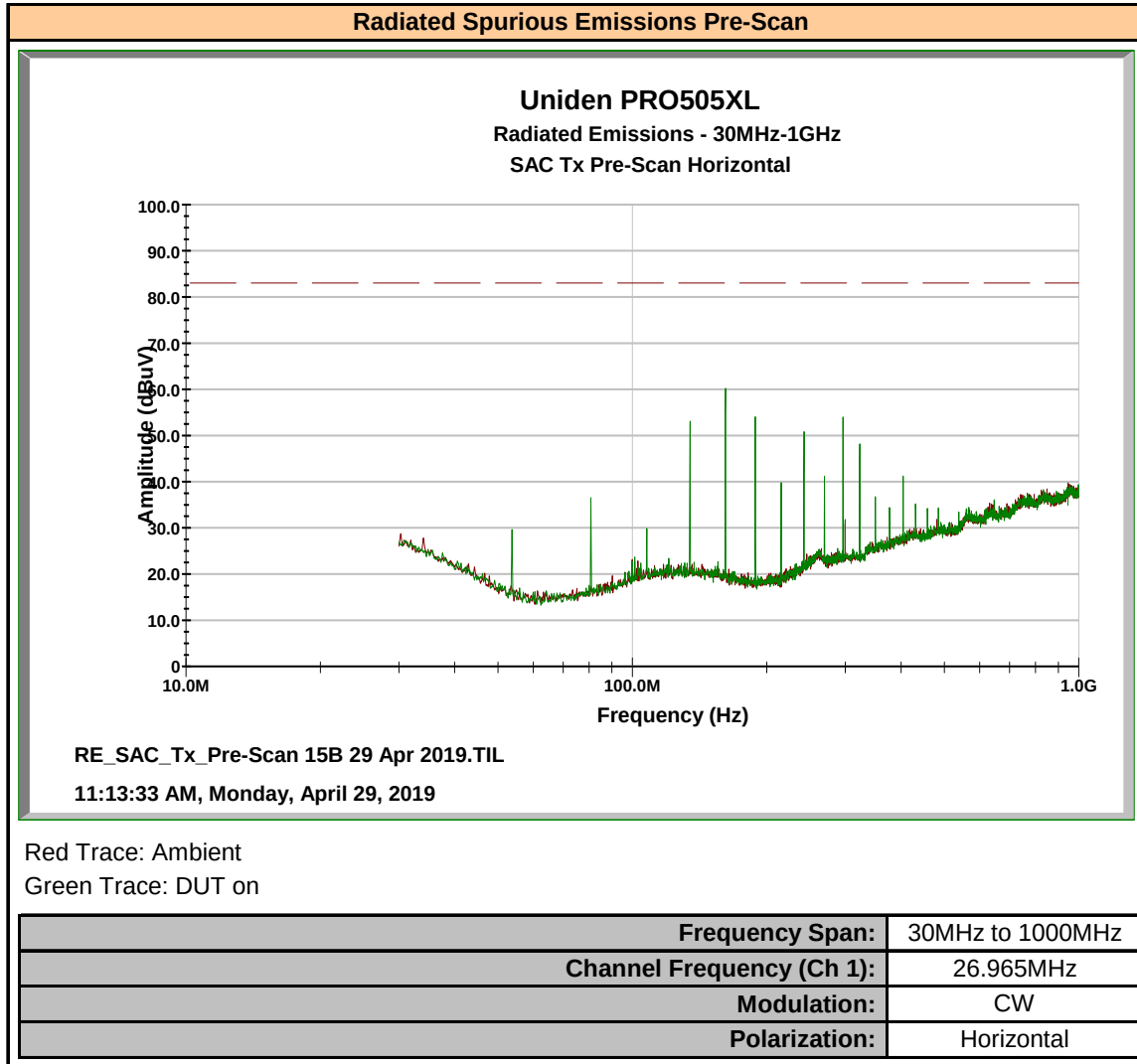
Plot 11.1 – Radiated Spurious Emissions Pre-Scan, 30MHz – 1000MHz, Horizontal
