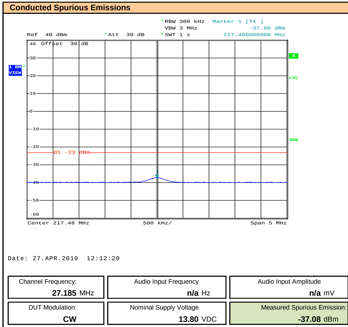
Plot 10.6 – Conducted Out of Band Emissions, Channel 19, 8th Harmonic
