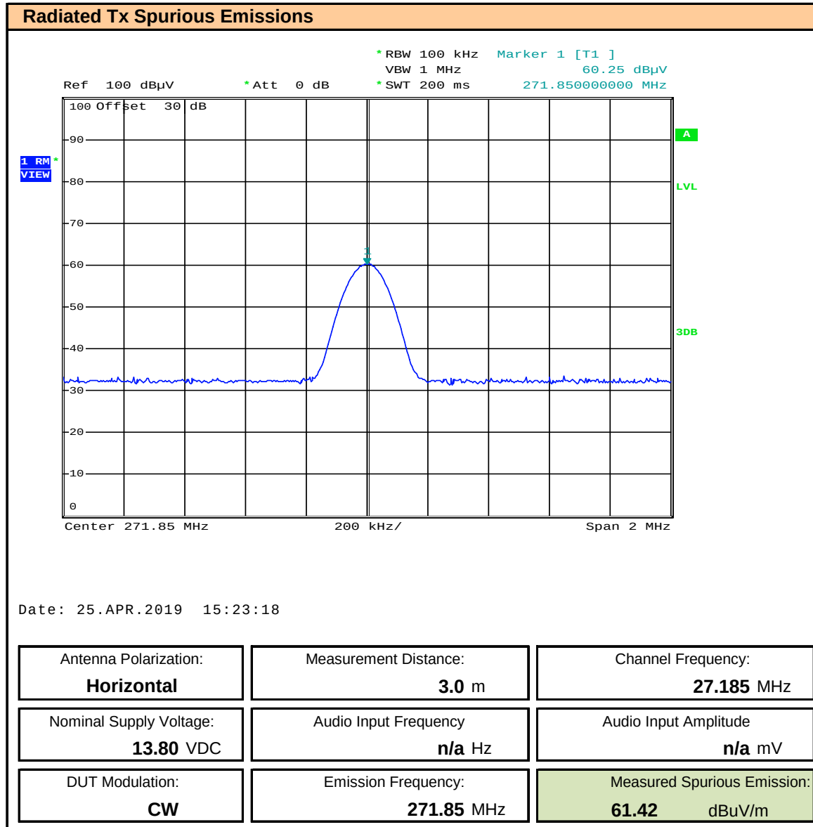
Plot 11.11 – Radiated Spurious Emissions OATS, 10 th Harmonic, Horizontal
