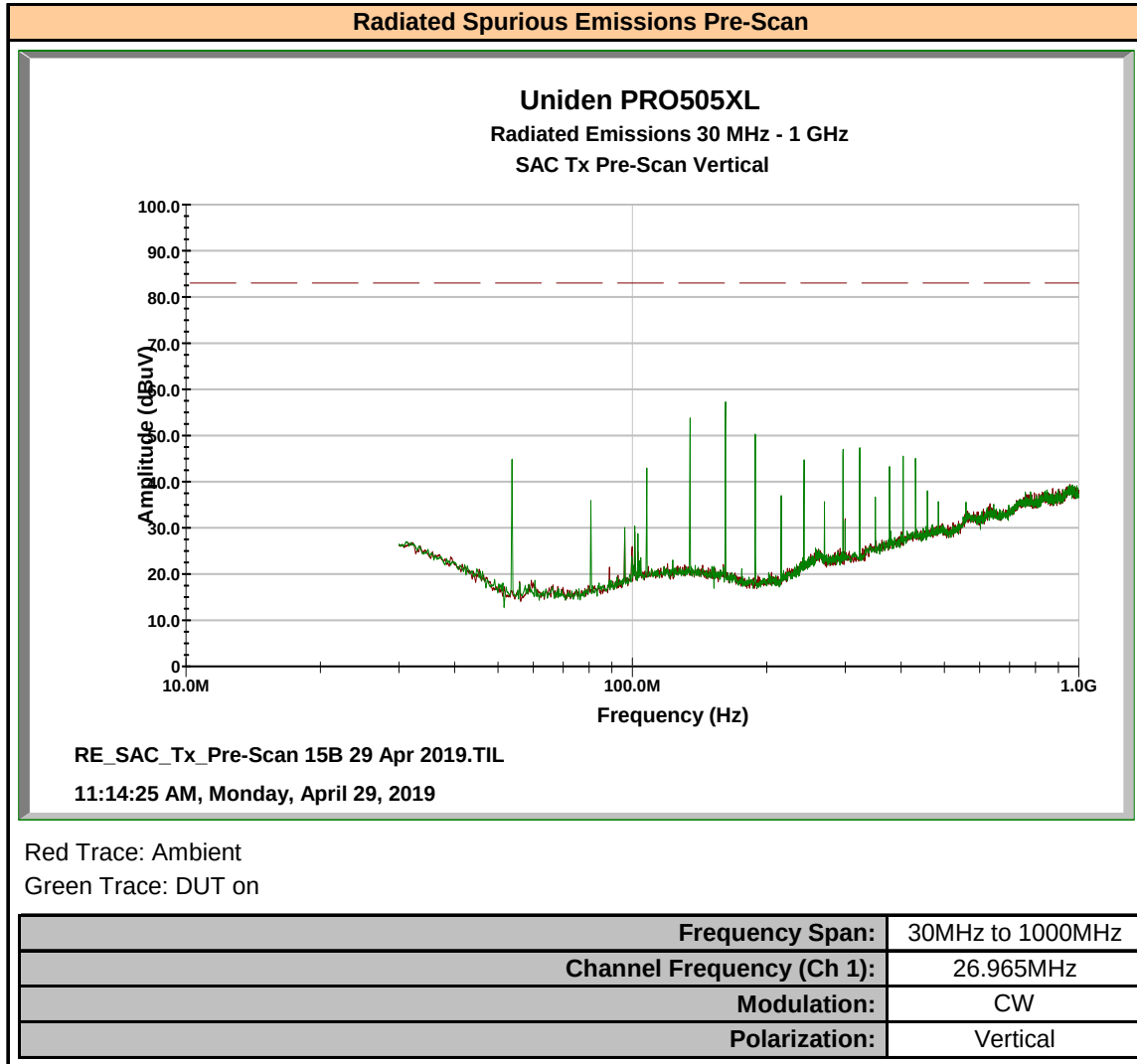
Plot 11.2 – Radiated Spurious Emissions Pre-Scan, 30MHz – 1000MHz, Vertical
