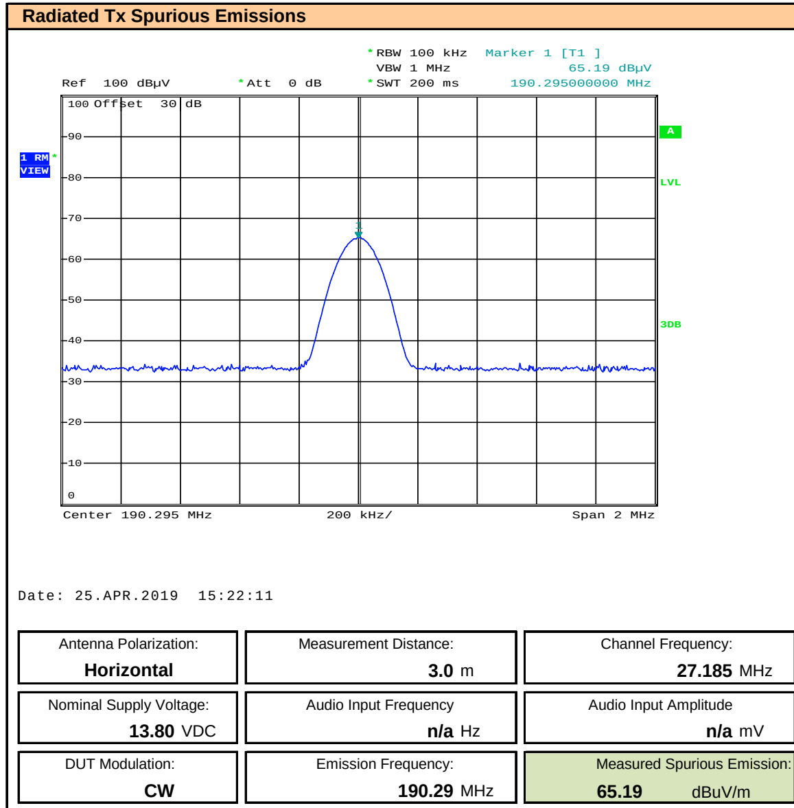
Plot 11.8 – Radiated Spurious Emissions OATS, 7 th Harmonic, Horizontal
