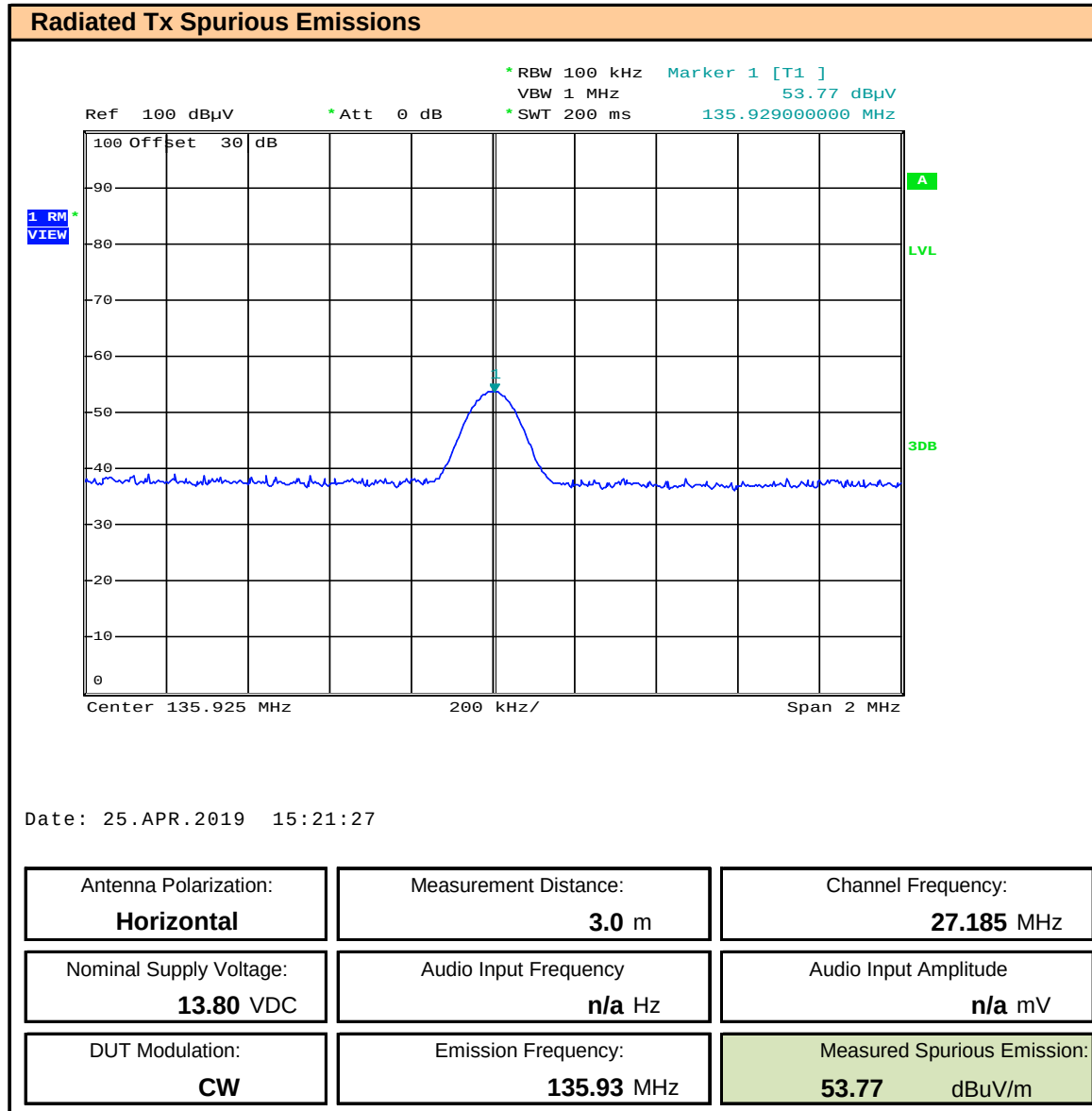
Plot 11.6 – Radiated Spurious Emissions OATS, 5 th Harmonic, Horizontal
