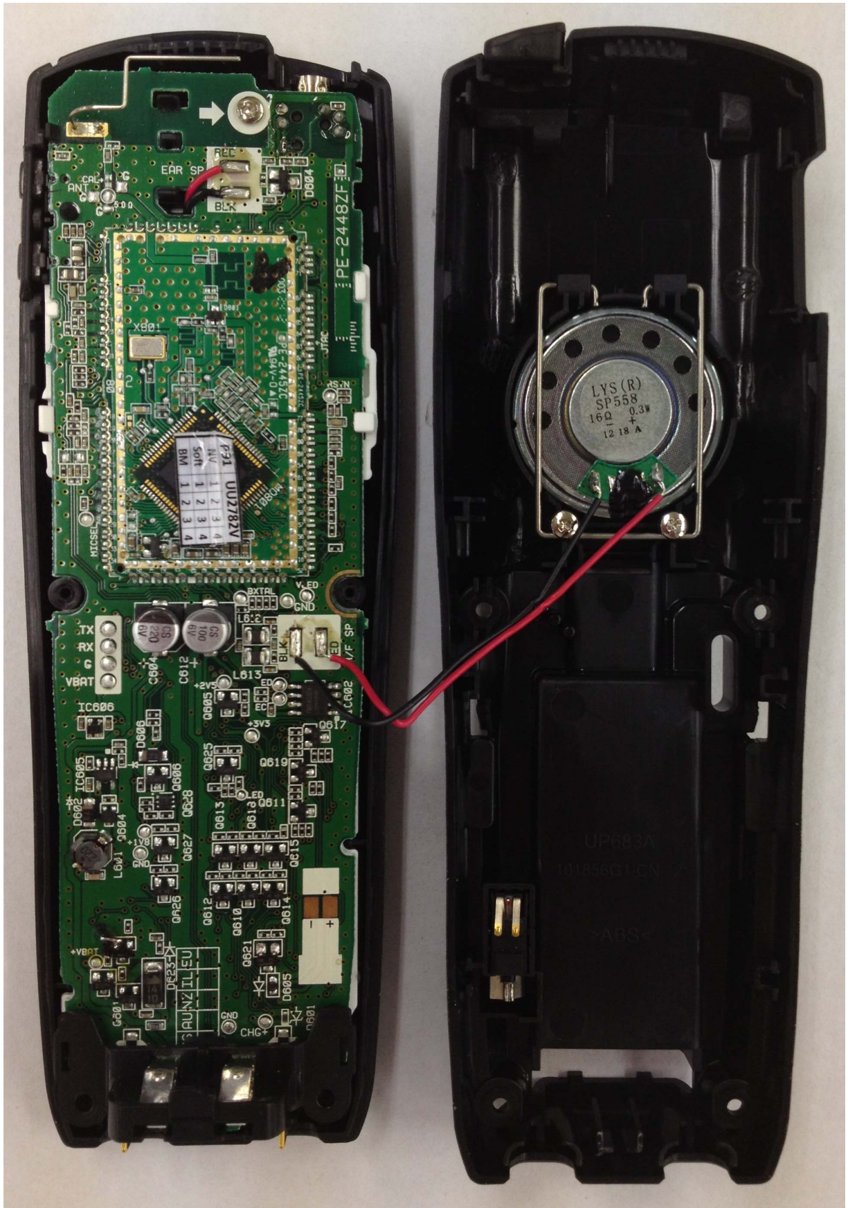
Rear Cover Opened ( " D100 DECT NA " Handset, " D160 DECT Handset NA " Extra Handset)
