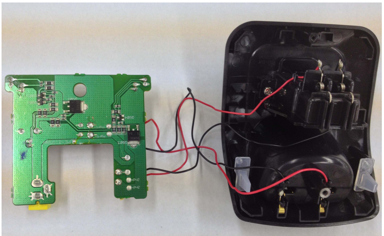
Main PCB Bottom View ( "D100 DECT NA" Charger, "D160 DECT Handset NA" Extra Charger)
