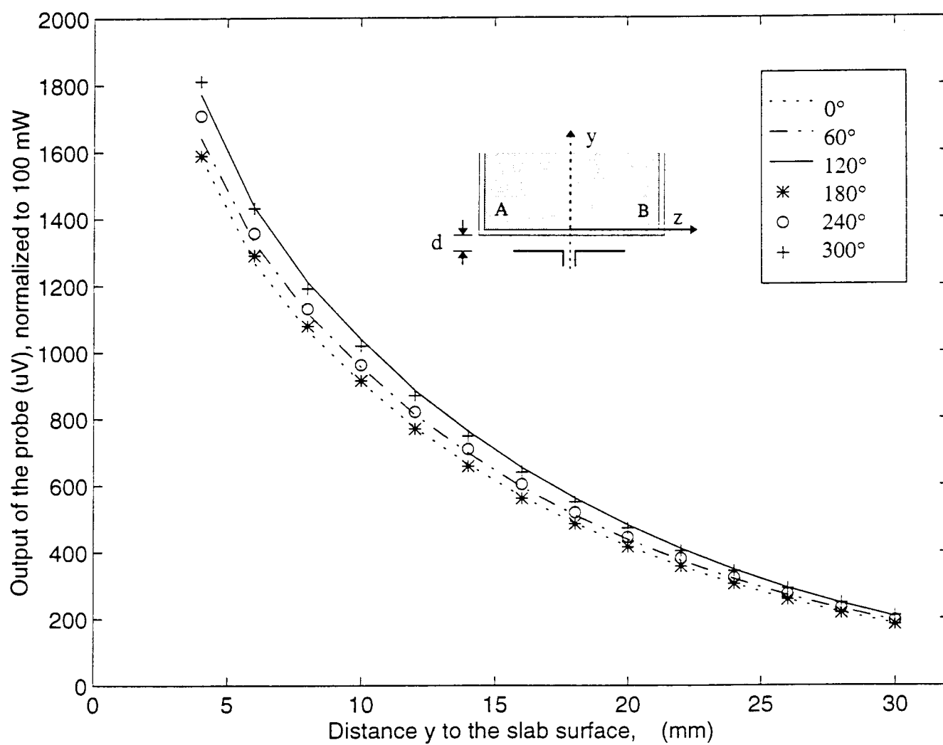
Figure 4b: Test for isotropy: The model shown in Figure 2 was used with nominal half wavelength dipole radiator of length 77 mm at 1900 MHz.
