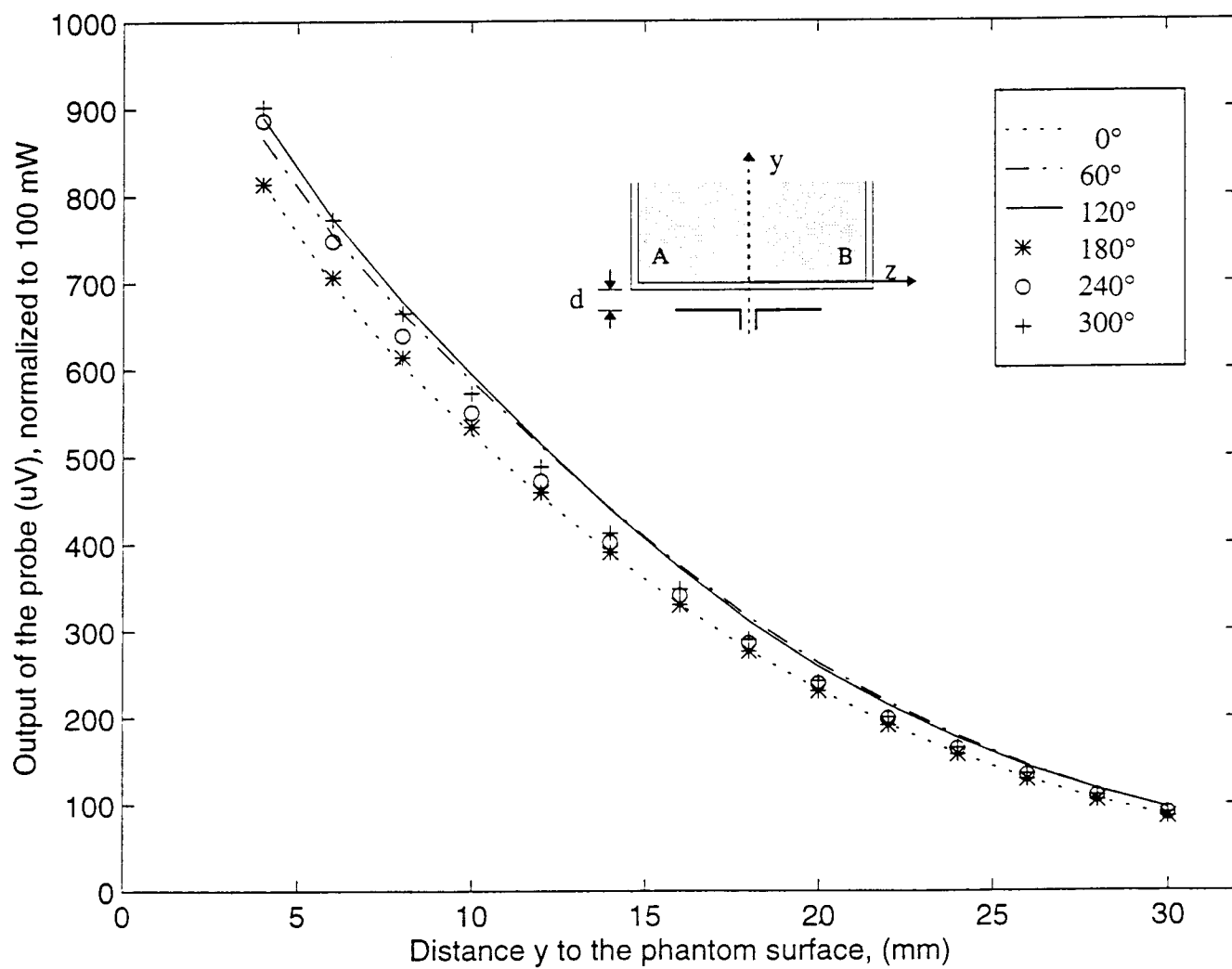
Figure 4a: Test for isotropy: The model shown in Figure 2 was used with nominal half wavelength dipole radiator of length 178 mm at 840 MHz.
