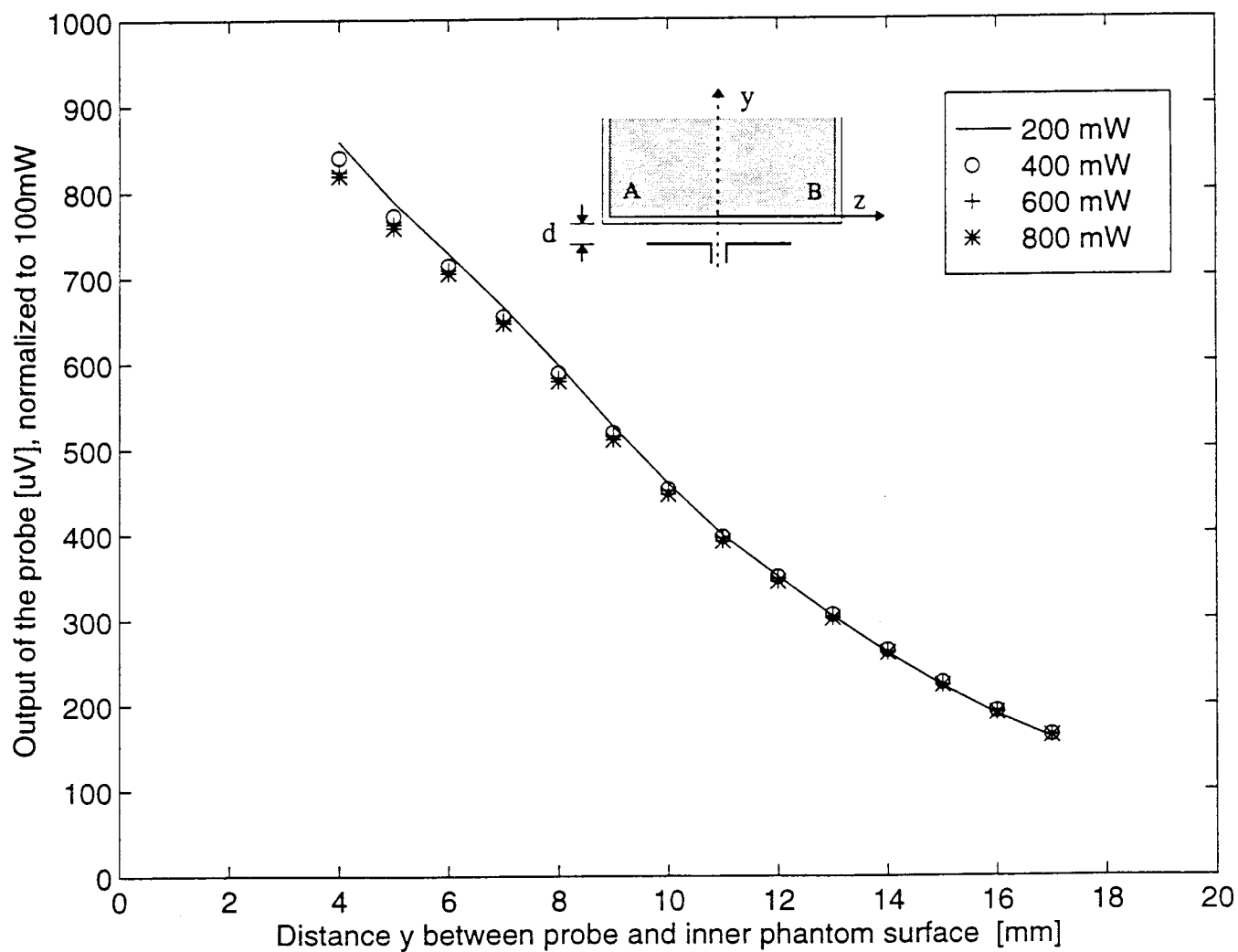
Figure 3b: Test for square-law behavior at 1900 MHz: Variation of the output voltage (proportional to |E_t|^2 ) for different radiated powers normalized to 0.1 W.
