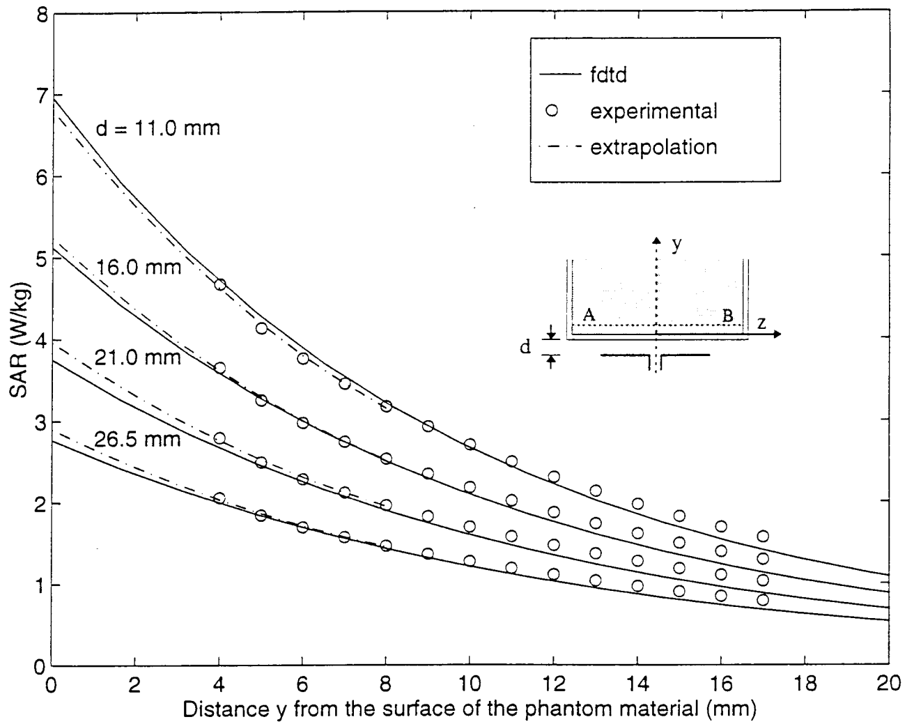
Figure 5a: Comparison of the calculated and measured SAR variations for a box phantom of dimensions 30 x 15 x 50 cm; 840 MHz; \lambda/2 dipole antenna; 0.5 W radiated power. Calibration factor for the Narda Model 8021 probe at 840 MHz = 0.49 (mW/kg)/ \mu V. Measured for the phantom material \epsilon_r = 41.1 , \sigma = 1.06 S/m.
