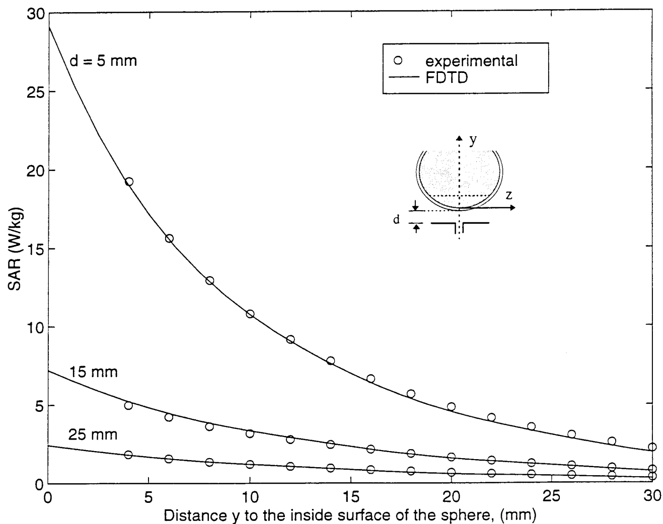
Figure 8a: Comparison of measured and FDTD-calculated SAR variations at 1900 MHz for a glass sphere model of outer diameter 22.3 cm and thickness 5 mm. SARs normalized to a radiated power of 0.5 W. Calibration factor = 0.84 (mW/kg)/ \mu V. Measured for the phantom material \epsilon_r = 45.5 , \sigma = 1.31 S/m.
