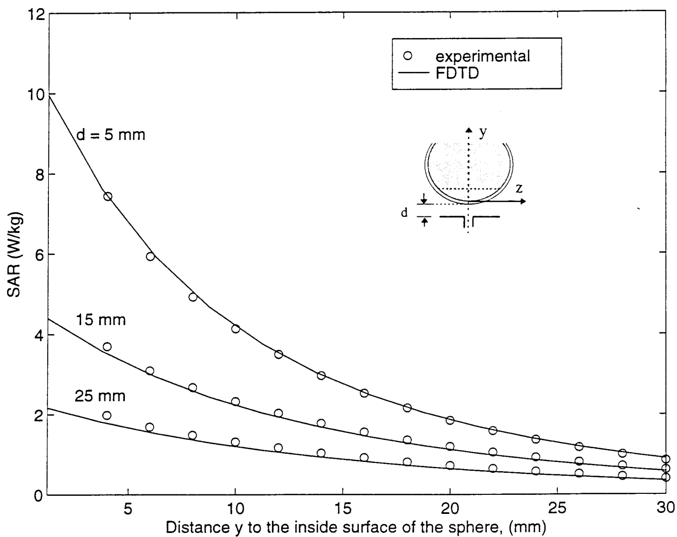
Figure 7a: Comparison of measured and FDTD-calculated SAR variations at 840 MHz for a glass sphere model of outer diameter 22.3 cm and thickness 5 mm. SARs normalized to a radiated power of 0.5 W. Calibration factor = 0.49 (mW/kg)/ \mu V. Measured for the phantom material \epsilon_r = 41.1 , \sigma = 1.06 S/m.
