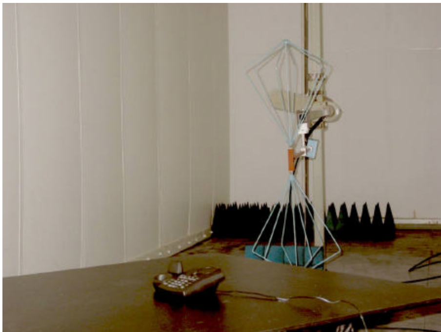
Uniden – Base Unit Testing for Radiated Emissions from Transmitter Frequency Range: 30 MHz – 200 MHz
