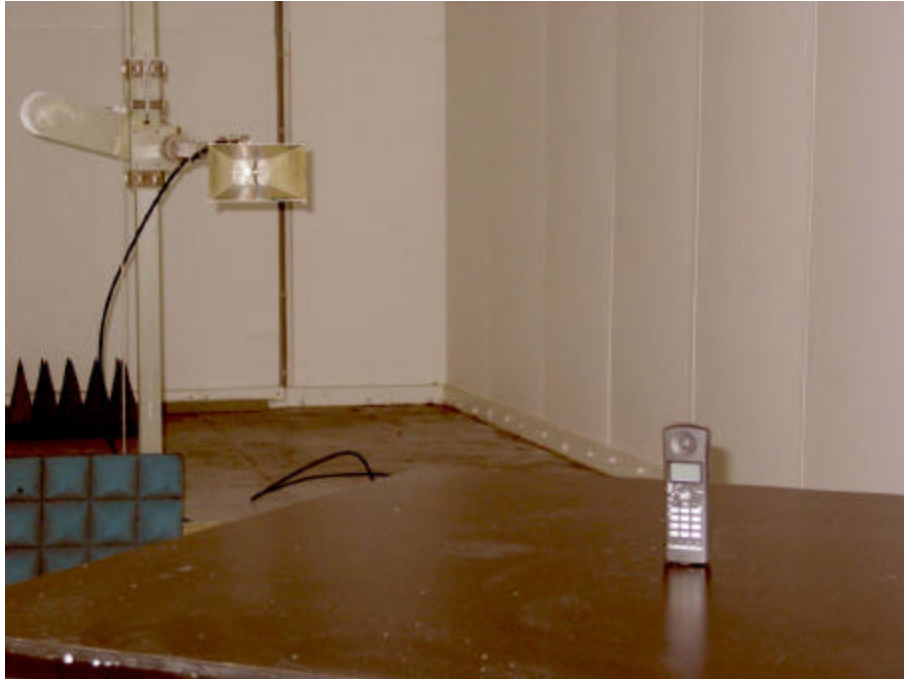
Uniden – Handset Testing for Radiated Emissions from Transmitter Frequency Range: 1 GHz – 18 GHz
