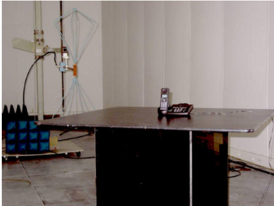
Uniden – Base & Handset Testing for Radiated Emissions from Transmitter Frequency Range: 30 MHz – 200 MHz
