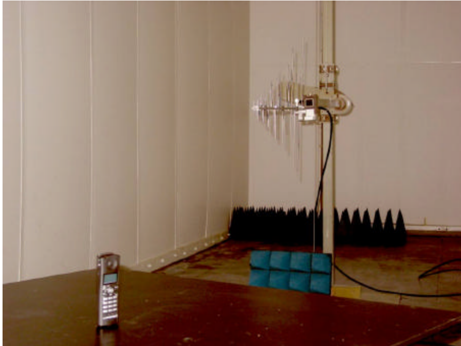
Uniden – Handset Testing for Radiated Emissions from Transmitter Frequency Range: 200 MHz – 1 GHz
