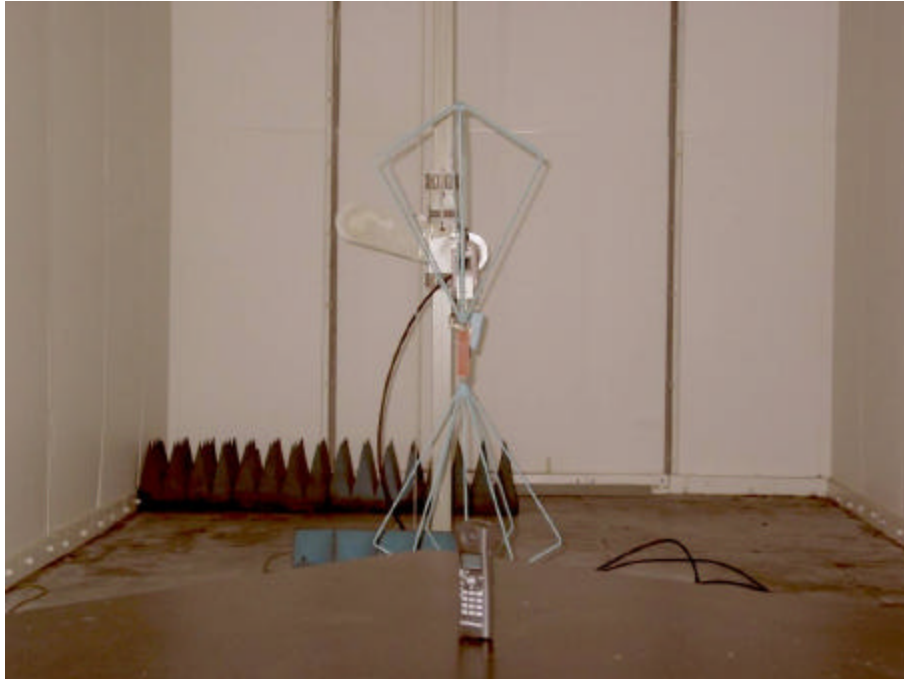
Uniden – Handset Testing for Radiated Emissions from Transmitter Frequency Range: 30 MHz – 200 MHz
