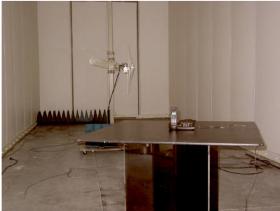
Uniden – Base & Handset Testing for Radiated Emissions from Transmitter Frequency Range: 200 MHz – 1 GHz
