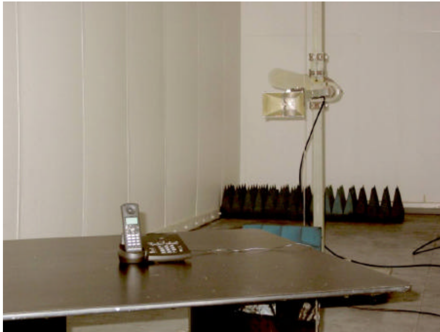
Uniden – Base & Handset Testing for Radiated Emissions from Transmitter Frequency Range: 1 GHz – 18 GHz
