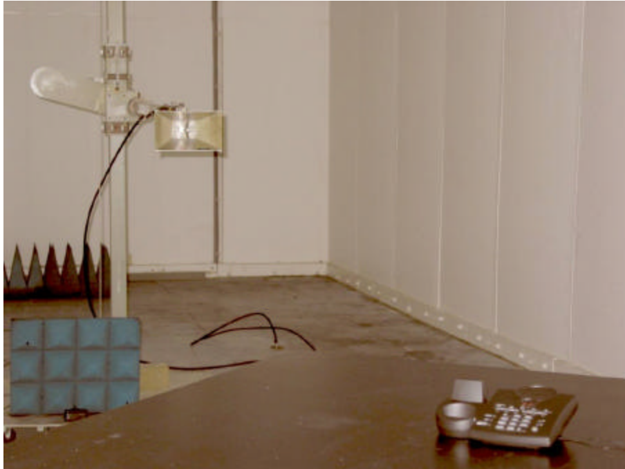
Uniden – Base Unit Testing for Radiated Emissions from Transmitter Frequency Range: 1 GHz – 18 GHz
