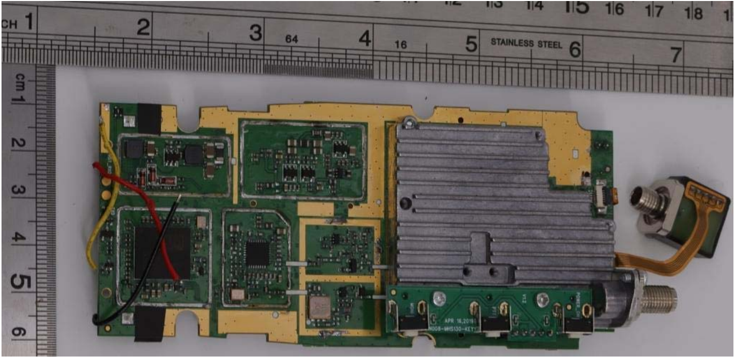
Figure E20.2 – Internal Photo – Covers Removed
