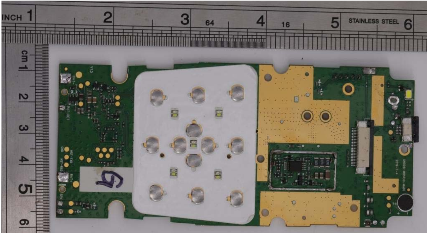
Figure E20.5 – Internal Photo – Display Removed
