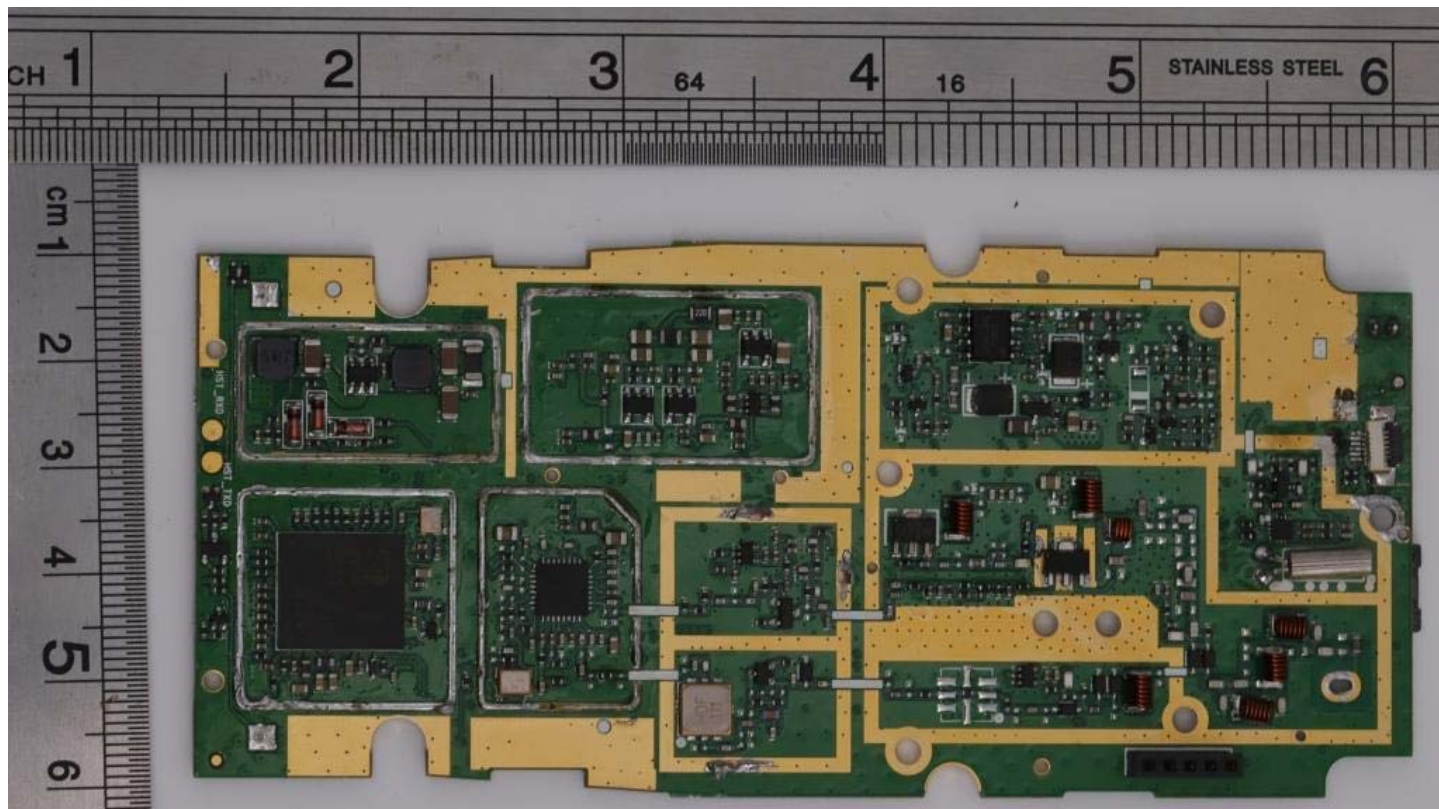
Figure E20.4 – Internal Photo – Heat Sink Removed
