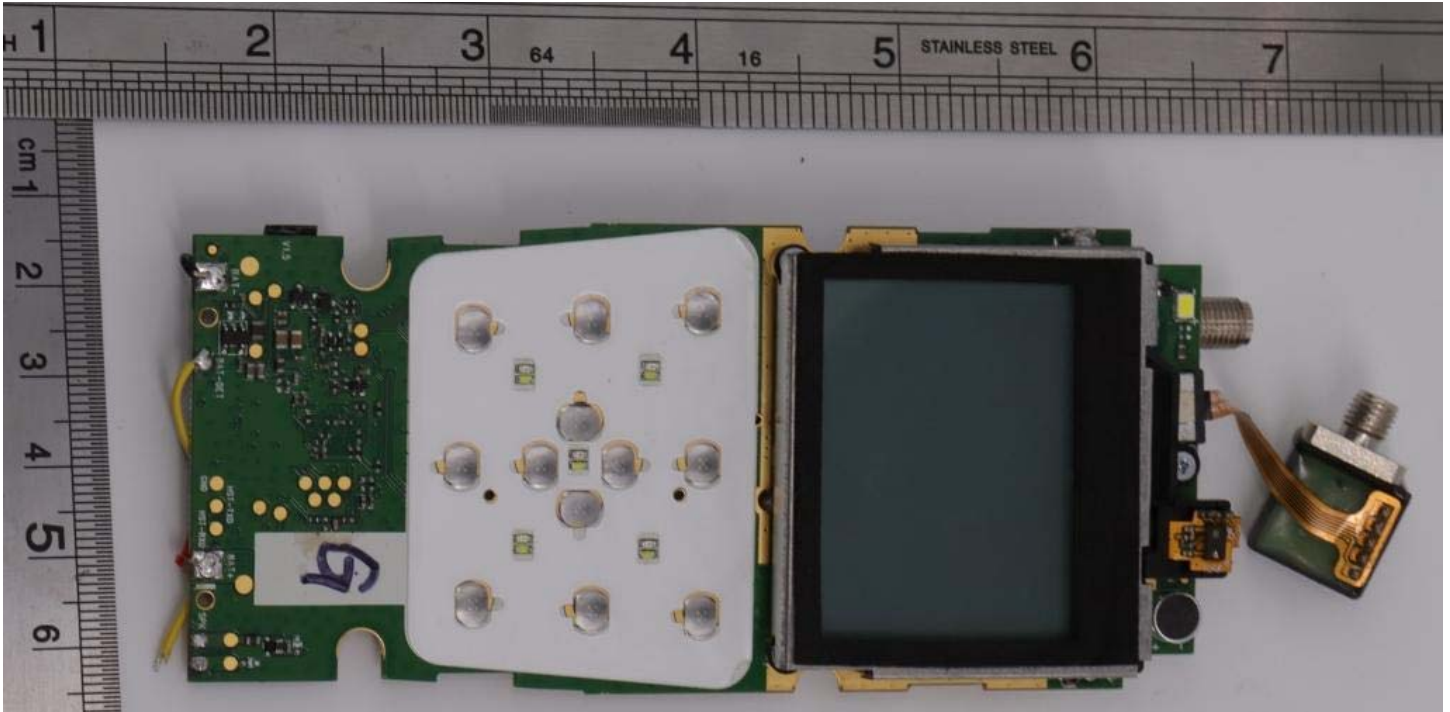
Figure E20.3 – Internal Photo – Keyboard/Display
