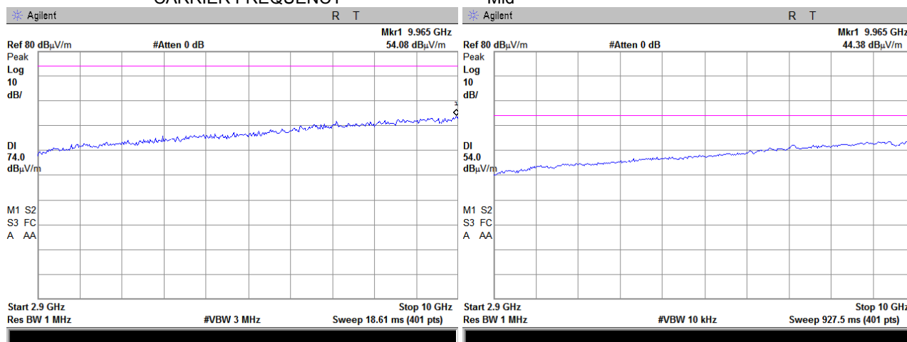
Plot 7.1.33 Radiated emission measurements from 2.9 to 10 GHz
