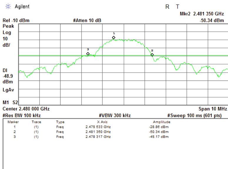
Plot 7.2.5 High band edge frequency
