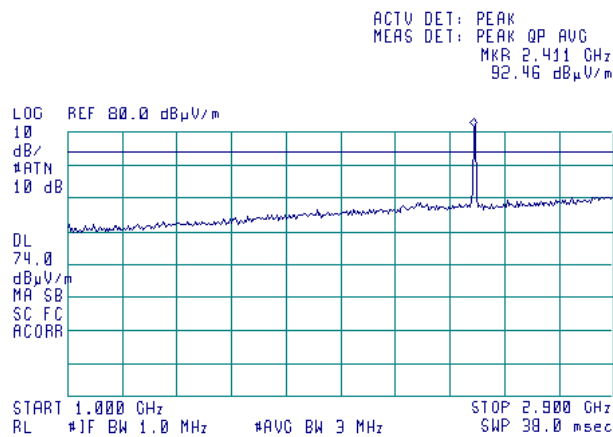
Plot 7.1.29 Radiated emission measurements from 1.0 to 2.9 GHz
