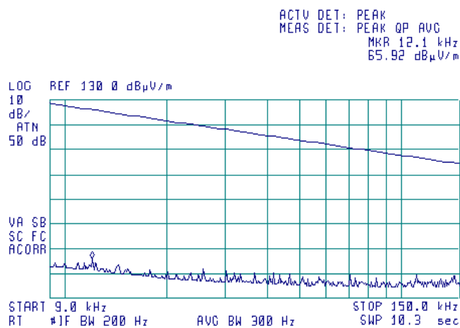
Plot 7.1.20 Radiated emission measurements from 9 to 150 kHz
